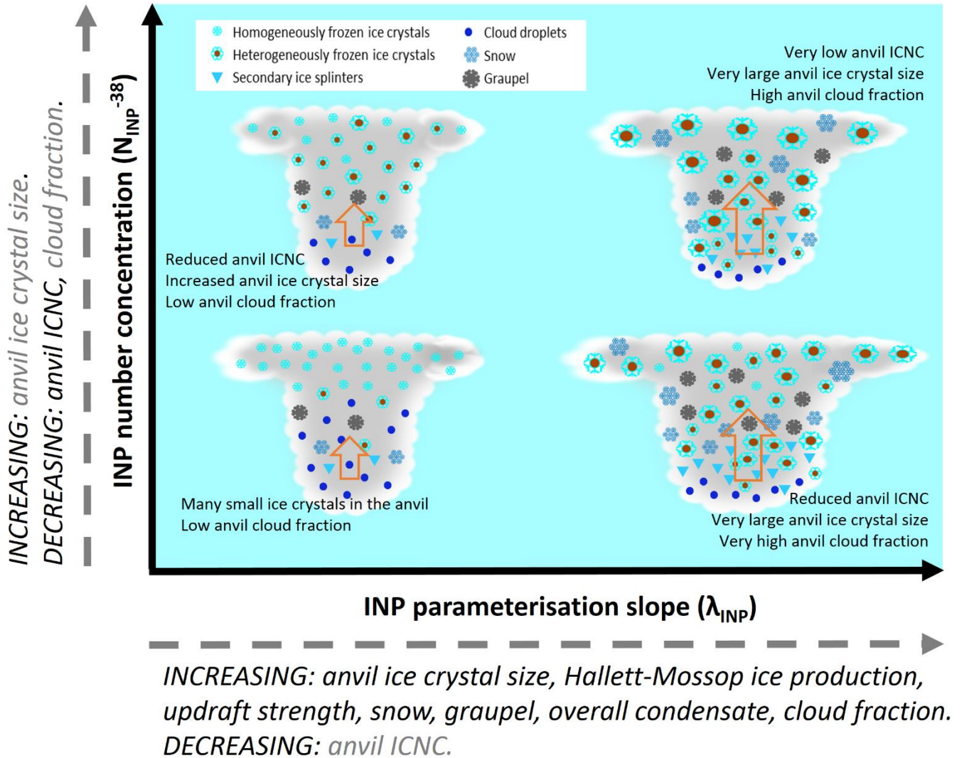
865 Figure 16. Schematic showing the key effects of the perturbations to absolute INP number concentration at -38\text{ }^{\circ}\text{C} ( N_{\text{INP}}^{-38} ) and INP parameterisation slope ( \lambda_{\text{INP}} ) on the deep convective cloud simulated in this study. Output variables written along the x- and y-axes in black indicate that they are primarily controlled by the uncertain input variable on that axes while grey writing indicates a secondary or smaller effect of the uncertain input variable in question.
