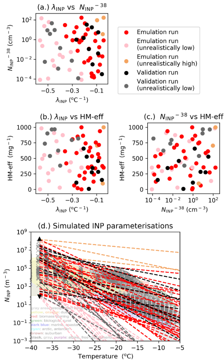
375 Figure 5. Experiment design. Values of the uncertain input parameter combinations used in the cloud model for the three uncertain input parameters ( N_{\text{INP}}^{-38} and \lambda_{\text{INP}} (a), \lambda_{\text{INP}} and HM-eff (b), and N_{\text{INP}}^{-38} and HM-eff (c)). Shown in (d) is the resultant INP parameterisations arising due to the combination of perturbations to \lambda_{\text{INP}} and N_{\text{INP}}^{-38} overlain on Fig. 1-10 of Kanji et al. (2017) (© American Meteorological Society. Used with permission). Output from the simulations shown in red, pink and orange are used to build the emulator while output from the simulations shown in black or grey are used to validate the emulator results. The distinction 380 between realistic (red, black) and unrealistic (pink, orange, grey) simulation perturbations is based on whether the corresponding parameterisation shown in (d) lies within the range of observations from Fig 1-10 of Kanji et al. (2017).
