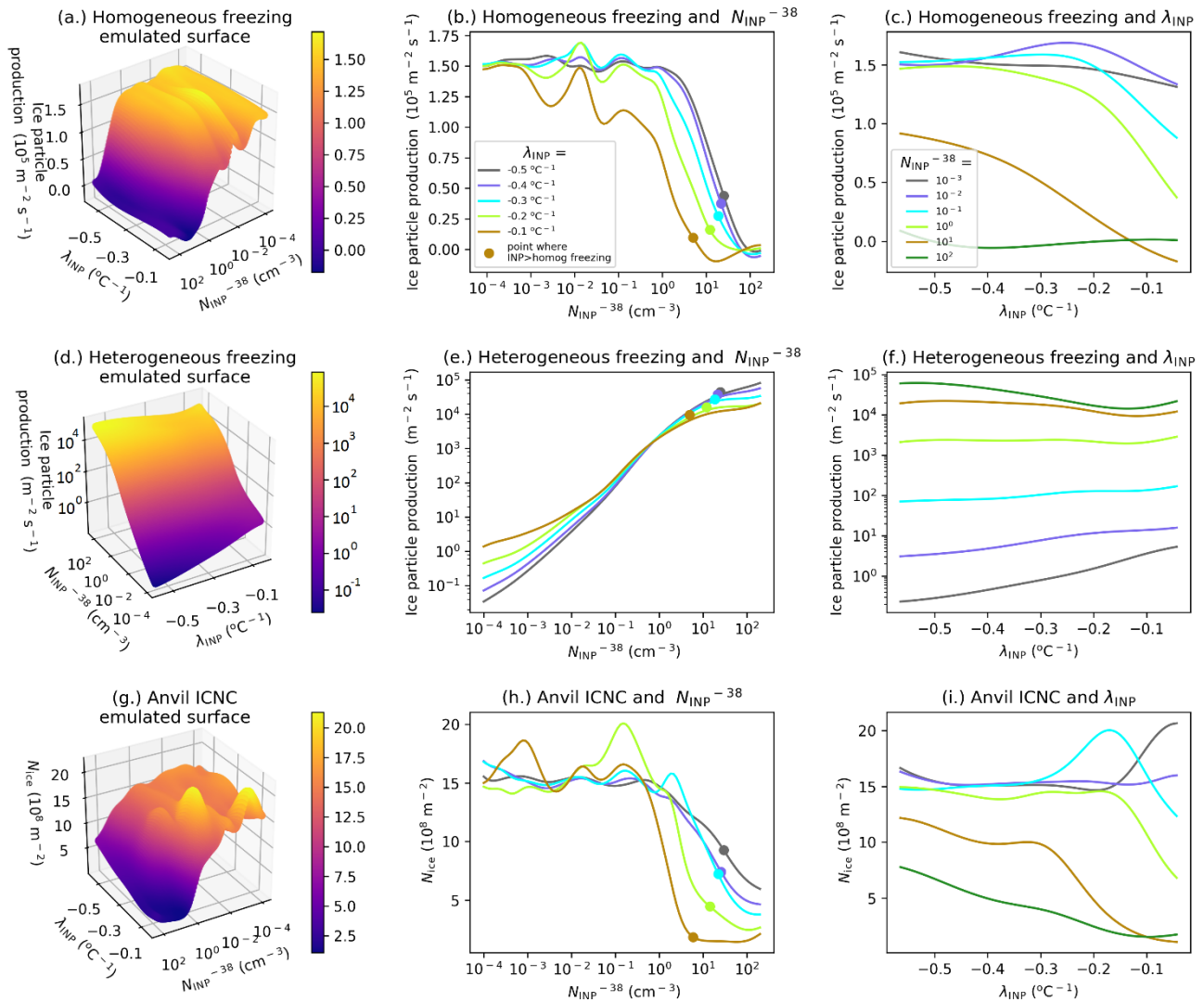
500 Figure 8. Emulator response surfaces. Prediction of ice particle production by homogeneous freezing (a, b, c), heterogeneous freezing (d, e, f), and anvil ICNC (g, h, i) by the emulator. Shown in (a), (d), and (g) are emulated response surfaces at a fixed HM-eff of 350 splinters \text{mg}^{-1} rimed. The colours indicate output values and are the same range and units as the z-axis. The line plots show the variation in predicted output value (y-axis) from these response surfaces for fixed \lambda_{\text{INP}} (b, e, h) and fixed N_{\text{INP}}^{-38} (c, f, i). Panels a-f are the average of the cloud property between 60 and 180 minutes (convective stage) of the simulation, while panels g-i are the 505 average of the relevant cloud property between 150 and 240 minutes (anvil stage) of the simulation.
