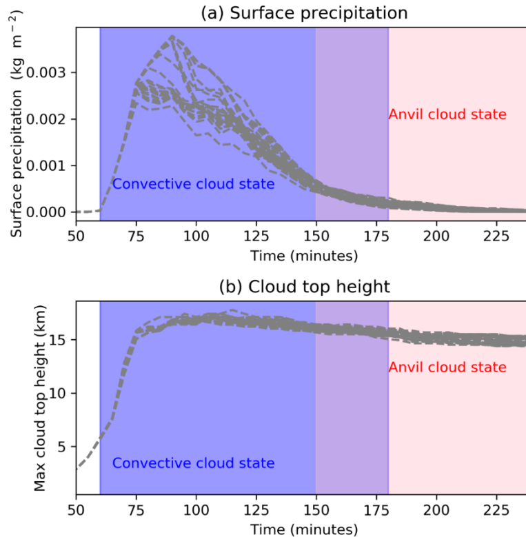
220 Figure 3. Simulated cloud properties. Evolution of surface precipitation in all cloudy regions (a) and maximum cloud top height (b) over time for all simulations included in analysis. The convective and anvil cloud stages defined for the purposes of analysis are highlighted.
