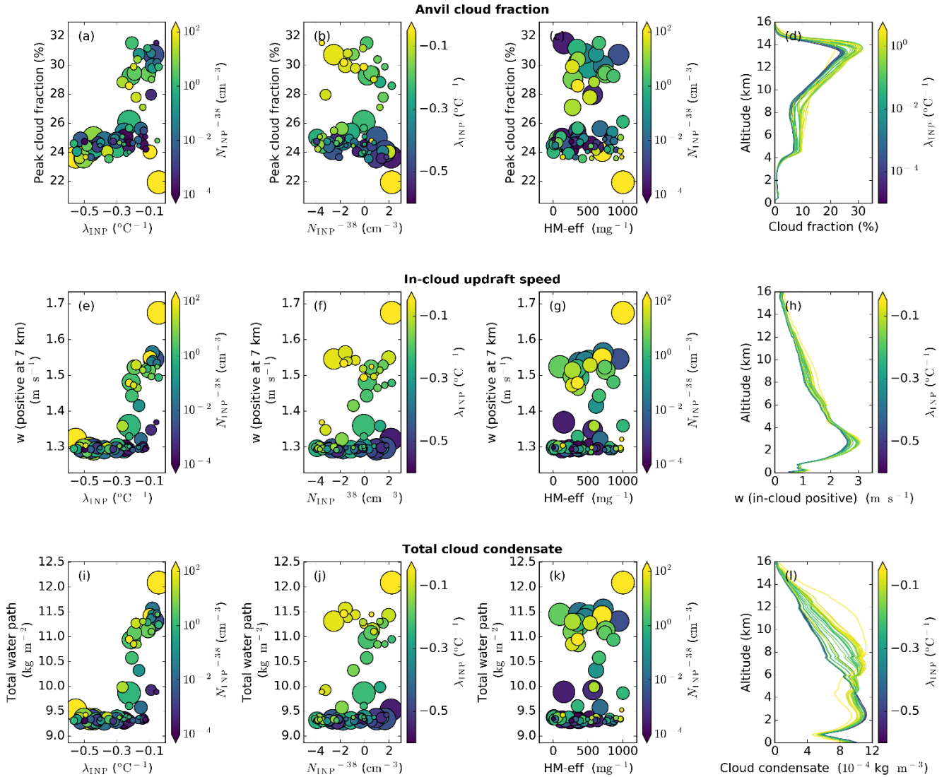
660 Figure 12. Anvil cloud fraction and driving processes. Dependence of anvil cloud fraction (a-d), in-cloud updraft speed at 7 km (e-h), and total cloud condensate (i-l) on the three uncertain input parameters: \lambda_{\text{INP}} (a, e, i), N_{\text{INP}}^{-38} (b, f, j), and HM-eff (c, g, k). In- 665 cloud profiles of anvil cloud fraction (d), in cloud updraft speed (h), and total cloud condensate (l) in all simulations are coloured by \lambda_{\text{INP}} . For panels (a), (e), and (i) the colour of the markers indicate N_{\text{INP}}^{-38} and the marker size indicates the HM-eff. For panels (b), (f), and (j) the colour of the markers indicate \lambda_{\text{INP}} and the marker size indicates HM-eff. For panels (c), (g), and (k) the colour of the markers indicate N_{\text{INP}}^{-38} and the marker size indicates \lambda_{\text{INP}} . Panels (a-d) are the average of the cloud property between 150 and 240 minutes (anvil stage) in the simulation, while panels (e-l) are the average of the relevant cloud property between 60 and 180 minutes (convective stage) in the simulations.
