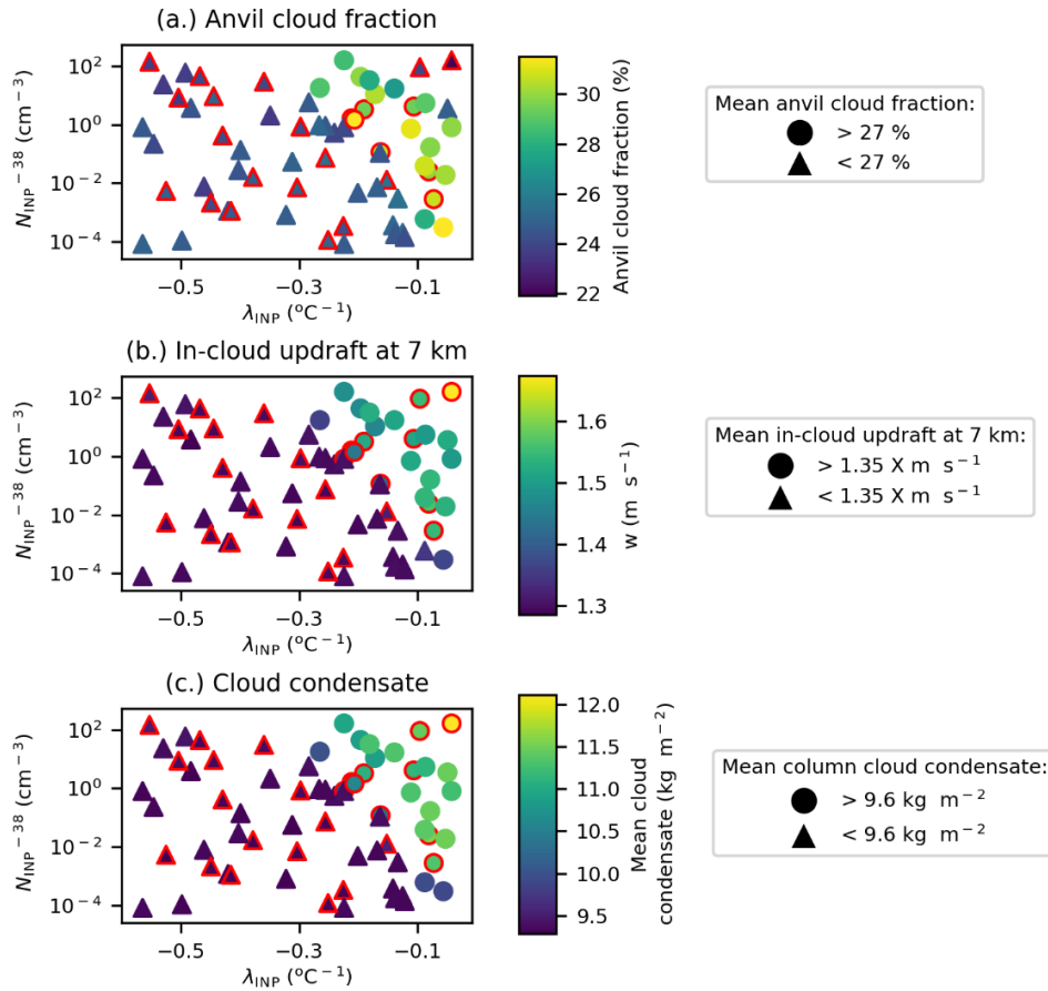
Figure 13. Regime change in anvil cloud fraction and driving processes. Variation in anvil cloud fraction (a), in-cloud updraft speed at 7 km (b), and total cloud water path (c) due to variation in \lambda_{\text{INP}} and N_{\text{INP}}^{-38} . Marker colours indicate the value of the mean peak anvil cloud fraction (a), in-cloud updraft speed at 7 km (b), and total cloud water path (c). Circular markers indicate a cloud fraction above 27% (a), a mean in-cloud updraft speed above 1.35 \text{ m s}^{-1} (b), and a water path over 9.6 \text{ kg m}^{-2} (c). Simulations with a HM-eff above 600 \text{ splinters mg}^{-1} are indicated with a red outline. Panel (a) is the average of the cloud property between 150 and 240 minutes (anvil stage) of the simulation, while panels (b) and (c) are the average of the relevant cloud property between 60 and 180 minutes (convective stage) of the simulation.
