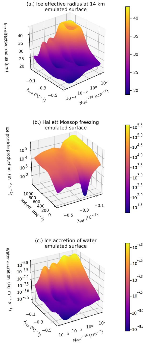
925 Figure A1. Emulator response surfaces. Prediction of ice effective radius (a), Hallett-Mossop ice particle production (b), and accretion of water by ice (c) by the emulator. Shown in (a) and (c) are the emulated response surfaces at a fixed HM-eff of 350 splinters mg -1 rimed. Shown in (b) is the emulated response surface at a fixed N_{\text{INP}}^{-38} of 1 cm -3 . The colours indicate output values and are the same range and units as the z-axis. Panel (a) is the average of the cloud property between 150 and 240 minutes (anvil stage) of the simulation, while panels (b) and (c) are the average of the relevant cloud property between 60 and 180 minutes 930 (convective stage) of the simulation.
