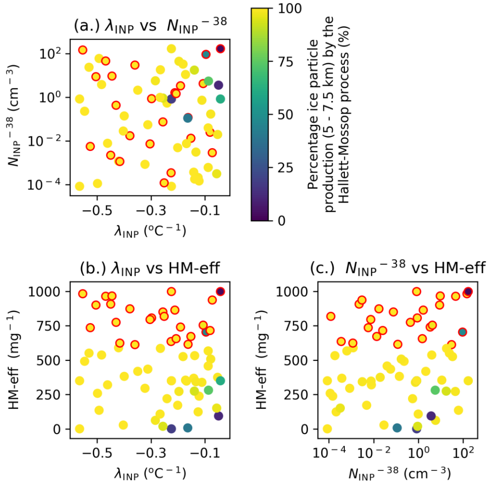
935 Figure A2. Source of ice crystals in the Hallett-Mossop region of the simulated deep convective cloud. Percentage of ice crystals produced between 5 and 7.5 km altitude that are produced from the Hallett-Mossop process [i.e. (Hallett-Mossop ice crystals / Hallett-Mossop and INP produced ice crystals) \times 100]. Simulations with a HM-eff above 600 splinters \text{mg}^{-1} are indicated with a red outline. Ice particle production rates are calculated from the convective stage of the simulation (between 60 and 180 minutes).
