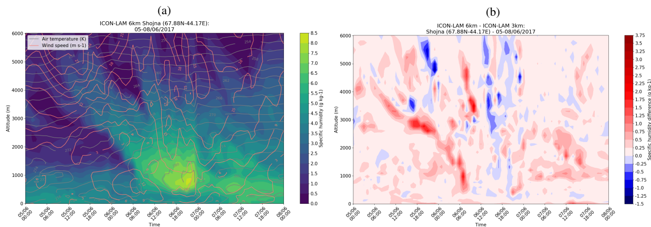
Figure 10. Time series of specific humidity in \text{g kg}^{-1} (color shading), air temperature in K (isolines) and wind speed in \text{m s}^{-1} (orange isolines) profiles at Shojna from ICON-LAM6 (a) and specific humidity difference between ICON-LAM6 and ICON-LAM3 (b, ICON-LAM3 remapped onto the ICON-LAM6 grid resolution), from 5 th June 2017 00:00 UTC to 8 th June 2017 00:00 UTC.
