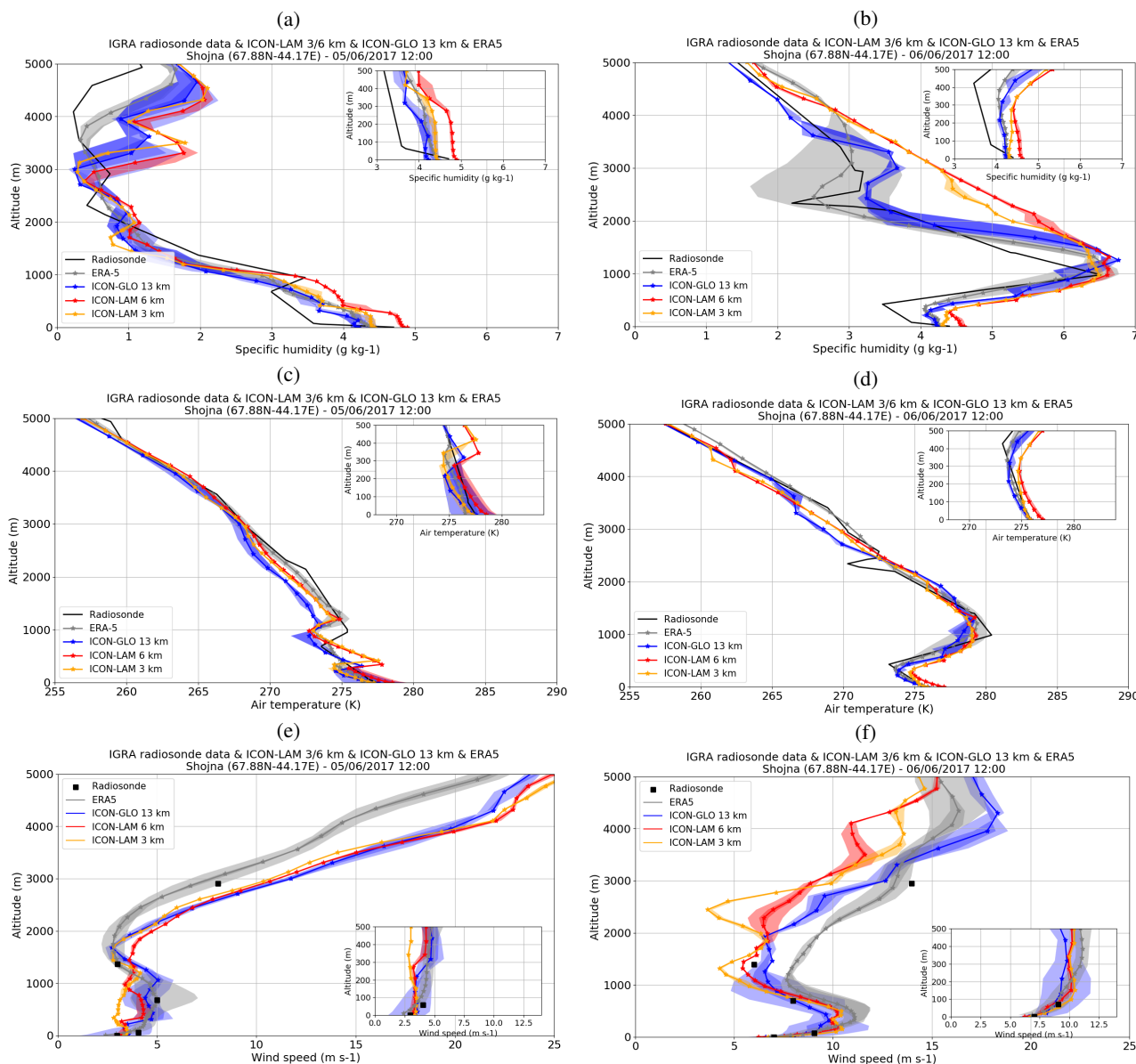
Figure 9. Vertical profiles of specific humidity in \text{g kg}^{-1} (a and b), air temperature in K (c and d) and wind speed in \text{m s}^{-1} (e and f) at Shojna from the IGRA radiosonde (black), ERA5 (grey) and ICON simulations (ICON-GLOBAL: blue, ICON-LAM6: red, ICON-LAM3: orange), on 5 th June 2017 12:00 UTC (a and c) and 6 th June 2017 12:00 UTC (b and d). For ERA5 and ICON simulations, the solid line presents the value at the Shojna nearest grid point, while the shading presents the range (maximum–minimum) across the four station surrounding grid points. A zoom of the profiles in the lowest 500 m is included in the upper right corner of each figure.
