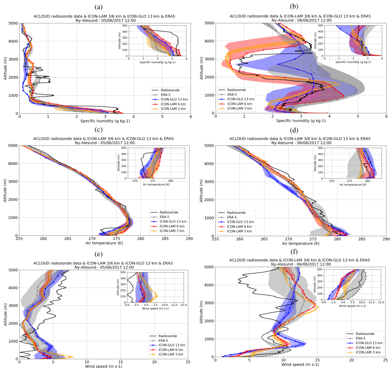
Figure 6. Vertical profiles of specific humidity in \text{g kg}^{-1} (a and b), air temperature in K (c and d) and wind speed in \text{m s}^{-1} (e and f) at Ny-Ålesund from the radiosonde data (black), ERA5 (grey), and ICON simulations (ICON-GLOBAL: blue, ICON-LAM6: red, ICON-LAM3: orange) on 5 th June 2017 12:00 UTC (a, c, e) and 6 th June 2017 12:00 UTC (b, d, f). For ERA5 and ICON simulations, the solid line presents the value for the Ny-Ålesund nearest grid point, while the shading presents the range (maximum-minimum) across the four station surrounding grid points. A zoom of the profiles in the lowest 500 m is included in the upper right corner of each figure.
