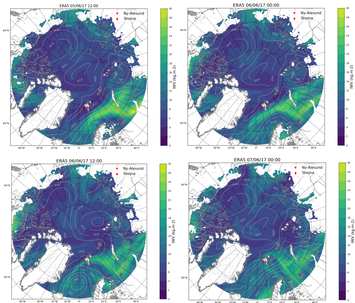
Figure A1. Pan Arctic ICON-LAM domain and representation of the integrated water vapour (IWV, \text{kg m}^{-2} , color shading) and mean sea level pressure (MSLP, hPa, white isolines) from ERA5 from 5 th June 2017 12:00 UTC to 7 th June 2017 00:00 UTC. The location of the Ny-Ålesund and Shojna research stations are included as red symbols.
