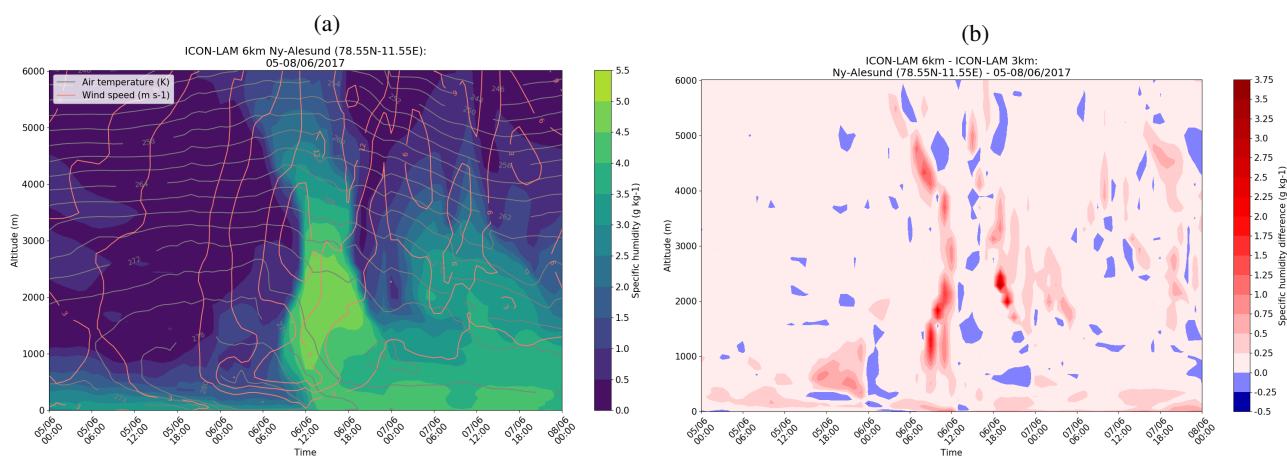
Figure 7. Time series of specific humidity ( \text{g kg}^{-1} , color shading), air temperature (K, grey isolines) and wind speed ( \text{m s}^{-1} , orange isolines) profiles at Ny-Ålesund from ICON-LAM6 (a) and specific humidity difference between ICON-LAM6 and ICON-LAM3 (b, ICON-LAM3 was remapped onto the ICON-LAM6 grid resolution), from 5 th June 2017 00:00 UTC to 8 th June 2017 00:00 UTC.
