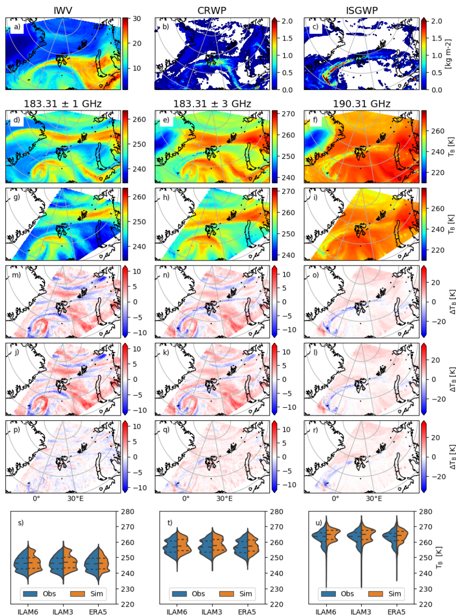
Figure 3. Top row shows the integrated contents of water vapour (IWV, a)) and liquid (CRWP, b)) and solid hydrometeor content (ISGWP, c)) from the 6 km ICON-LAM simulation for the 6 th June 2017 12:00 UTC. In panels d-f) the forward simulated T_B at 183.31 \pm 1 , 183.31 \pm 3 , and 190.31 GHz based on ICON-LAM on the 6km resolution are shown. g) to i) show the observations from MHS for an overpass between 11:00 and 13:00 UTC. The differences between simulation and observation for 6 and 3 km ICON LAM simulations and ERA5 reanalysis (rows) are shown in m) to r). Bottom panels s)-u) present, through kernel density plots the observations to each corresponding simulation.
