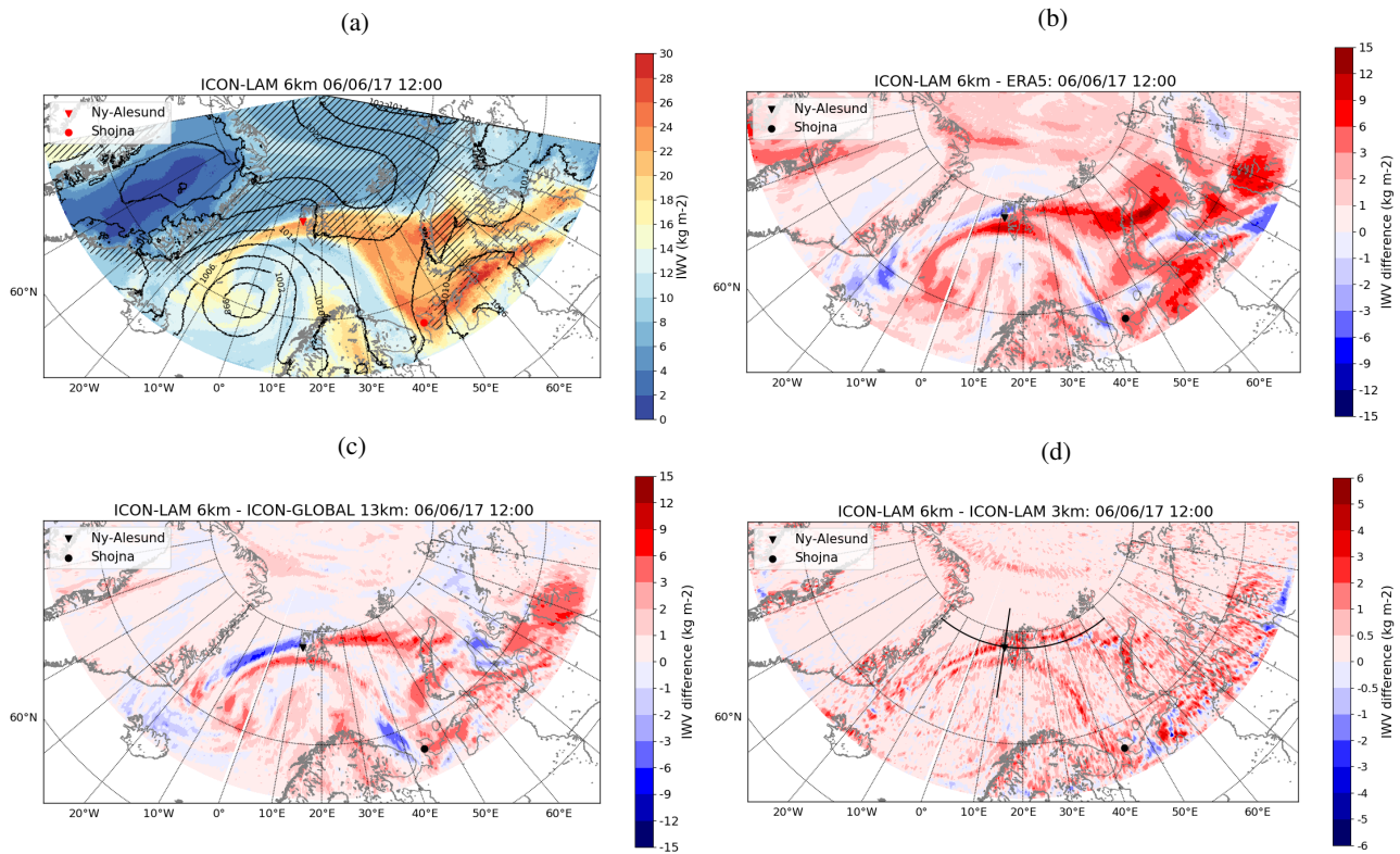
Figure 2. (a): Integrated water vapour (IWV, \text{kg m}^{-2} , color shading), mean sea level pressure (MSLP, hPa, black isolines), precipitation (pink isolines for precipitation > 5 \text{ mm} ) and sea-ice (black hatches for sea-ice fraction > 0.15 ) from ICON-LAM 6 km. (b), (c), (d): Differences of IWV between ICON-LAM 6 km and ERA5 (ICON-LAM6 - ERA5, b), ICON-GLOBAL 13 km (ICON-LAM6 - ICON-GLOBAL, c) and ICON-LAM 3 km (ICON-LAM6 - ICON-LAM3, d, note the different scale) on 6 th June 2017 12:00 UTC. All IWV fields have been remapped onto the ERA5 (0.25x0.25 regular lat-lon) grid to calculate the differences. The black lines (d) are the reference lines for the presented cross sections in Fig. 4. The locations of the Ny-Ålesund and Shojna research stations are also shown.
