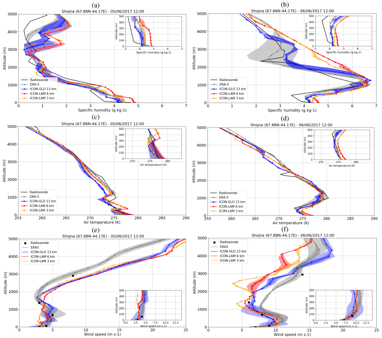
Figure 9. Vertical profiles of specific humidity ( \text{in } \text{g kg}^{-1} ; (a and b), air temperature \text{in } \text{K} (K; c and d) and wind speed \text{in } \text{m s}^{-1} ( \text{m s}^{-1} ; e and f) at Shojna from the IGRA radiosonde (black), ERA5 (grey) and ICON simulations (ICON-GLOBAL: blue, ICON-LAM6: red, ICON-LAM3: orange), on 5 th June 2017 12:00 UTC (a and c) and 6 th June 2017 12:00 UTC (b and d). For ERA5 and ICON simulations, the solid line presents the value at the Shojna nearest grid point, while the shading presents the range (maximum-minimum) across the four station surrounding grid points. A zoom of the profiles in the lowest 500 m-m is included in the upper right corner of each figure.
