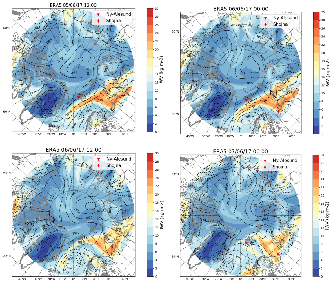
Figure A1. Pan Arctic ICON-LAM domain and representation of the integrated water vapour (IWV, kg m -2 , color shading) and mean sea level pressure (MSLP, hPa, white-black dotted isolines) from ERA5 from 5 th June 2017 12:00 UTC to 7 th June 2017 00:00-00 UTC . The location of the Ny-Ålesund and Shojna research stations are included as red symbols.
