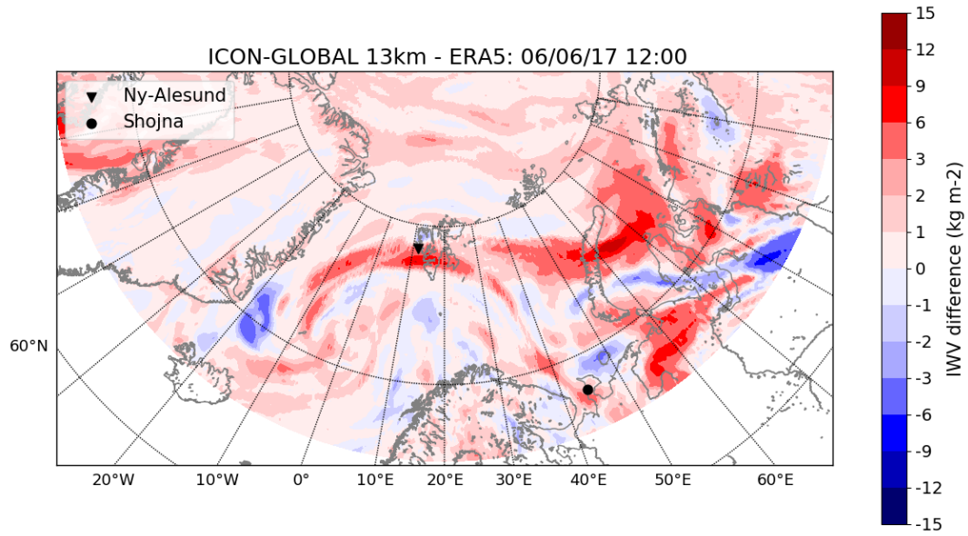
Figure B1. Differences of integrated water vapour (IWV, kg m -2 ) between ICON-GLOBAL 13 km and ERA5 on 6 th June 2017 12:00:00 UTC. The IWV field has been remapped onto the ERA5 (0.25x0.25 regular lat-lon) grid to calculate the difference.
