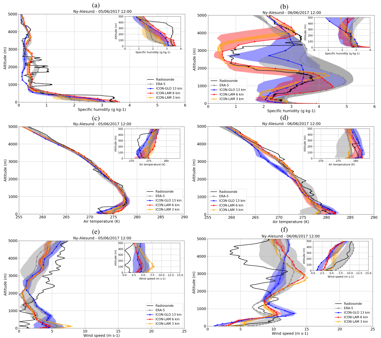
Figure 6. Vertical profiles of specific humidity ( \text{in g kg}^{-1} ; a and b), air temperature \text{in K} (K; c and d) and wind speed \text{in ms}^{-1} ( \text{m s}^{-1} ; e and f) at Ny-Ålesund from the radiosonde data (black), ERA5 (grey), and ICON simulations (ICON-GLOBAL: blue, ICON-LAM6: red, ICON-LAM3: orange) on 5 th June 2017 12:00 UTC (a, c, e) and 6 th June 2017 12:00 UTC (b, d, f). For ERA5 and ICON simulations, the solid line presents the value for the Ny-Ålesund nearest grid point, while the shading presents the range (maximum-minimum) across the four station surrounding grid points. A zoom of the profiles in the lowest 500 m is included in the upper right corner of each figure.
