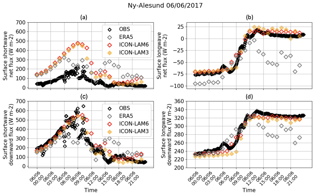
Figure 11. Time series of the surface shortwave net flux (a), surface longwave net flux (b), surface shortwave downward flux (c) and surface longwave downward flux (d) ( \text{W m}^{-2} ) from ERA5, ICON-LAM6, ICON-LAM3 and from observations at Ny-Ålesund on 6 th June 2017. The fluxes are positive downward.
