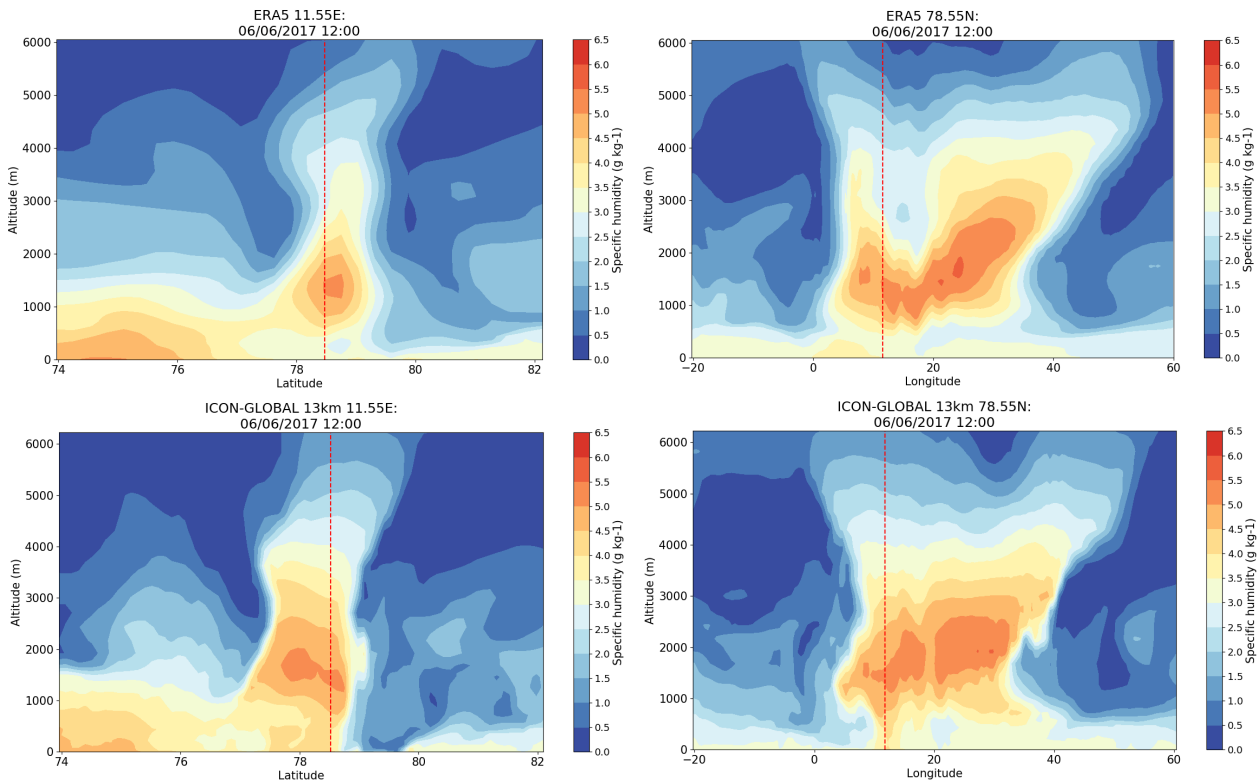
Figure C1. Altitude-latitude/longitude cross-sections of specific humidity ( \text{g kg}^{-1} , color shading) and wind speed ( \text{m s}^{-1} , grey isolines) from ERA5 (top panels) and ICON-GLOBAL (bottom panels), along latitude at 11.55^\circ\text{E} (left panels) and along longitude at 78.55^\circ\text{N} (right panels) on 6 th June 2017 12:00–00 UTC. Black and red dotted lines: Ny-Ålesund location. The location of the cross-sections is indicated in Fig. 2.2d.
