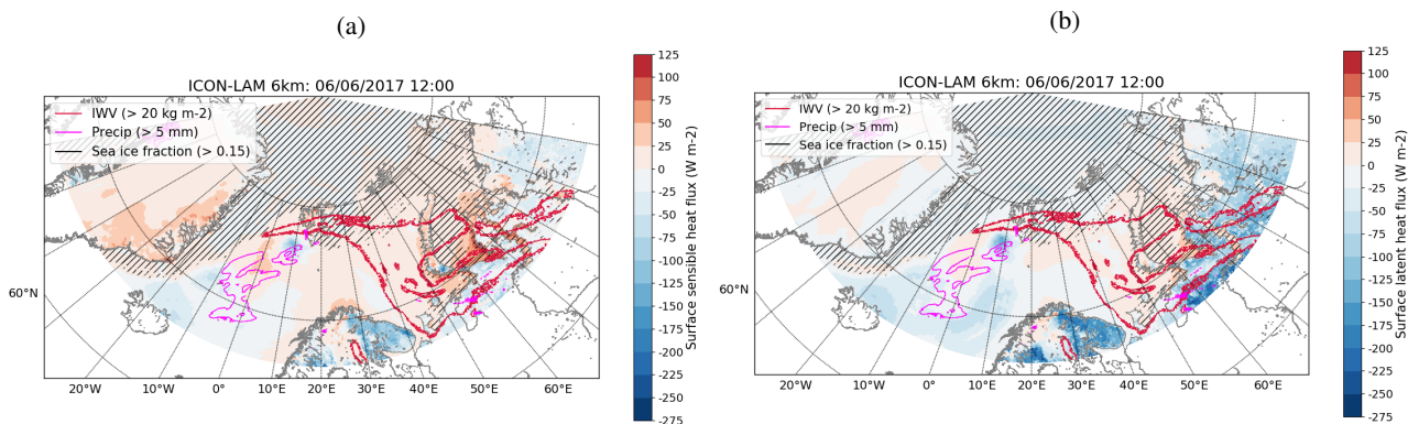
Figure 12. Surface map of sensible (a) and latent (b) heat fluxes ( \text{W m}^{-2} , color shading) from ICON-LAM 6 km, on 6 th June 2017 12:00-00 UTC. Positive/negative signs indicate a downward/upward flux to/from the surface. Regions of IWV > 20 \text{kg m}^{-2} (red line), precipitation > 5 \text{mm} (pink line) and sea-ice fraction > 0.15 (black hatching) are included.
