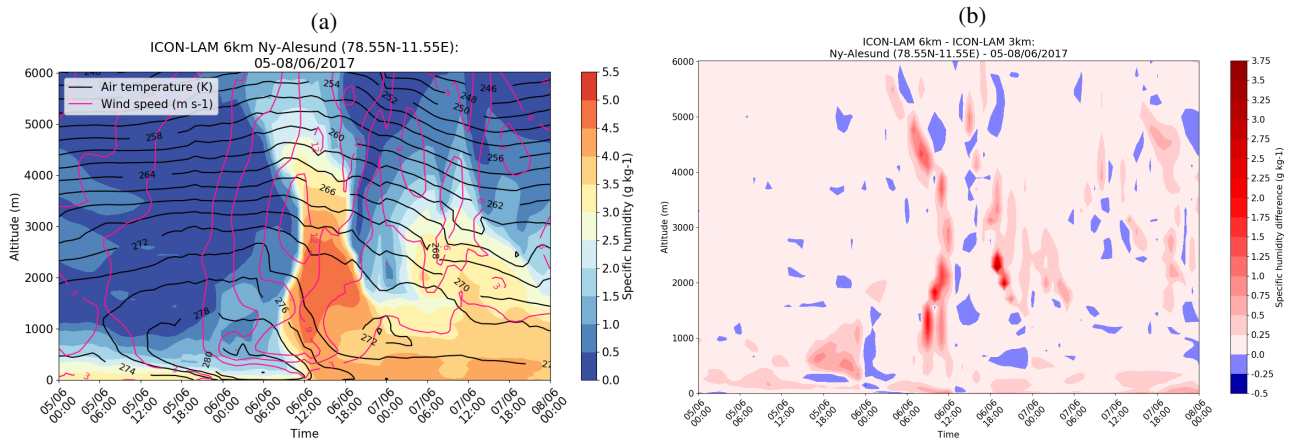
Figure 7. Time series of specific humidity ( \text{g kg}^{-1} , color shading), air temperature (K, grey-black isolines) and wind speed ( \text{m s}^{-1} , orange-magenta isolines) profiles at Ny-Ålesund from ICON-LAM6 (a) and specific humidity difference between ICON-LAM6 and ICON-LAM3 (b, ICON-LAM3 was remapped onto the ICON-LAM6 grid resolution ), from 5 th June 2017 00:00 UTC to 8 th June 2017 00:00 UTC ( ICON-LAM3 was remapped onto the ICON-LAM6 grid resolution ).
