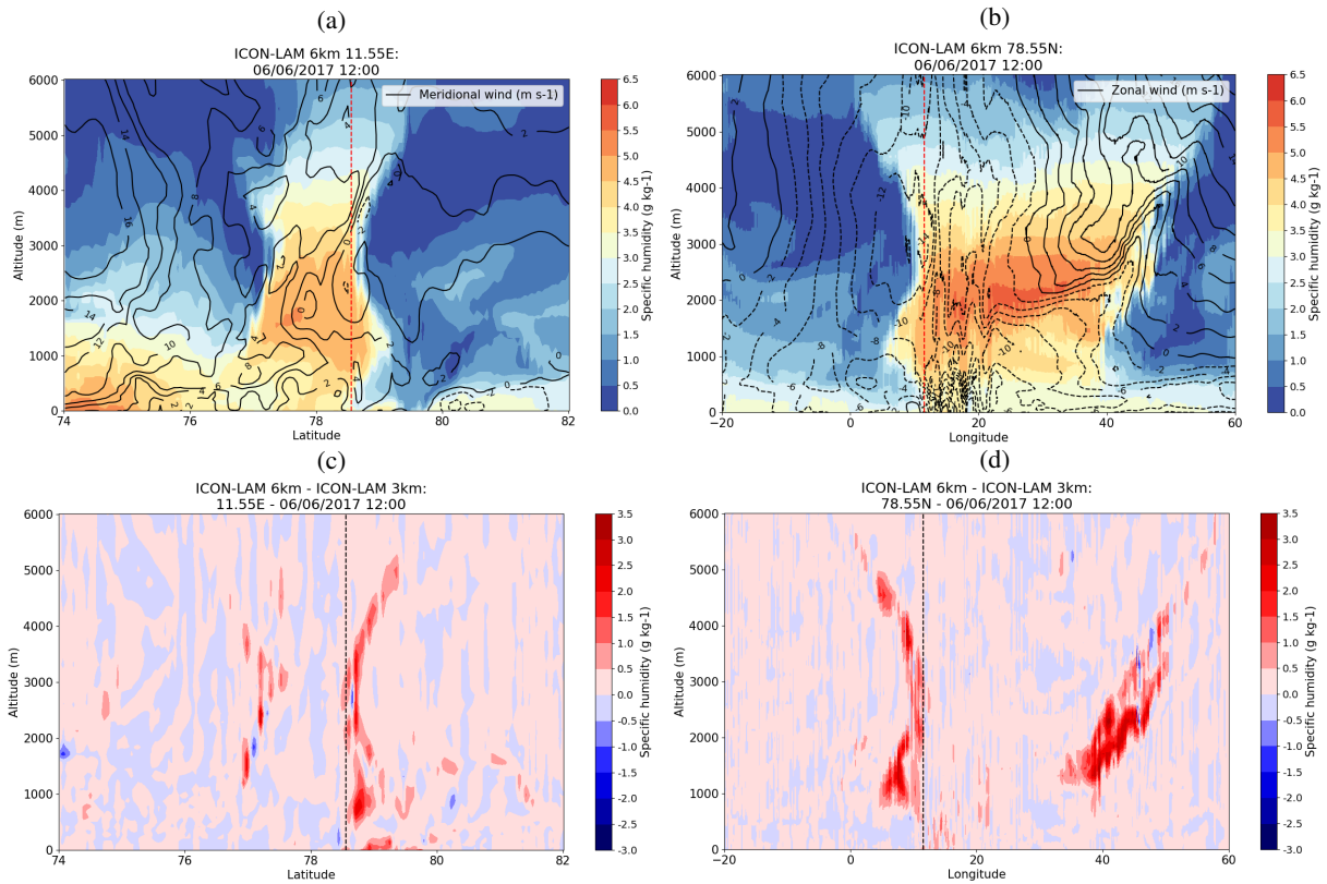
Figure 4. Altitude-latitude/longitude cross-sections of specific humidity ( \text{g kg}^{-1} , color shading) and wind speed ( \text{m s}^{-1} , grey isolines) from ICON-LAM6 (a, b) and of specific humidity difference between ICON-LAM6 and ICON-LAM3 (c, d), along latitude at 11.55^\circ\text{E} (a, c) and along longitude at 78.55^\circ\text{N} (b, d) on 6 th June 2017 12:00. Black and red dotted lines: column above Ny-Ålesund location. The location of the cross-sections is indicated in Fig. 2d. Altitude-latitude/longitude cross-sections of specific humidity ( \text{g kg}^{-1} , color shading) and wind speed ( \text{m s}^{-1} , black isolines) from ICON-LAM6 (a, b) and of specific humidity difference between ICON-LAM6 and ICON-LAM3 (c, d), along latitude at 11.55^\circ\text{E} (a, c) and along longitude at 78.55^\circ\text{N} (b, d) on 6 th June 2017 12:00 UTC. Red/black vertical lines: column above Ny-Ålesund location.
