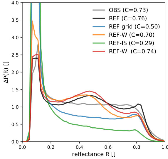
Figure 9. 0.6\mu m SEVIRI solar reflectance histograms for the test period computed for the observations (OBS) and the reference experiment (REF). The additional distributions were computed using only the grid-scale clouds (REF-grid), only the water clouds (REF-W) and only the ice clouds (REF-IS) of the reference experiment, respectively. For the red line (REF-WI) water and ice clouds are taken into account and only the snow contribution to the ice clouds was omitted. The numbers in the legend indicate the cloudiness, i.e. the fraction of pixels exceeding a reflectance of 0.2.
