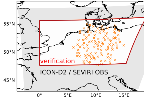
Figure 1. ICON-D2 domain in observation space (gray shaded) and the reduced verification domain (red box). Orange x indicate DWD’s pyranometer stations measuring global horizontal irradiance.
