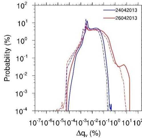
Figure 3: Probability distribution of the ratio of the change in water vapor concentration due to the impact of cirrus ice crystals and the aviation induced increase in the water vapor ‘ \Delta q_v ’ at aerosol activation, roughly 1 second after emission, for the 24 th 6am (blue) and 26 th April 2013 5pm (red) for areas with temperatures lower than 233.15K, ice saturation ratio larger than 1 and IWC larger than 10^{-11} \text{ kgm}^{-3} . The water vapor emission index is set to 1.25 \text{ kg kg-fuel}^{-1} . Cloud properties for the two days are displayed in figure 2. Dashed lines indicate the change in the aviation induced increase in water vapor due to the sublimation of cirrus ice crystals in the combustor only and solid lines indicate the change when also accounting for the sublimation of cirrus ice mixed into the plume and the deposition on cirrus ice once the plume is ice supersaturated.
