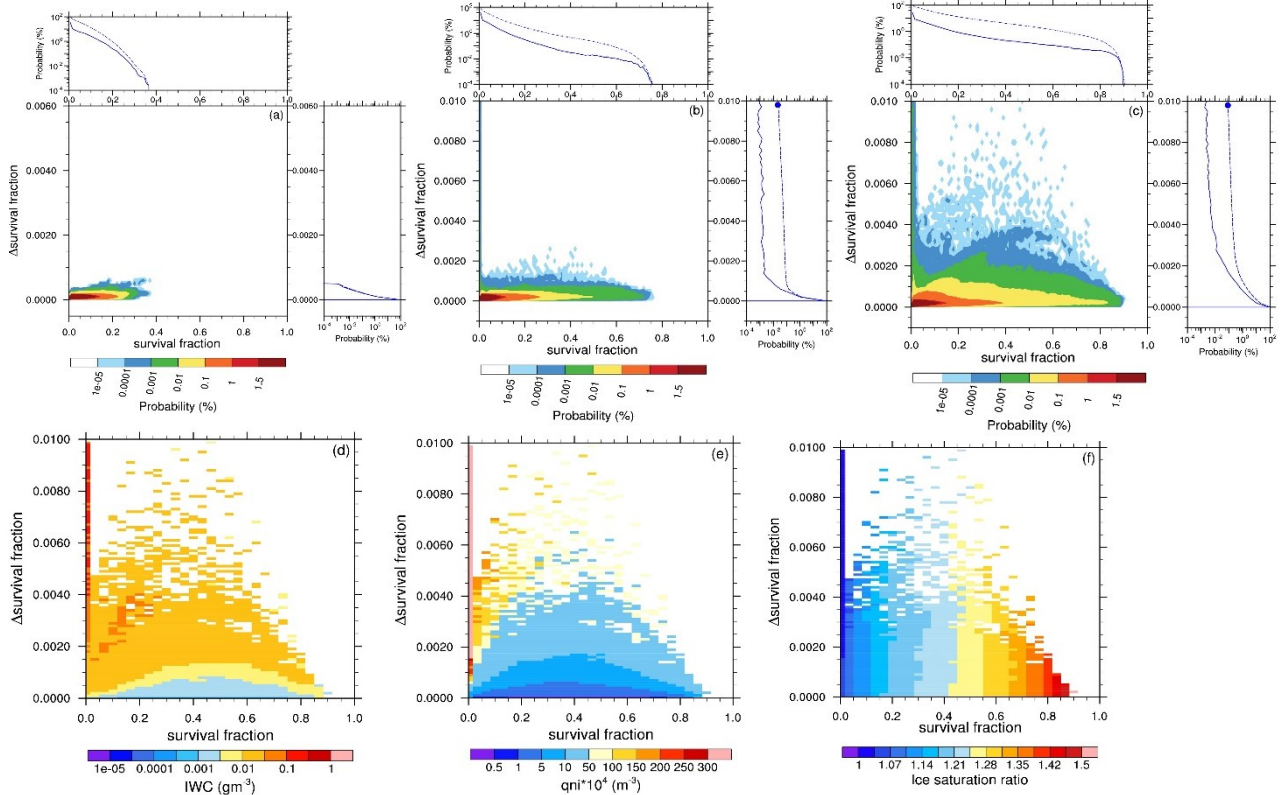
Figure 7: Joint probability distribution of contrail ice crystal survival fraction during the vortex phase when neglecting the impact of cirrus ice crystals (SF) and its change due to the presence of cirrus ice crystals ( \Delta SF) for (a) the 24 th April for 80% reduced soot number emissions and for the 26 th April 2013 for (b) current soot number emissions, 2.5 \cdot 10^{15} kg-fuel -1 , and (c) 80% reduced soot number emissions. Furthermore, cirrus properties for combinations of SF and \Delta SF for the 26 th April (d) ice water content ‘IWC’, (e) cirrus ice crystal number concentration ‘qni’ and (f) in-cloud ice saturation ratio. In (a) – (c) the PDF of the fraction of surviving ice crystals (solid) and the associated cumulative PDF (dashed) when neglecting the impact of natural cirrus ice crystals (top) and its change due to the presence of cirrus ice crystals (right) is additionally shown. The dot in the probability distribution of the change in survival fraction (c, right) indicates the probability of changes in the survival fraction that are larger than 1%. Analysis was restricted to areas where ambient temperature is at least 5K below the formation threshold temperature. A Brunt-Väisälä frequency of 0.012 \text{ s}^{-1} (strong stability) has been assumed for all cases.
