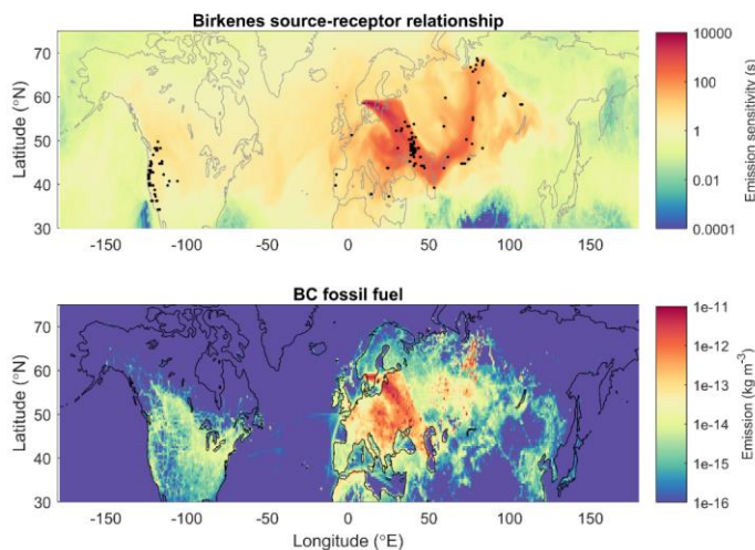
Figure 10 BC source-receptor relationship at Birkenes (2 October 2020 00:00 – 4 October 2020 00:00) modelled with FLEXPART in backwards mode ( top ) and BC fossil fuel emissions ( bottom ). Markers in the top panel indicate locations with BC emissions from biomass burning that contribute 0.1 > \text{ng m}^{-3} to BC concentrations at Birkenes. Only emissions that contribute to the modelled concentrations at Birkenes are included in the lower panel. The source-receptor relationship includes air masses up to 100 m above ground level.
