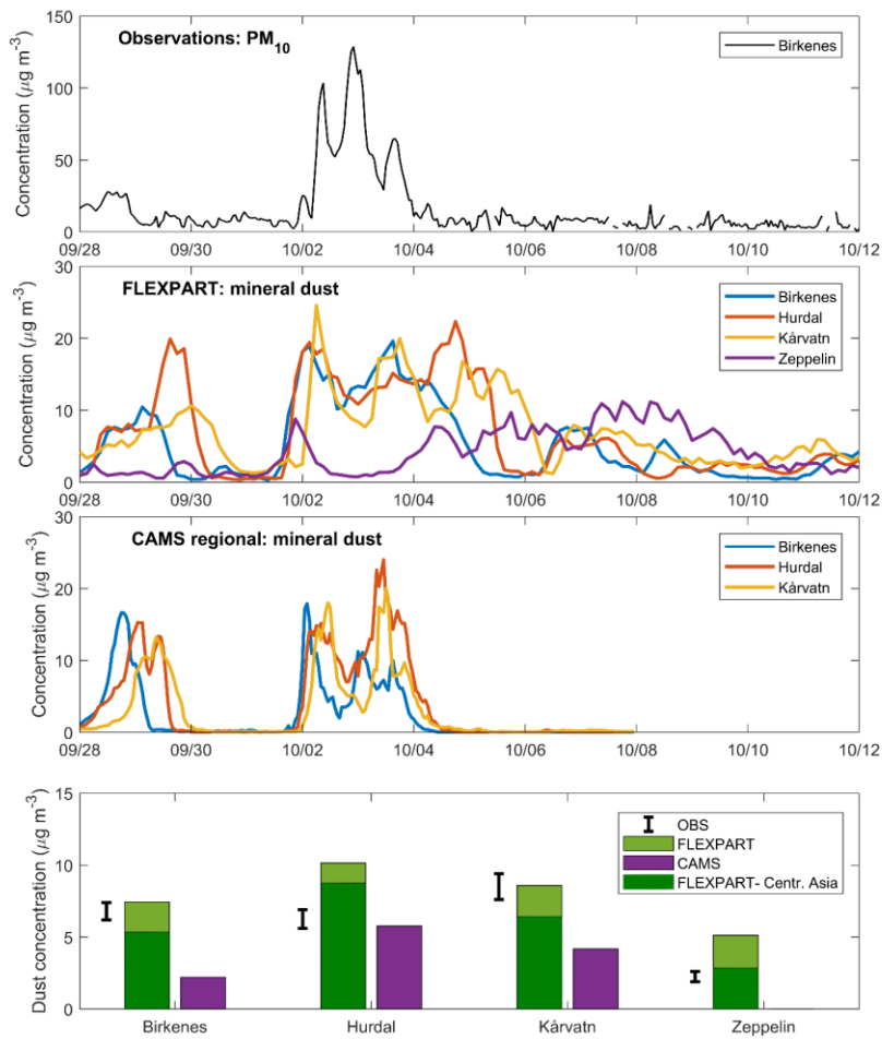
Figure 7 PM 10 concentrations observed at Birkenes (a). Mineral dust surface concentrations as simulated with FLEXPART (b) and CAMS-regional (c) at three stations in Norway and the remote station (outside CAMS domain). Bottom panel (d); mean concentrations from simulations compared to observations from weekly samples for Birkenes (30 September – 7 October 2020), Hurdal and Kärvatn (28 September – 5 October 2020) and Zeppelin (2 – 12 October 2020). For FLEXPART estimates in the bottom panel (d) light green colours indicate dust from global sources and dark green colours indicate the contribution of dust from Central Asia only.
