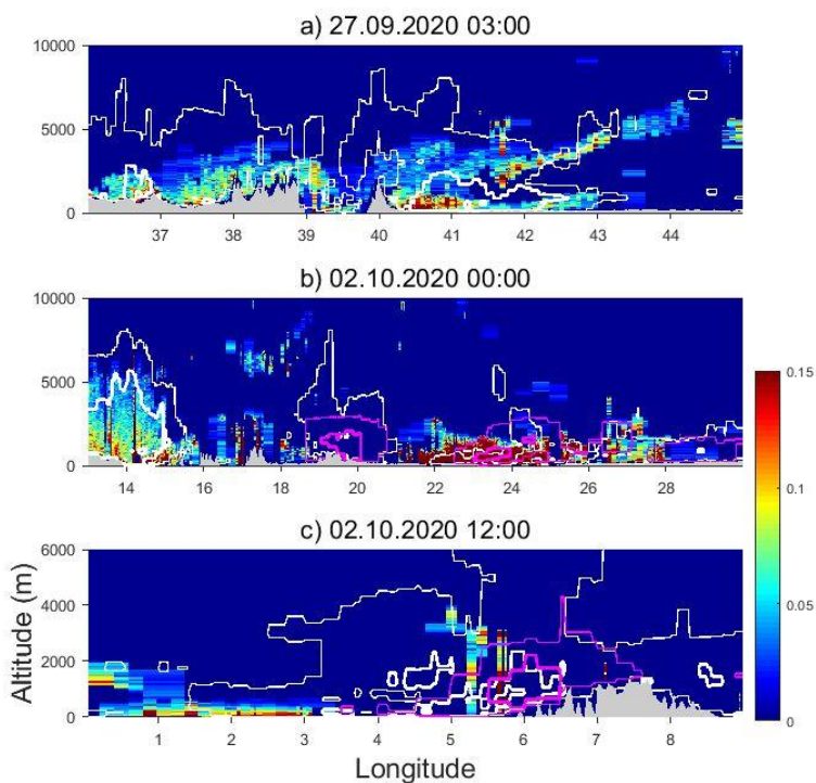
Figure 6 Aerosol extinction at 532 nm [units: km -1 ] during three overpasses (see Fig. 5 for location) is shown as colour plot (a. CALIOP overpass from 26 Sept. 2020, time of first record 23:48, b: 2. October 2020 01:18, and c. 2 October 2020 11:55). The titles of panels a-c indicate the FLEXPART 3-hourly time step corresponding to the overpass. White contours show FLEXPART mineral dust concentrations (thick and thin lines, top: 40 and 6 \mu\text{g m}^{-3} , middle: 50 and 10 \mu\text{g m}^{-3} , bottom: 15 and 3 \mu\text{g m}^{-3} ). Magenta contours show FLEXPART BC concentrations (thick and thin lines, top: none, middle: 50 and 5 \text{ng m}^{-3} , bottom: 40 and 10 \text{ng m}^{-3} ).
