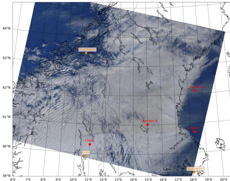
305 Figure 2 RGB from OLCI bands 3, 6 and 8 centred at 442.5, 560 and 665 nm. Data from 2 Oct 2020, 09:33 UTC.
