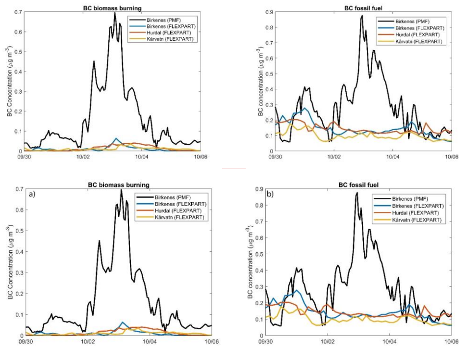
Figure 8 eBC_{BB} (left) and eBC_{FF} (right) concentrations retrieved with PMF from observations at Birkenes (black) and simulated with FLEXPART at Birkenes, Hurdal and Kärvatn.
