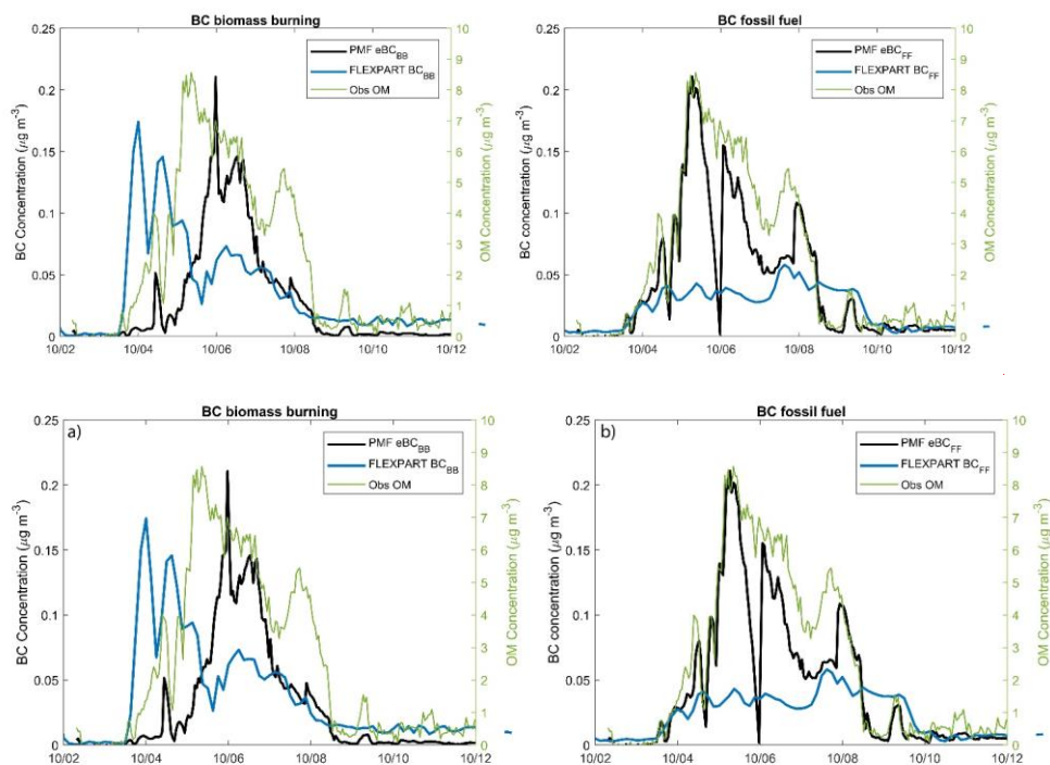
Figure 9 eBC_{BB} (left) and eBC_{FF} (right) concentrations retrieved with PMF from observations (black) and simulated with FLEXPART (blue) and observed OM concentrations (green) at Zeppelin.
