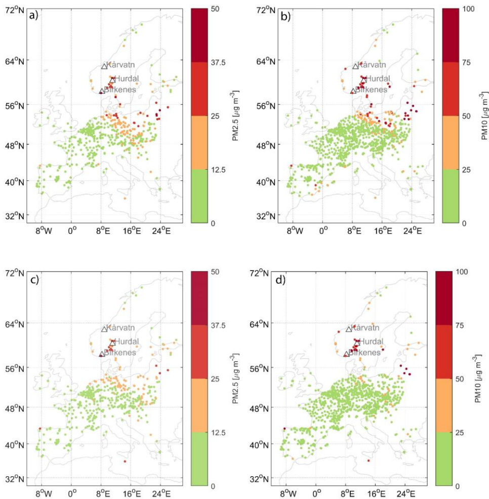
Figure 1 Mean PM 10 and PM 2.5 (a,c) and PM 10 (b,d) values on 2 (a,b) and 3 (c,d) October 2020 (4824-hour mean) at all EEA air quality background sites (includes urban as well as rural, but sites close to roads are excluded). Triangles indicate three Norwegian rural background sites with extensive PM speciation (section 2.1.1). For comparison: The WHO air quality guidelines for maximum daily averaged PM 10 and PM 2.5 are 50 µg m -3 and 25 µg m -3 , respectively, and the EU limit value for PM 10 is 50 µg m -3 .
