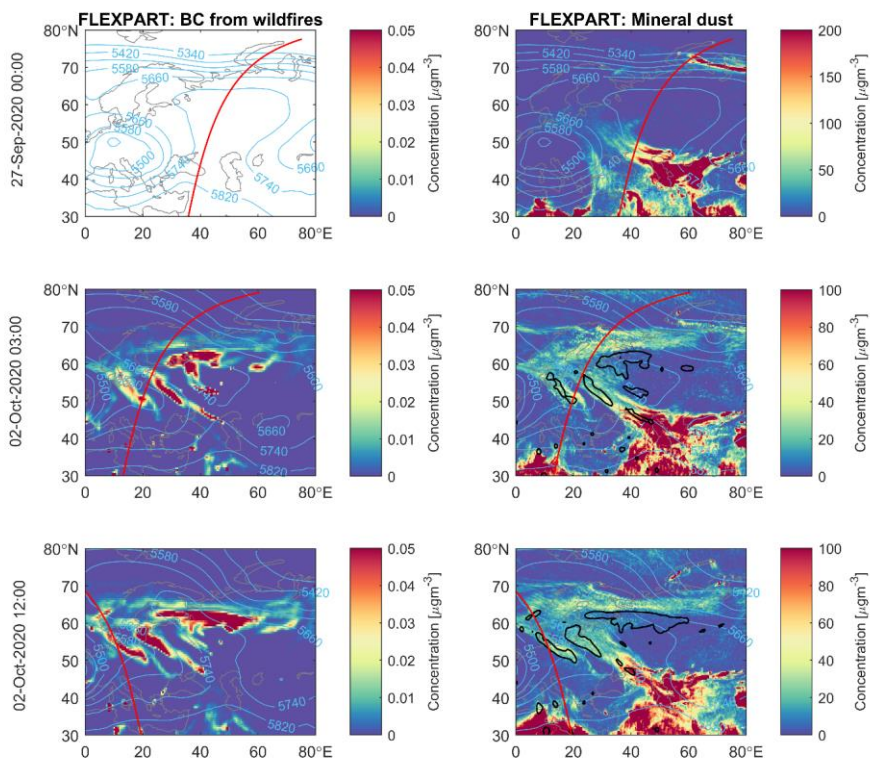
Figure 5 Modelled surface concentrations of BC from biomass burning (left a, c, e) and mineral dust (right b, d, f) on 27 September 2020 and 2 October 2020 (midnight and noon). Blue contours: ECMWF 500 hPa geopotential height (m). In the right column black contour lines indicate the regions of the modelled wildfire plume ( BC > 0.03 \mu\text{g m}^{-3} ) as shown in the left column. BC simulations started only after 27 September 2020 because no relevant emissions were observed for the episode in Norway. The red lines indicate the location of CALIOP overpasses shown in Fig. 6.
