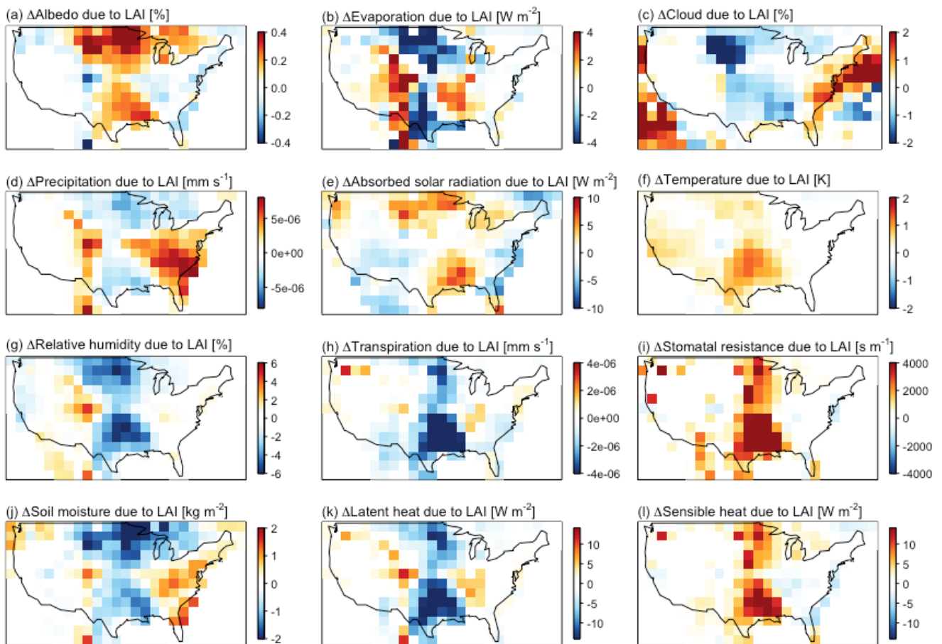
14 15 Figure 7. Summertime changes in (a) albedo, (b) ground evaporation, (c) cloud cover, (d) precipitation, (e) absorbed solar 16 radiation, (f) surface temperature, (g) relative humidity, (h) vegetation transpiration, (i) stomatal resistance, (j) soil moisture, 17 (k) latent heat flux, and (l) sensible heat flux driven by LAI increase with dynamic meteorology.
