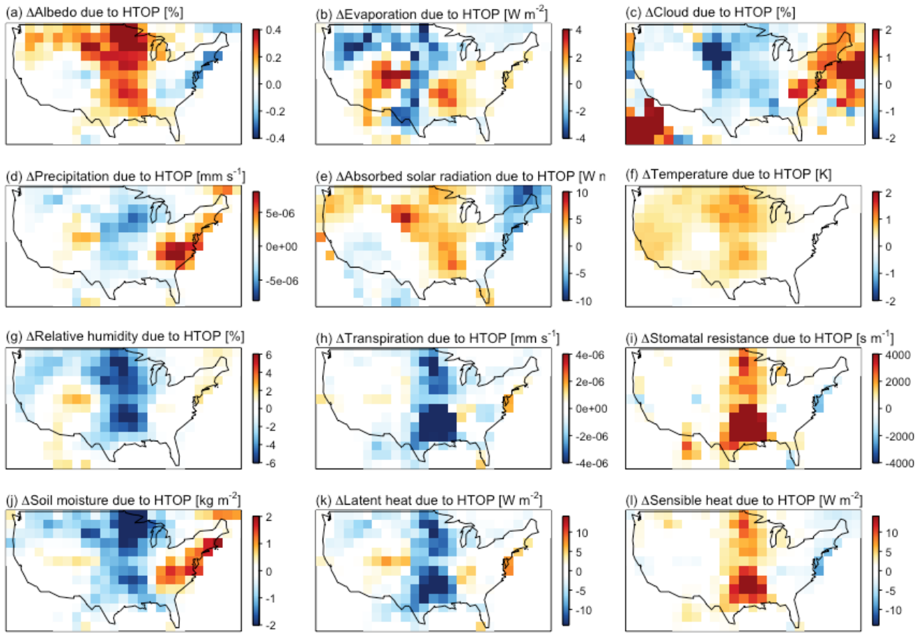
1 2 Figure 8. Same as Fig.7 but driven by canopy height increase.
