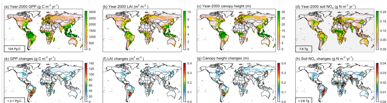
21 Figure 4. Annual mean of year-2000 (a) gross primary production (GPP), (b) leaf area index (LAI), (c) canopy height, (d) soil 22 NO x emission, and corresponding increases (e-h) due to increased nitrogen deposition over 2000–2050.
