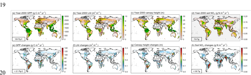
20 21 Figure 4. Annual mean of year-2000 (a) gross primary production (GPP), (b) leaf area index (LAI), (c) canopy height, (d) soil 22 NO x emission, and corresponding increases (e-h) due to increased nitrogen deposition over 2000–2050.
