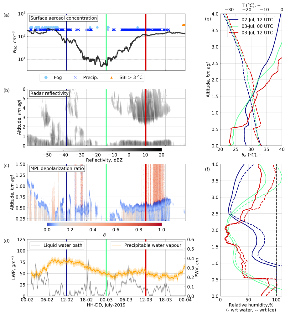
Figure 11. Conditions during the 03 July 2019 low aerosol case study. (a) Surface N_{20} (CPC), with occurrences of fog (OPC-N3), precipitation (POSS), and SBI > 3^{\circ}\text{C} events indicated. (b) Radar reflectivity (MMCR). (c) Lidar depolarisation ratio (MPL), blue colours represent liquid droplets and reds are ice crystals. (d) Column integrated liquid water path and precipitable water vapour (MWR). (e) Temperature (dashed) and equivalent potential temperature (solid) radiosonde profiles. (f) Relative humidity with respect to water (solid) and ice (dashed) from radiosonde profiles. The coloured vertical lines on the left-hand plots correspond to the time of each vertical radiosonde profile in the right-hand plots.
