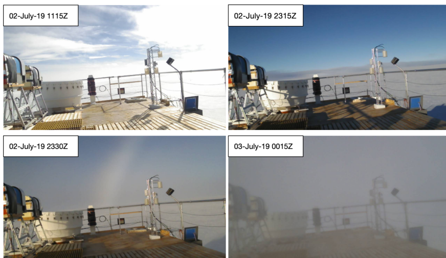
Figure 12. Photographs from a webcam oriented towards the eastern horizon on 02-03 July 2019. The aerosol inlet is visible mounted on the mast in the SE corner.
