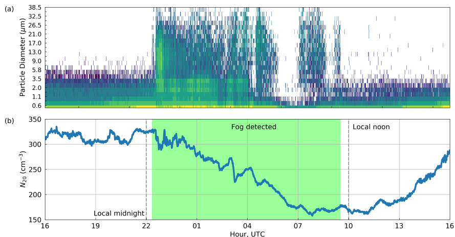
Figure 3. (a) Particle size distribution from the OPC-N3 from 31 July 2019 16:00 UTC to 01 August 2019 16:00 UTC (1 min averages). (b) N_{20} particle number concentration from the CPC during the same period (1 min averages). The duration of the fog event identified by the methodology described in Section 2.2 is shaded in green.
