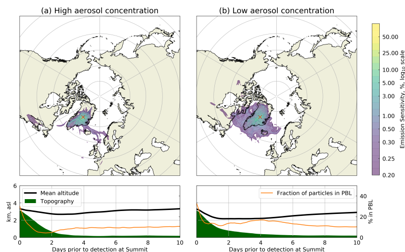
Figure 9. Results from FLEXPART back trajectory simulations averaged over the high N_{20} events (a) and the low N_{20} events (b). Upper: Surface emission sensitivity aggregated over 20 days prior to detection at Summit (as a percentage of the maximum value). Lower: Mean altitude and fraction of particles within the planetary boundary layer (PBL) for all simulated particles over the 10 days prior to detection.
