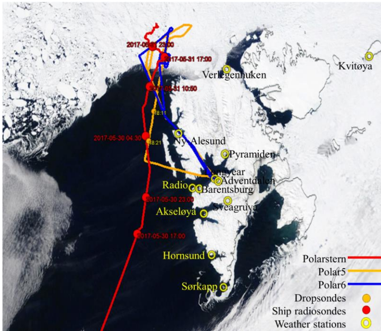
Figure 1: Satellite visible image (Modis corrected reflectance from NASA Worldview, https://worldview.earthdata.nasa.gov )
