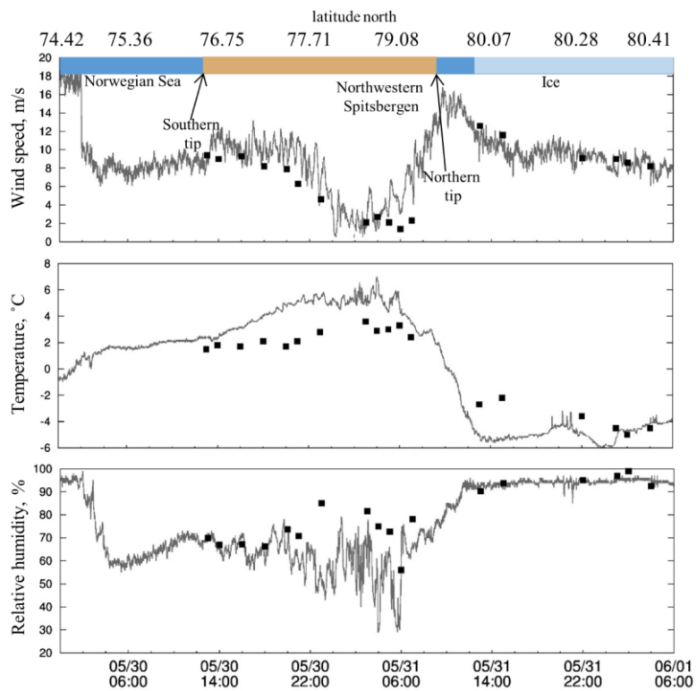
Figure 53: Wind speed (top), air temperature (center) and relative humidity (bottom) measured on RV Polarstern on 30-31 May 2017. Black squares show modelling data at the grid points nearest to the Polarstern track. Color panels on the top show when RV Polarstern was in the open sea (blue), downwind from Svalbard (brown) and in the sea ice (light blue)
