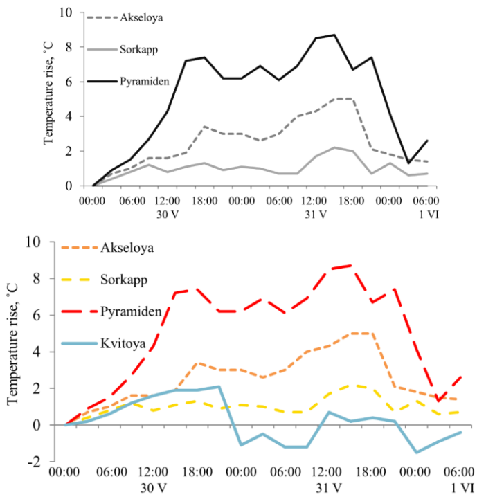
775 Figure 46: Temperature change from 'initial' time at each individual AWS station during foehn episode, where the initial time is 00 UTC 30 May. Temperature rise (observed temperature "minus" temperature at the initial time (00 UTC 30 May)) during foehn episode according to AWS observations.
