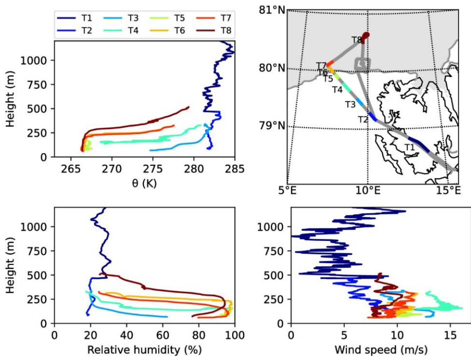
Figure 911: Vertical profiles of potential temperature (left top), relative humidity (left bottom) and wind speed (right bottom) as observed by the Polar 6 aircraft along its track line (right top). Gray shading in the upper right panel corresponds to the
