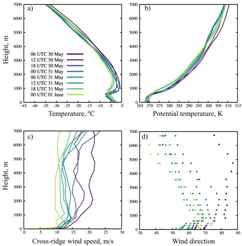
Figure B1: Vertical profiles of incoming flow during episode 2017 according to WRF modelling: a) air temperature, b) potential temperature, c) cross-ridge wind component and d) wind direction
