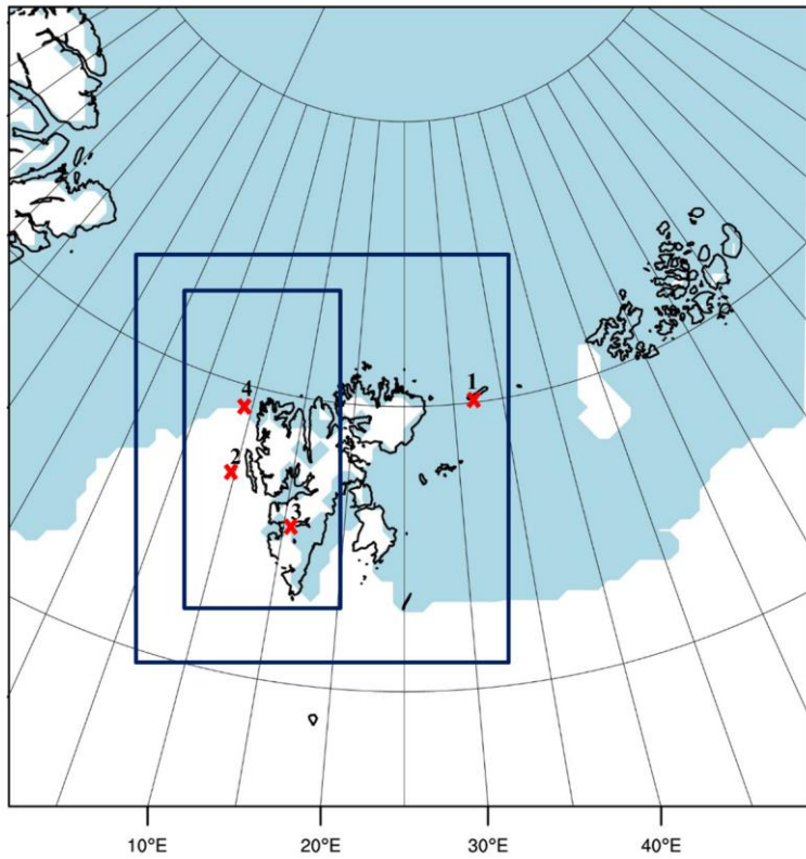
Figure 2: WRF outer domain 1 and nested domains 2 and 3. Sea ice is shaded. Red X-marks show points where vertical profiles were analyzed in Figure 9
