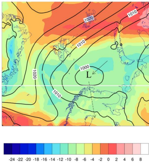
760 Figure 23: Synoptic chart at 06 UTC 30 May 2017 according to ECMWF YOPP analysis: sea-level pressure (black contours, every 5 hPa) and air temperature at 850 hPa level (color, every 2 K). Arrows show movements of cyclone center during May 29-31
