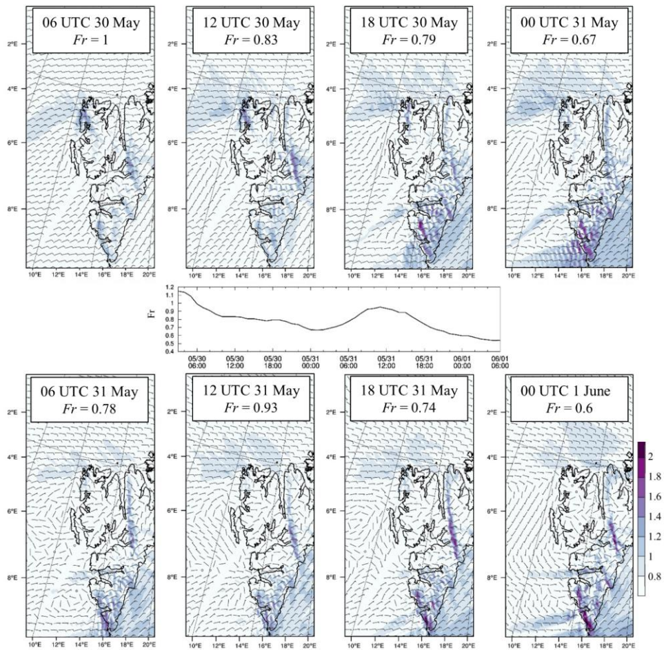
Figure 1012: Dynamics of orographic flows during the observed episode 2017: wind speed (at 10 m AGL) normalized to windward wind speed (averaged in the lowest 1.7-km layer in 80°N, 35°E (near Kvitøya)) (color) and wind direction (barbs) at 10 m AGL and Fr number in the incoming flow (in the center) according to WRF modelling
