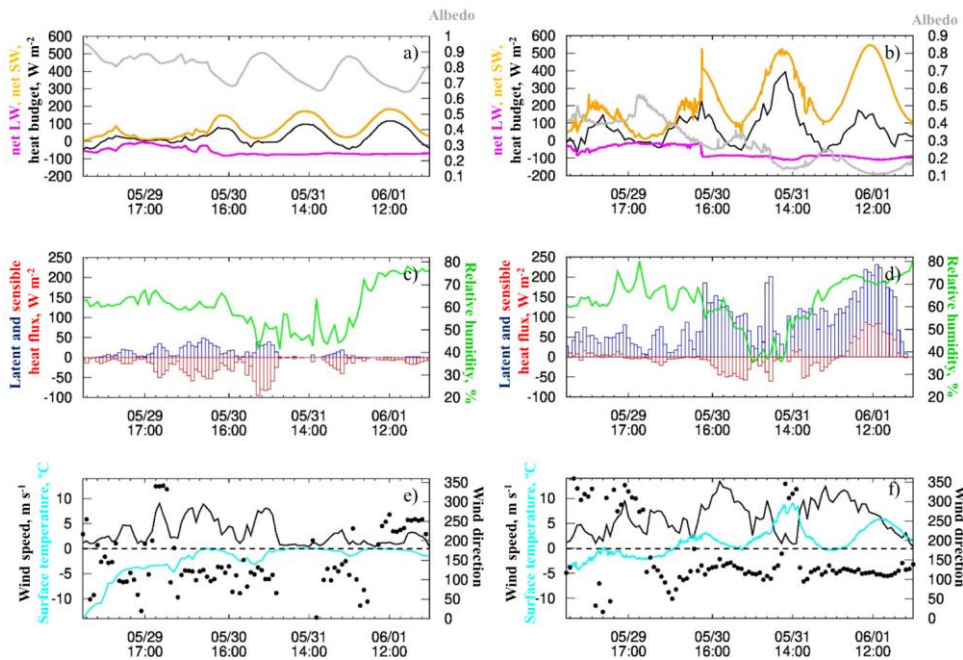
Figure 1113: Terms of radiation and heat budget in Ny-Alesund (left) and Adventdalen (right) during 29 May – 1 June 2017:
