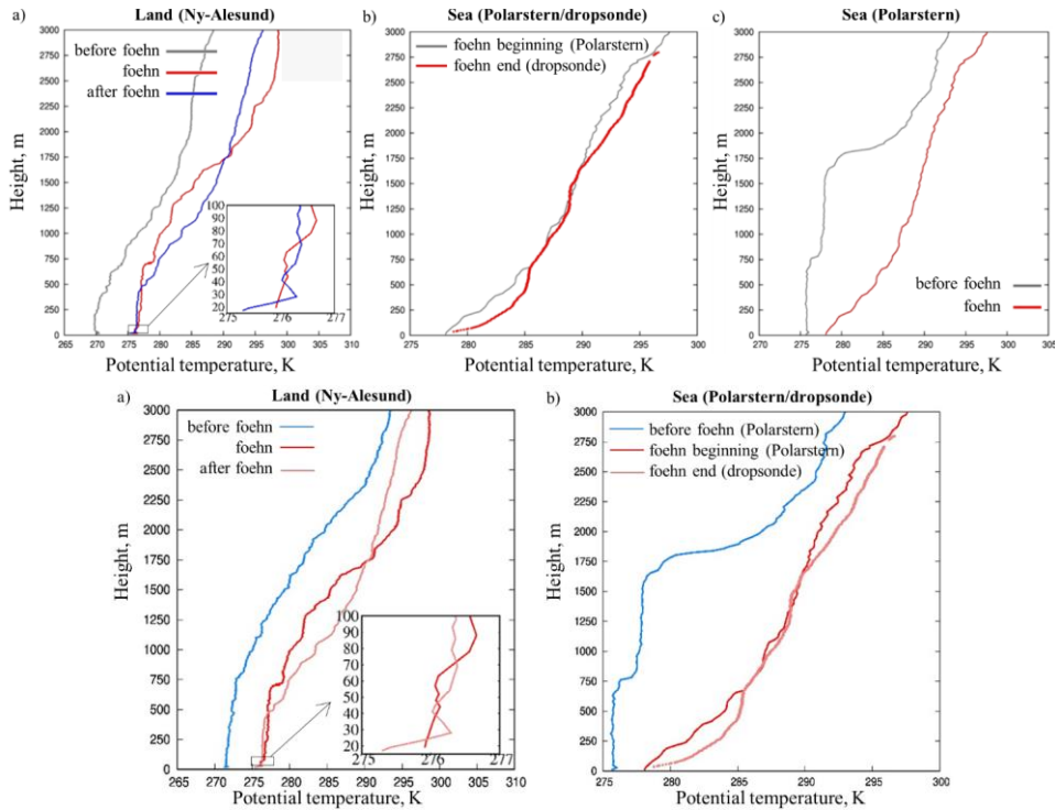
Figure 810: Observations of potential temperature in the lower troposphere a) over land (Ny-Alesund) and b),-e) over sea. a) Radiosonde observations over Ny-Alesund before foehn onset (12 UTC May 29), during foehn (12 UTC May 30) and after foehn episode (12 UTC June 1). The lowermost 100-m layer is zoomed (see inset). b) Polarstern radiosonde observations at 11:00 May 30 (south from Spitsbergen), at 04:34 May 31-and dropsonde observations at 18:21 May 31. The latter two observations were taken in front of north-western Spitsbergen, in the beginning and in the end of foehn episode, respectively.
