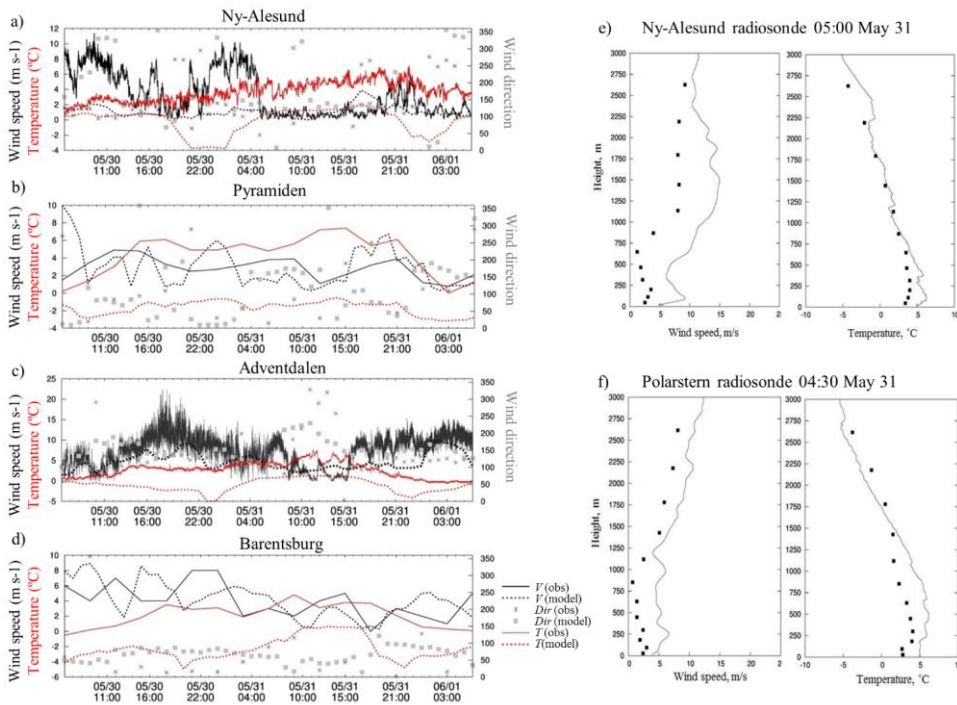
830 Figure A1: WRF model verification against AWS (a-d) and radiosonde data in Ny-Alesund (e) and Polarstern (f). a-d) 10-m wind speed V_{10} (black lines), 2-m temperature T (red lines) and wind direction Dir (asterisks and squares) according to AWS observations (solid lines and asterisks) and WRF simulation (dotted lines and squares). Wind speed at Adventdalen station was measured with sonic anemometer at 2.7 m AGL. e-f) Wind speed (left) and temperature (right) according to observations (solid line) and WRF simulation (squares).
