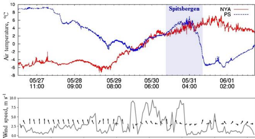
Figure 4: a) Time series of air temperature in Ny-Alesund (NYA) and on RV Polarstern (PS) as shown similarly by Knudsen et al. (2018). Blue shading shows the time period when Polarstern was downwind from Spitsbergen. b) Time series of wind speed (line) and direction (arrows) in Ny-Alesund
