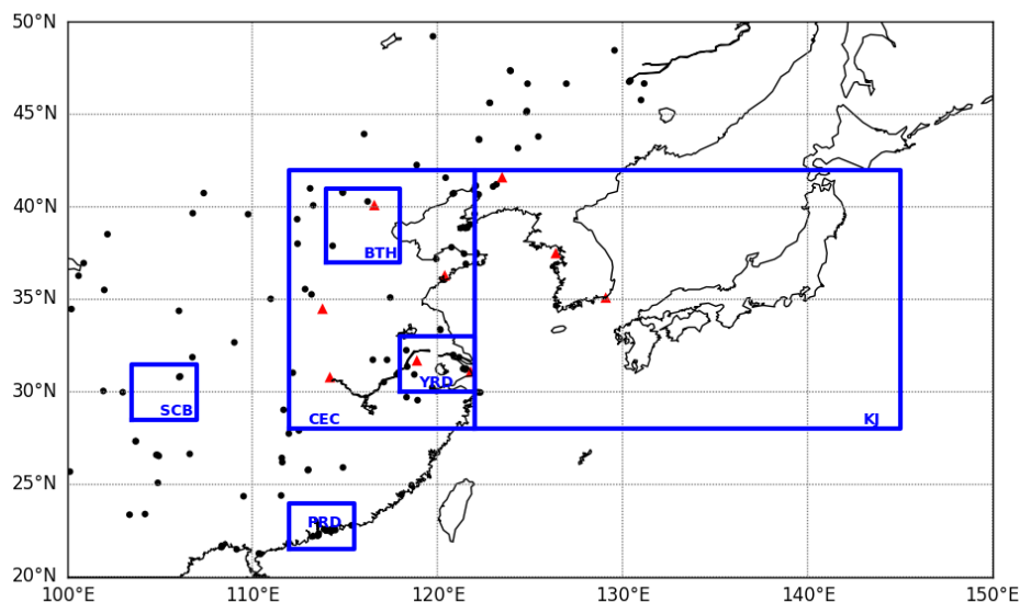
15 Figure 1: Northeast Asian domain of the study. Six subregions of interest are considered: the Central East China (CEC, 28-42°N, 112-122°E), the Beijing-Tianjin-Hebei region (BTH, 37-41°N, 114-118°E), the Yangtze River Delta (YRD, 30-33°N, 118-122°E), the Pearl River Delta (PRD, 21.5-24°N, 112-115.5°E), the Sichuan Basin (SCB, 28.5-31.5°N, 103.5-107°E), and the Korea-Japan region (KJ, 28-42°N, 122-145°E). Black circles show the rural-type surface stations and the red triangles the IAGOS airports used in this study.
