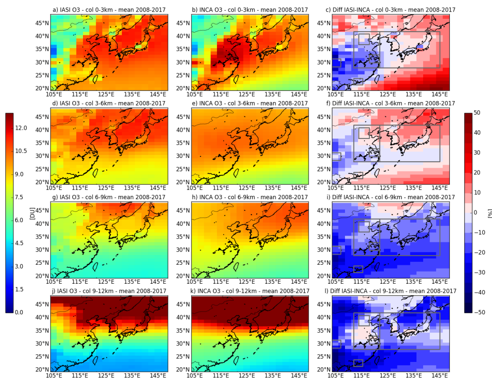
Figure 3: Mean O_3 partial columns for 2008-2017 observed with IASI (left panels), simulated by INCA (middle panels), and their differences (right panels). For different partial columns are considered: the lowermost tropospheric columns from the surface to 3 km altitude (named 0-3km), the lower free tropospheric columns from 3 to 6 km altitude (named 3-6km), the upper free tropospheric column from 6 to 9 km (named 6-9km), and the upper tropospheric column from 9 to 12 km (named 9-12km).
