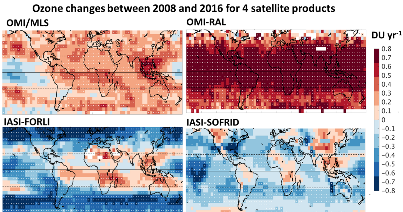
Figure B2: Global gridded ozone trends between 2008 and 2016 derived for the tropospheric columns from four satellite products (OMI/MLS, OMI-RAL, IASI-FORLI, and IASI-SOFRID) in the TOAR-I framework. The figure is an extension/update of Fig. 24 from Gaudel et al. (2018), under the CC-BY 4.0 copyright.
