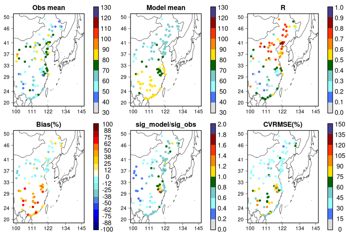
5 Figure A1: Mean daily O_3 concentrations (in \mu\text{g}/\text{m}^3 ) observed at the rural-type Chinese stations and simulated by INCA for 2014-2017. The statistics of the comparison at each station is shown with the correlation coefficient (R), the mean bias, the ratio of the standard deviation of the model and the observations, and the coefficient of variation of the Root Mean Square Error (CVRMSE).
