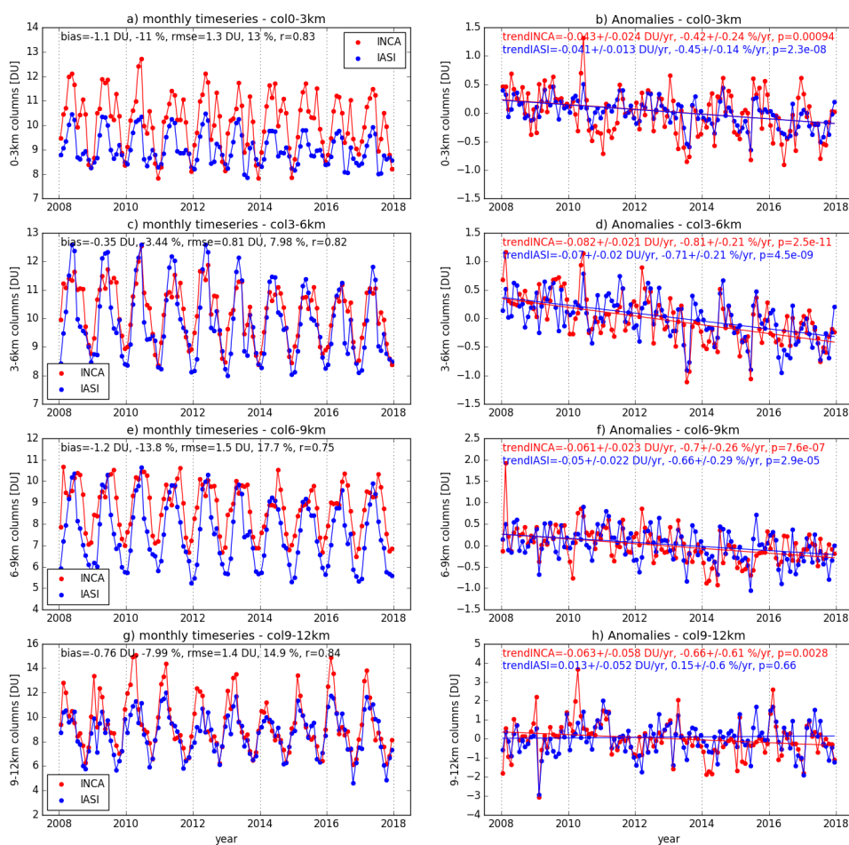
Figure 4: IASI and INCA monthly timeseries (left) and anomalies (right) for the 0-3km, 3-6km, 6-9km, and 9-12km O 3 partial columns over the CEC region for 2008-2017. Biases, RMSE and Pearson correlation coefficient between the IASI and INCA monthly timeseries are provided as well as the trends, uncertainties, and associated p-values calculated from the anomalies timeseries.
