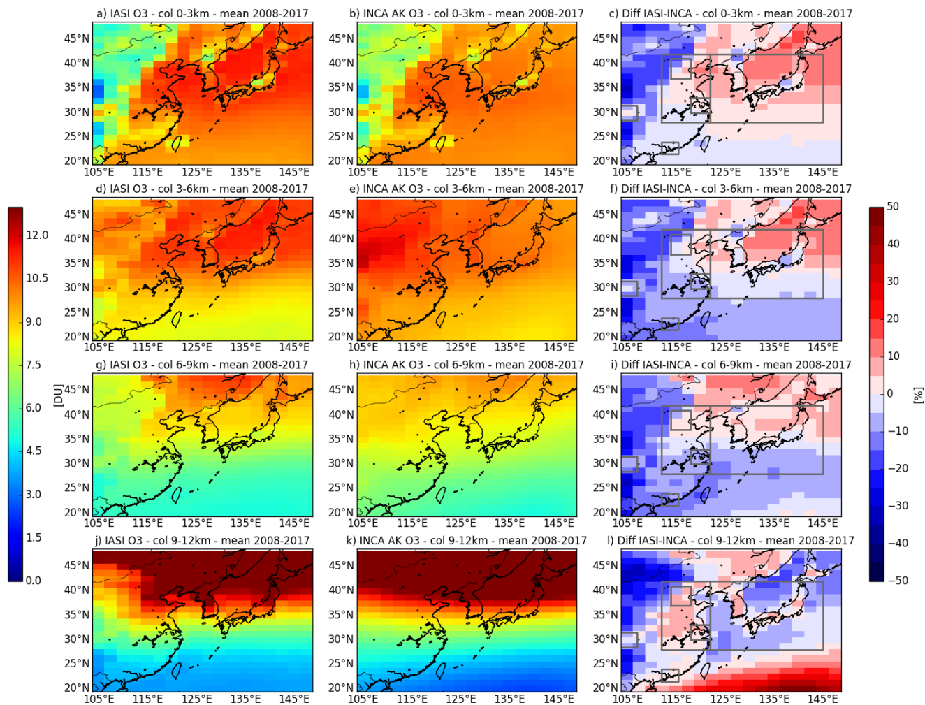
Figure A2: Mean O 3 partial columns for 2008-2017 observed with IASI (left panels), simulated by INCA (middle panels), and their differences (right panels). The INCA ozone profiles are smoothed by each individual IASI AKs. Four different partial columns are considered: 0-3km, 3-6km, 6-9km, and 9-12km columns.
