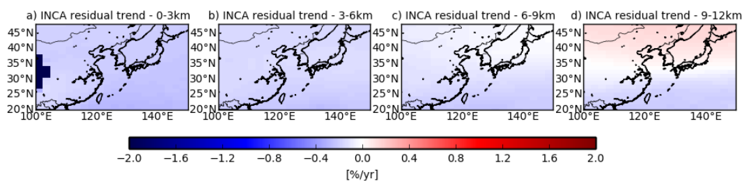
Figure B1: Residual O 3 trend derived from the INCA simulation in which all the emissions, CH 4 and meteorology are kept constant to their 2007 values. The trend is calculated for the 0-3km, 3-6km, 6-9km, and 9-12km O 3 partial columns.
