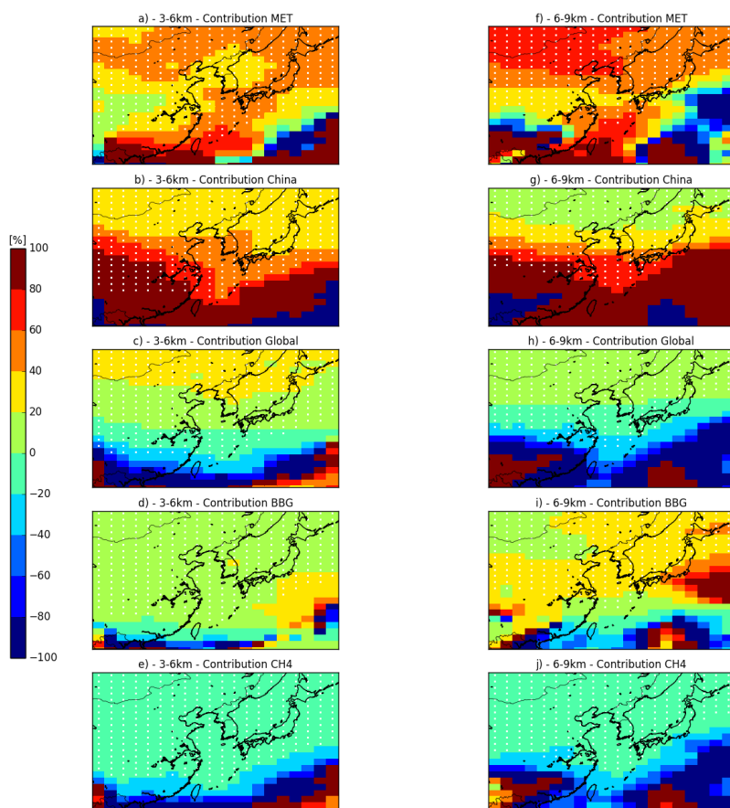
10 Figure 6: Contributions of the meteorological variability, the Chinese anthropogenic emissions, the global anthropogenic emissions, the global biomass burning emissions and the CH 4 to the trends calculated for the 3-6km and 6-9km partial columns (see Table 4 for details on the sensitivity tests).
