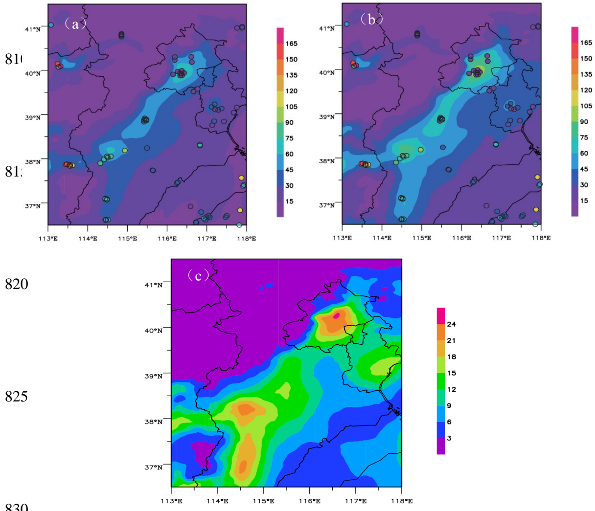
Fig. 9 Spatial distribution of 72-h averaged SO 2 concentration simulated with (a) a priori and (b) posteriori ES, and (c) the increment during December 28-30, 2016. Color solid dot denotes the measurements.
