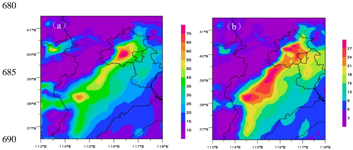
Fig. 4 Spatial distributions of 96-h averaged sensitivity coefficients ( \mu\text{g m}^{-3} ) of (a) SO 2 and (b) NO x concentrations with respect to SO 2 and NO x ES during December 27–30, 2016.
