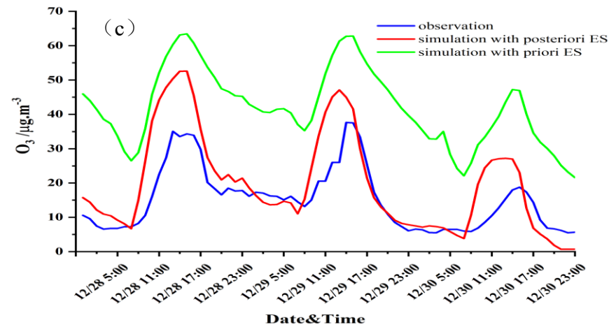
895 Fig.11 Time serial of regional averaged (a) SO 2 , (b) NO 2 , and (c) O 3 concentrations respectively simulated with a priori and a posteriori ES, and measurements at 45 stations in the BTH region during December 28–30, 2016.
