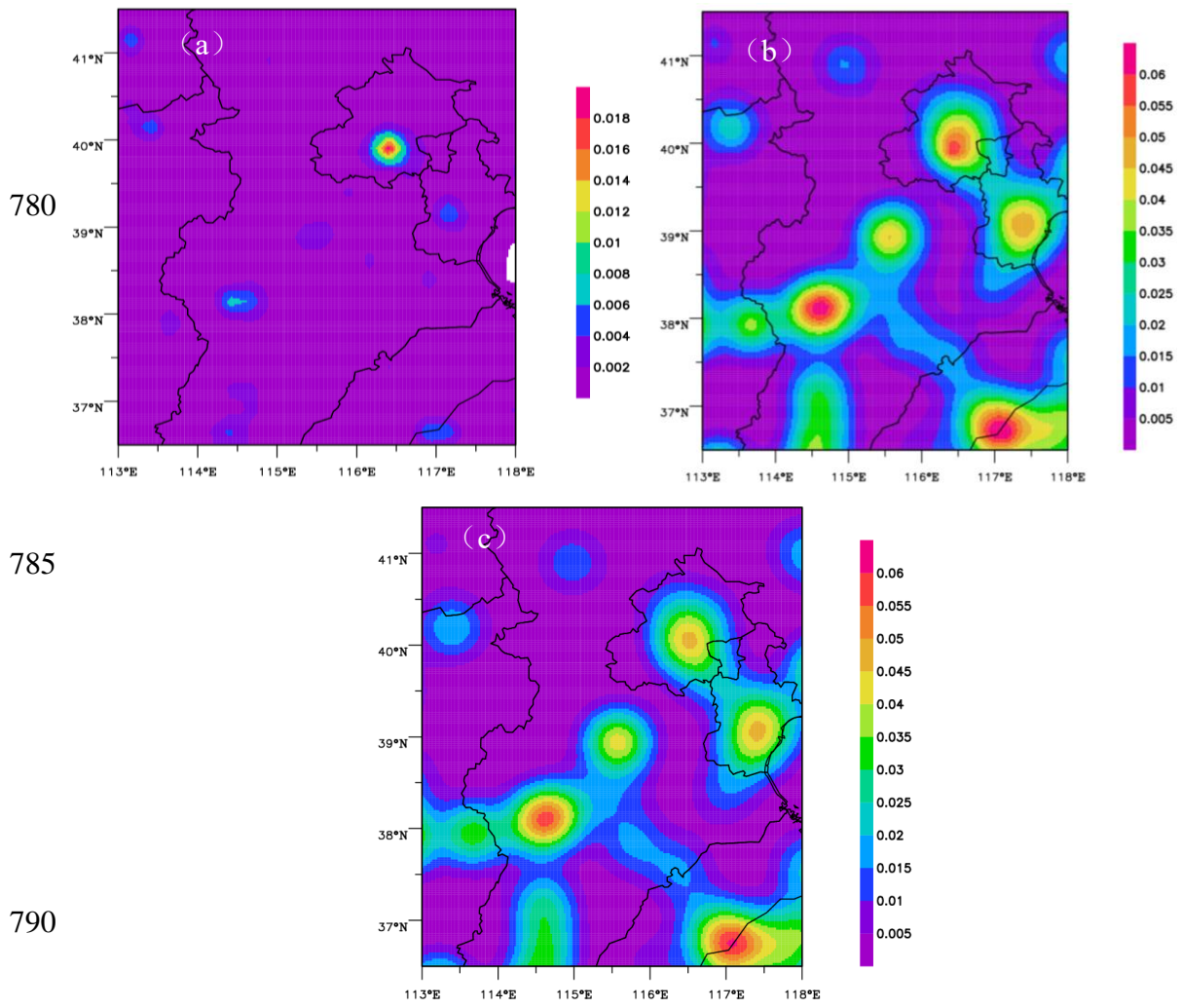
Fig. 8 Same to Fig.7 except for NO 2 .
