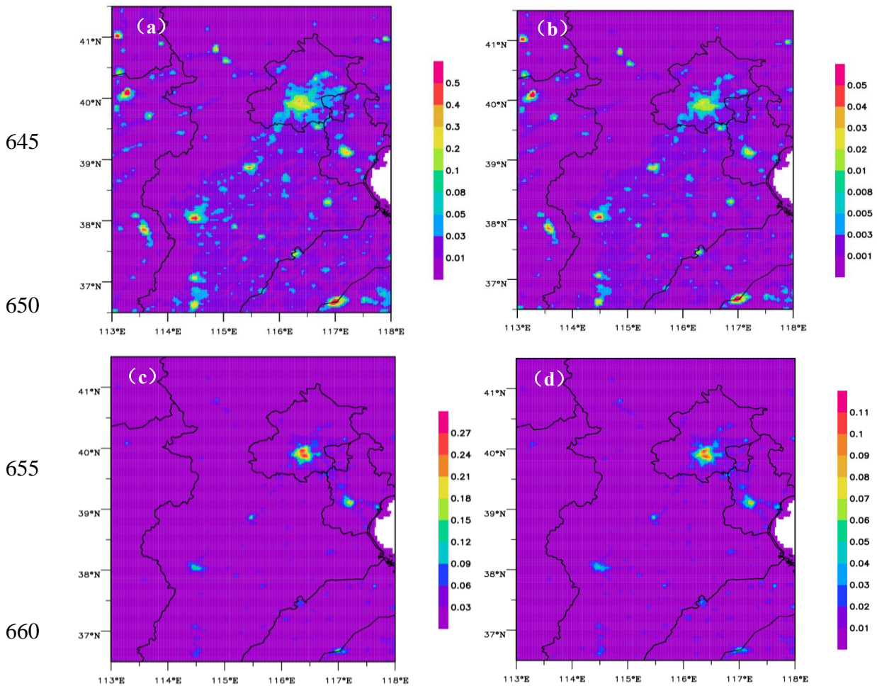
Fig. 2 Spatial distributions of (a) averaged emission rates of \text{SO}_2 ES, (b) standard deviation in the BEC of \text{SO}_2 ES, (c) averaged emission rates of \text{NO}_x ES, (d) standard deviation in the BEC of \text{NO}_x ES at 08:00 local time in December 2012. Unit: mole/s.
