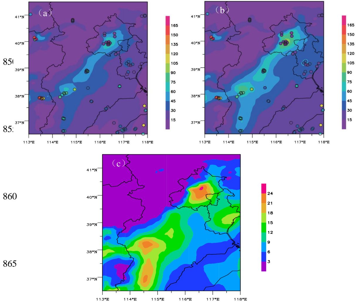
Fig. 9 Spatial distribution of 72-h averaged \text{SO}_2 concentration simulated with the (a) a priori and (b) a posteriori ES, and (c) the increment during December 28-30, 2016. Color solid dot denotes the measurements.
