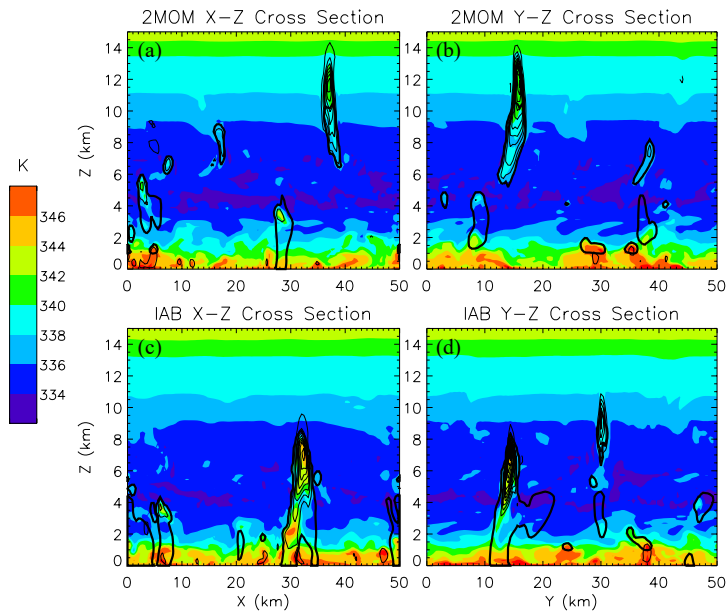
Figure 1. Cross sections (x-z in a and c; y-z in b and d) through cloud simulations at 360 min from (a, b) 2MOM and (c, d) IAB randomly selected ensemble members. Colors represent the equivalent potential temperature, the moist static energy divided by c_p . The thick contour shows total condensate (cloud and precipitation) of 0.1 \text{ g kg}^{-1} . Solid thin contours show vertical velocity starting with 1 \text{ m s}^{-1} and contour interval of 3 \text{ m s}^{-1} .
