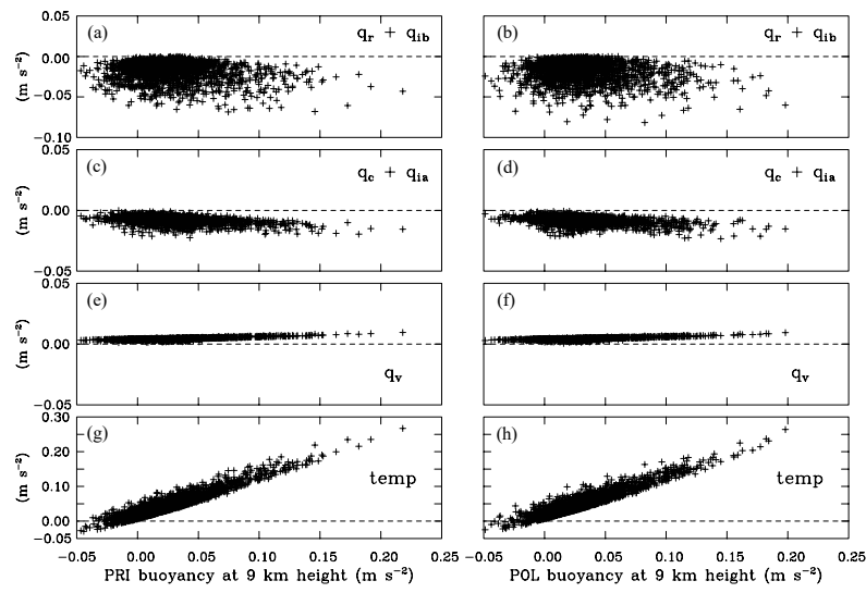
1070 Figure 9. As Fig. 8, but at 9 km. Panels (a,b) include rain combined with ice B mixing ratios; panels (c,d) include cloud water combined with ice A mixing ratio.
