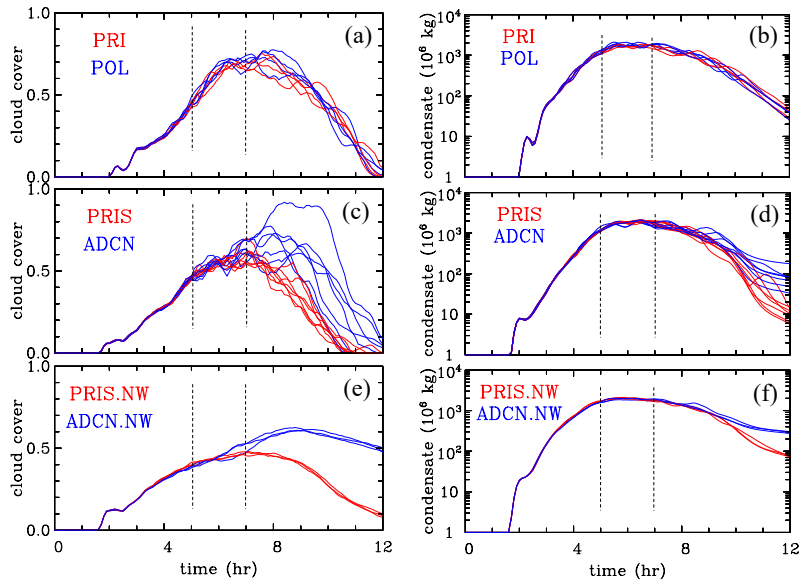
950 Figure 2. Evolution of (a, c, e) cloud cover and (b, d, f) total mass of cloud and precipitation inside the computational domain in (a, b) PRI and POL IAB ensembles, (c, d) PRIS and ADCN 2MOM ensembles, and (e, f) PRIS.NW and ADCN.NW 2MOM ensembles. Dashed vertical lines show the 6 th and 7 th hour period for which analyses are completed.
