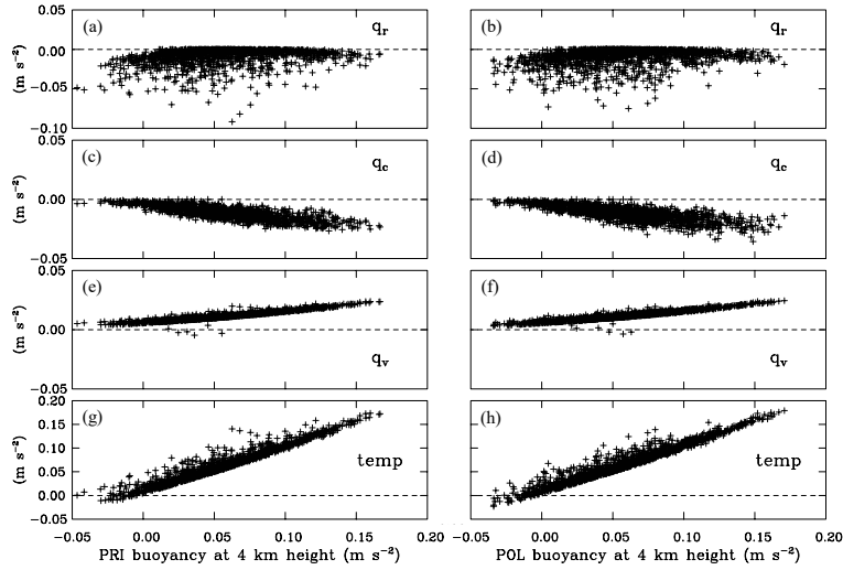
1050 Figure 8. Scatterplots of buoyancy components at 4 km as a function of the total buoyancy in (a, c, e, g) PRI and (b, d, f, h) POL of all 4 ensemble members of IAB simulations at hour 6 and 7. The horizontal axes in both columns represent the total buoyancy. Panels (g) and (h) show temperature buoyancy component. Panels (e) and (f) show the water vapor contribution. Panels (a), (b), (c) and (d) are the loading buoyancy components, separated into (c, d) cloud water and (a, b) rain components. Point with updraft larger than 1 m s -1 and total condensate larger than 1 g kg -1 are included. Only about 8% of data points is shown.
