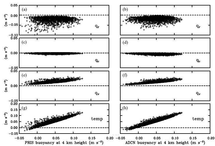
Figure 10. As Fig. 8 but for all 7 simulations (left panels) PRIS and (right panels) ADCN from 2MOM ensemble. Only 5% of data points are shown.
