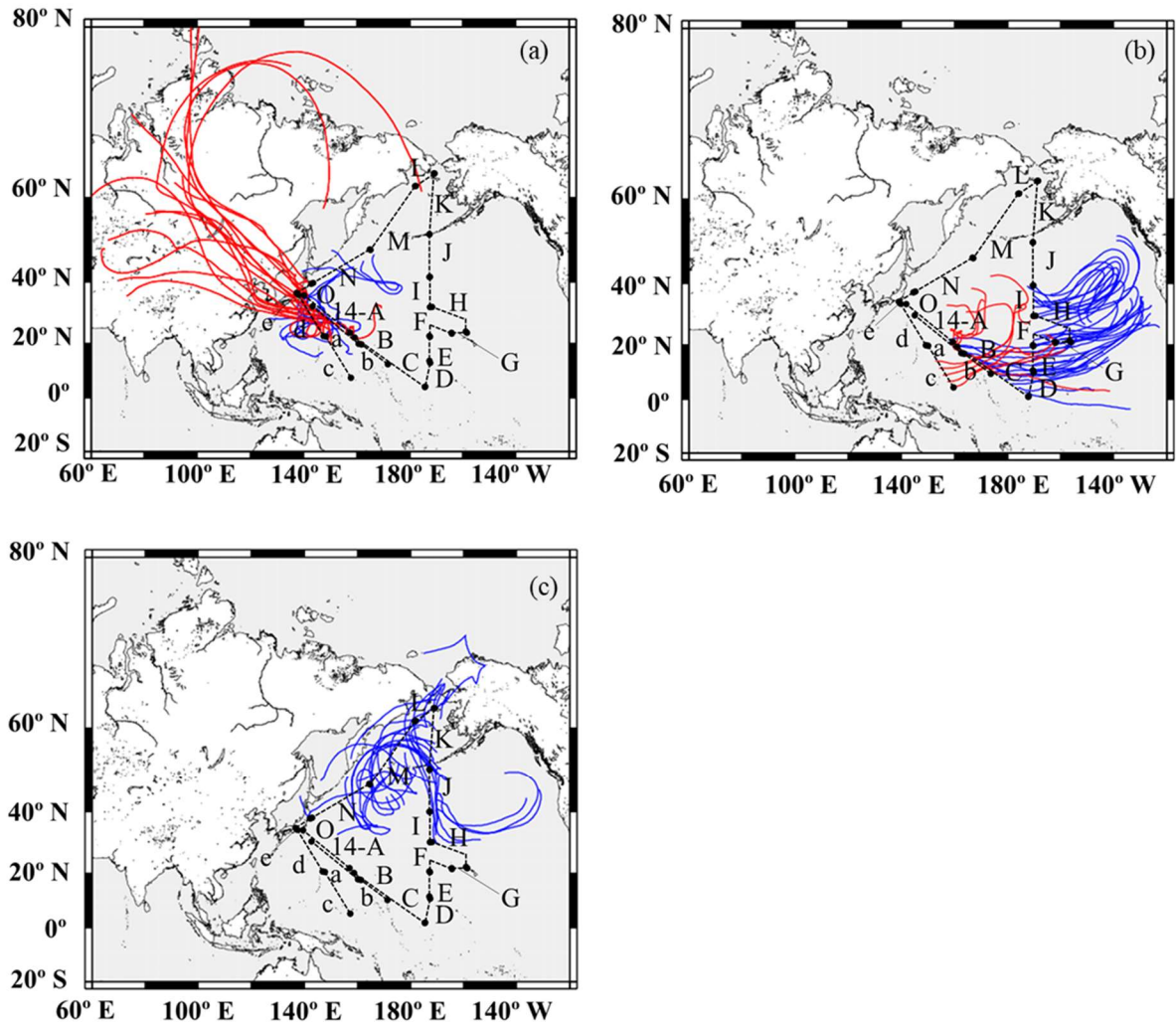
Figure 2. Seven-day backward trajectories along the ship tracks for (a) group I, (b) group II, and (c) group III. The arrival height was set to 500 m and a new trajectory was obtained every 612 hours. The maps were created using GMT. Red and blue lines indicate trajectories during the KH-13-7 and 14-3 cruises, respectively.
