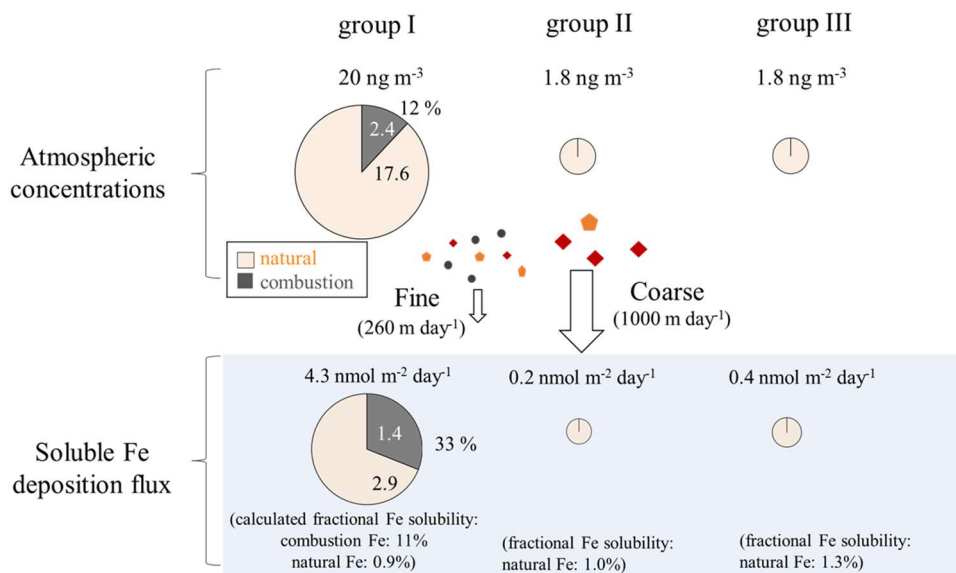
Figure 11. Summary of the contribution of combustion and natural Fe in atmospheric aerosols and soluble Fe depositions. The sizes of the pie charts are indicative of the magnitude of the atmospheric Fe concentrations and soluble Fe deposition fluxes.
