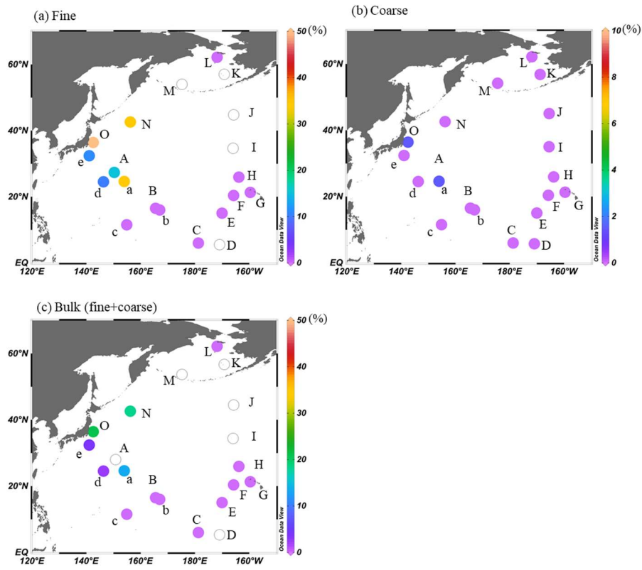
Figure 9. The contribution of combustion Fe in (a) fine, (b) coarse, and (c) total (fine + coarse) Fe in marine aerosols. Data with open circles were not determined. The figures were produced using Ocean Data View (Schlitzer, 2020).
