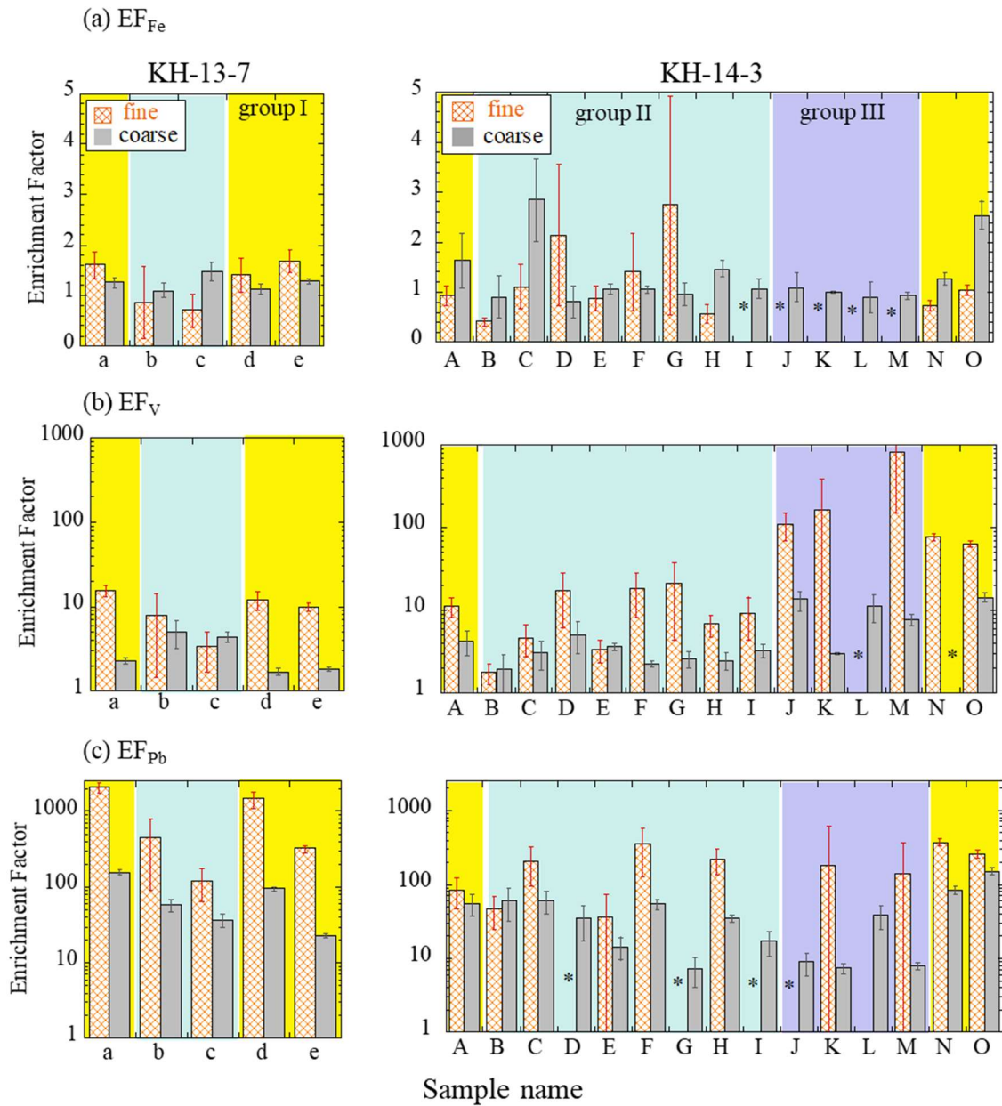
Figure 4. Enrichment factors of (a) Fe, (b) V, and (c) Pb. Errors were calculated from ICP-MS error and blank subtraction errors. Yellow, blue, and purple areas indicate group I (air masses from the Asian continent), II (air masses from the central and eastern Pacific), and III (air masses from the northern North Pacific), respectively. *Not available due to insufficient sample amount.
