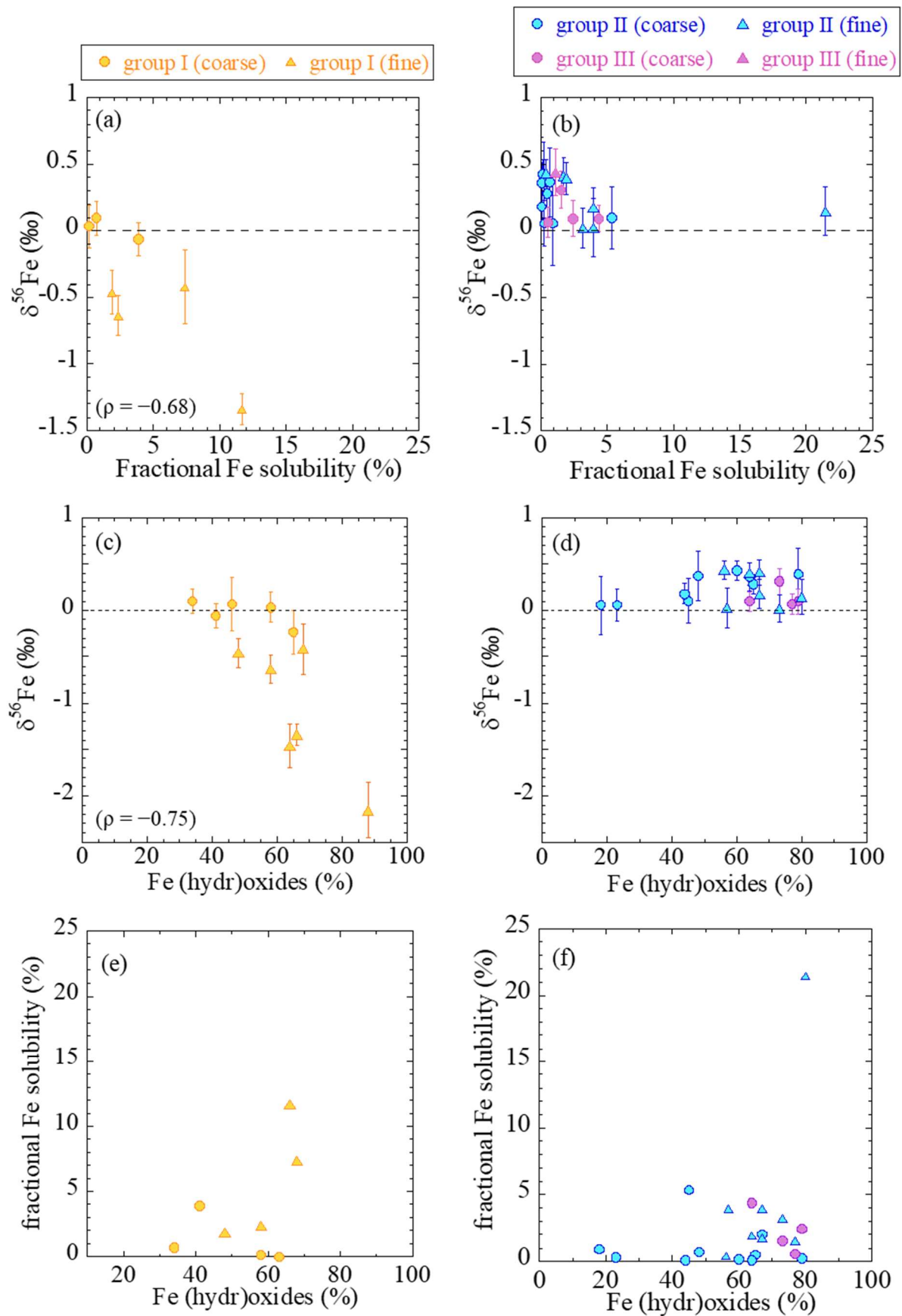
Figure 8. The relationships between (a,b) the fractional Fe solubility and \delta^{56}\text{Fe} ; (c, d) the fraction of Fe (hydr)oxides and \delta^{56}\text{Fe} ; and (e, f) the fraction of Fe (hydr)oxides and the fractional Fe solubility. \rho is the Spearman Rank Order correlation coefficient ( p < 0.05 ). *Only for fine particles. Yellow, group I; blue, group II; purple, group III.
