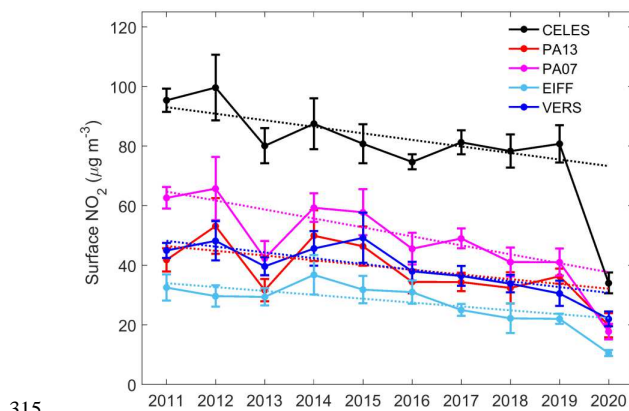
Figure 7: Similar to Figure 6 but with surface NO 2 concentration for different in situ sensors of AIRPARIF network (see Table 1).
