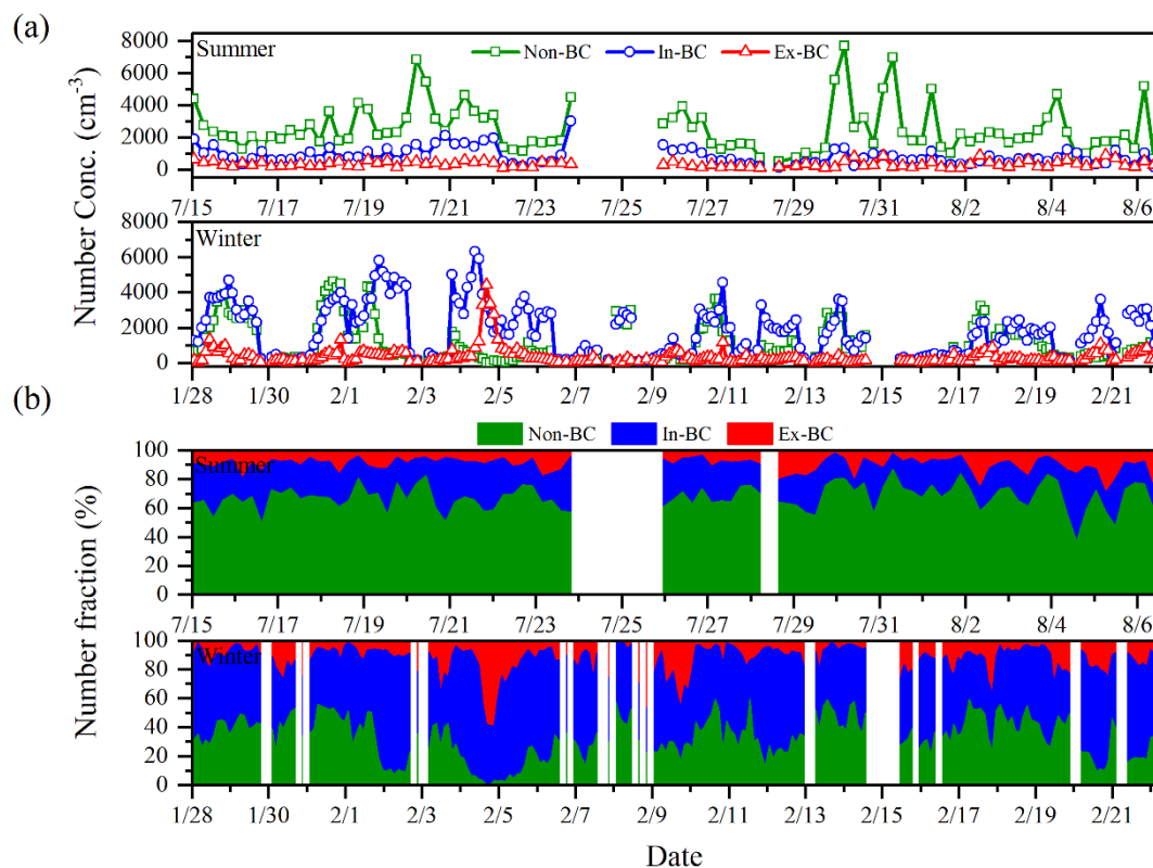
350 Figure 9. Summer (top) and winter (bottom) time series of (a) number concentrations and (b) number fractions of Non-BC (in green), In-BC (in blue), and Ex-BC (in red) of 150-nm particles.
