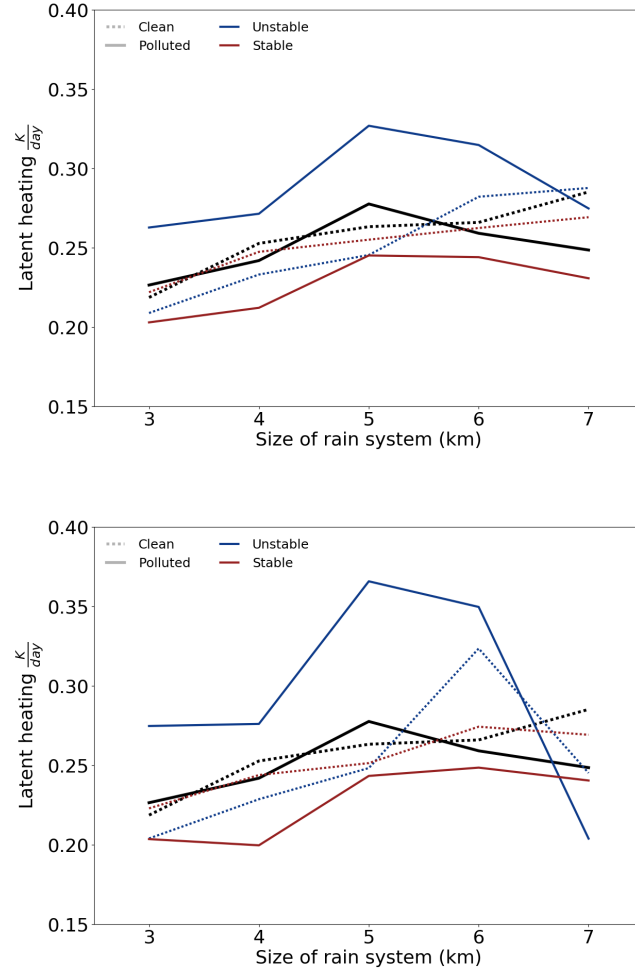
Figure 2. The mean amount of latent heating released due to precipitation formation rate in the geometrical center of the rain system as a function of rain system size for all (top) and dry (bottom) warm clouds with an extent of 15 km. Black is for all stabilities, blue is for unstable environments, red is for stable environments; dashed represents pristine and solid represents polluted surroundings.
