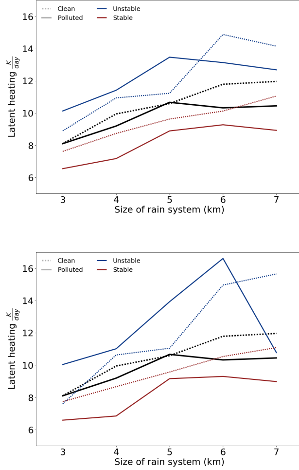
Figure 3. The maximum rate latent heat release due to precipitation within the cloud as a function of rain system size for all (top) and dry (bottom) warm clouds with an extent of 15 km. Black is for all stabilities, blue is for unstable environments, red is for stable environments; dashed represents pristine and solid represents polluted surroundings.
