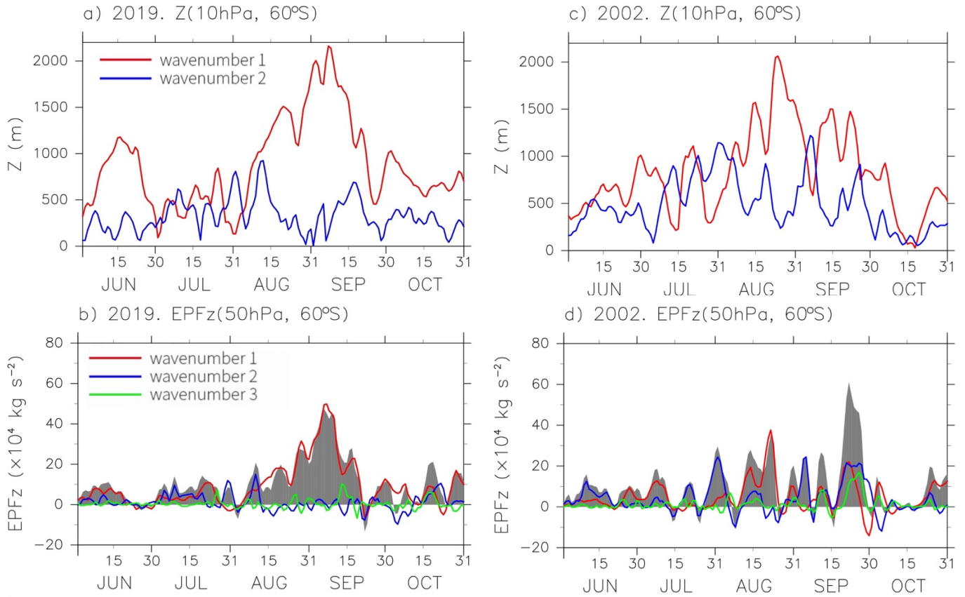
4 Figure 4. Time series of planetary waves amplitudes [m] at 10 hPa and 60°S (a,c) and the vertical component of the E-P flux 5 [ \times 10^4 \text{ kg s}^{-2} ] at 60°S and 50 hPa (b,d) from 1 June to 31 October for 2019 (left) and 2002 (right). The red, blue, and green 6 lines denote the zonal wavenumbers 1, 2, and 3, respectively. In the bottom panels, grey shadings show the vertical component 7 of the E-P flux of all wavenumbers.
