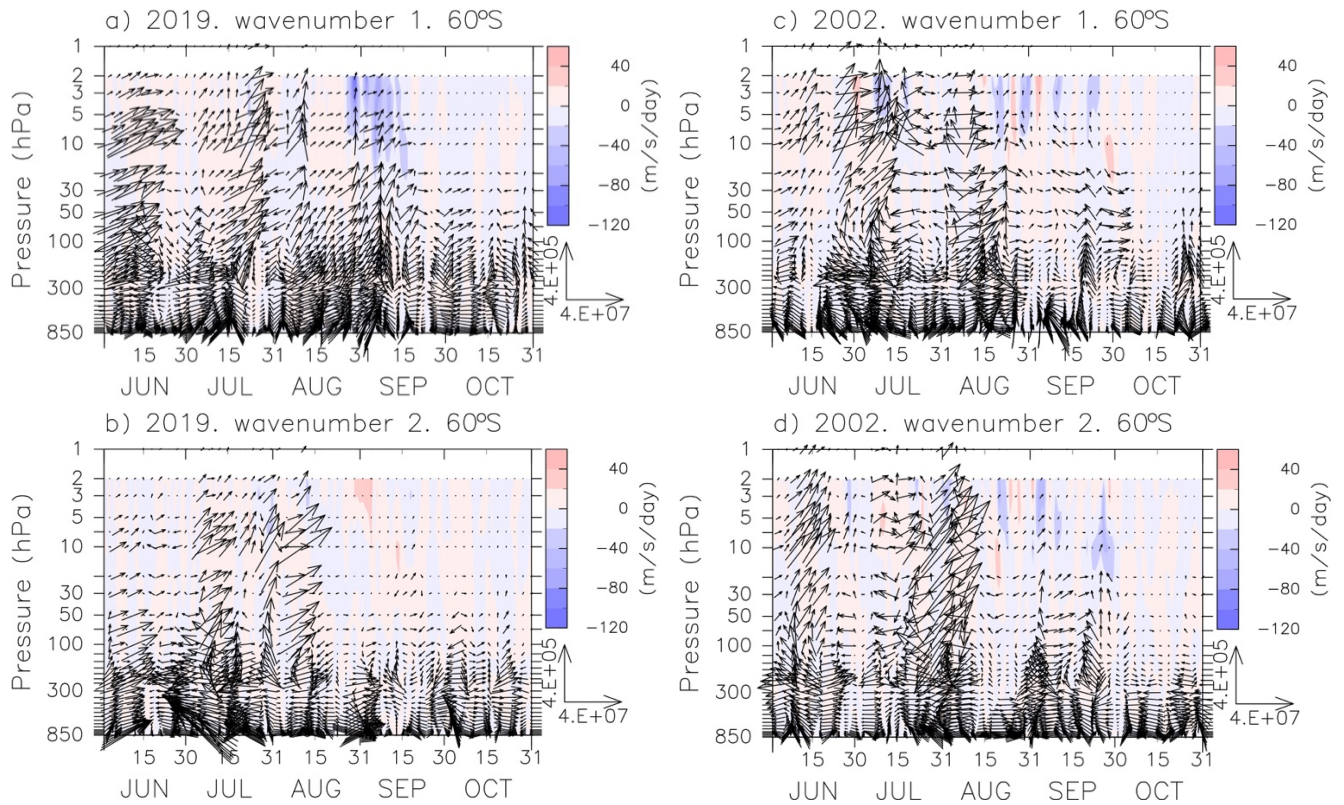
2 Figure 6. Time–height cross-sections of the E-P flux [ \text{kg s}^{-2} ] (vectors) at 60°S for zonal wavenumber 1 (a, c) and 2 (b, d) and 3 the wave driving due to its divergence [ \text{m s}^{-1} \text{day}^{-1} ] (colour shading) from 1 June to 31 October in 2019 (left) and 2002 (right). 4 E-P flux vectors pointing to the right direction corresponds to the poleward. The blue (red) shading denotes the zonal wind 5 deceleration (acceleration).
