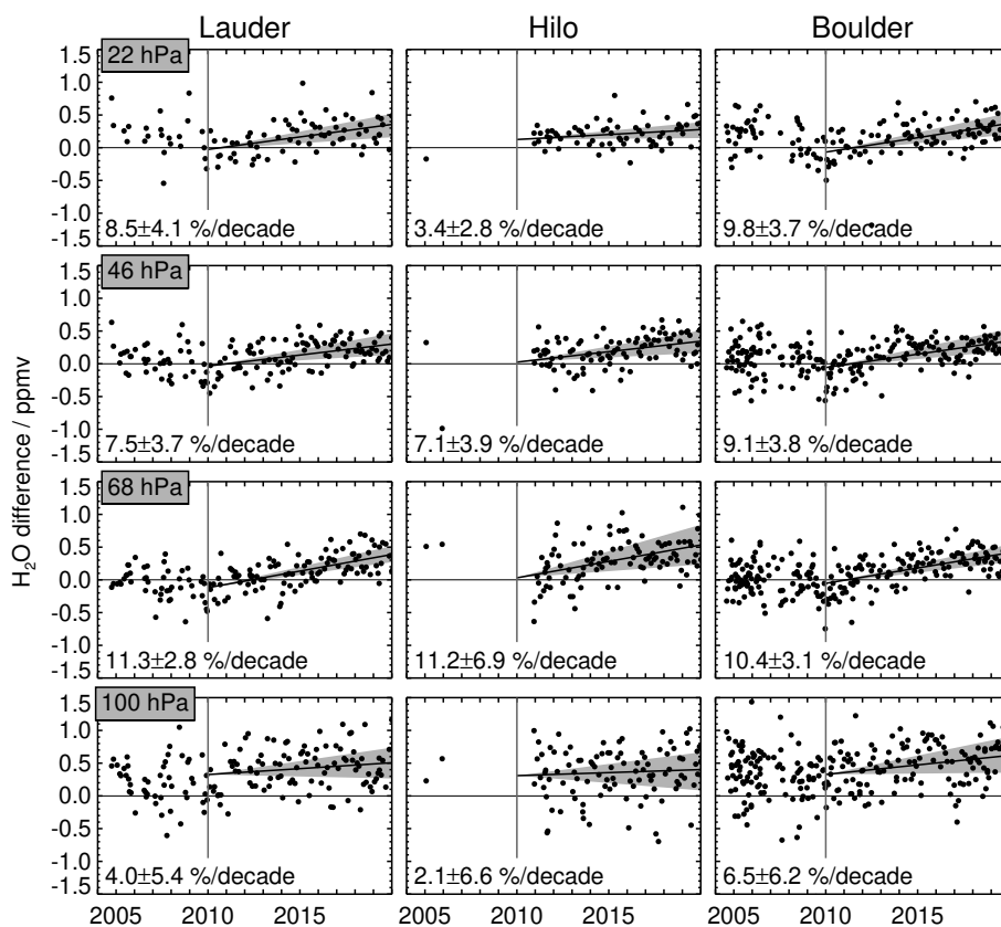
Figure 1. Timeseries of differences between MLS v4 and coincident frost point sonde measurements made from Lauder (45°S, 170°E, left), Hilo (20°N, 155°W, center) and Boulder (40°N, 105°W, right) at selected pressure levels (rows). Coincidence criteria are, as for Hurst et al. (2016), \pm 2^\circ latitude, \pm 8^\circ longitude, and \pm 18 hours. Positive differences imply that MLS measures greater humidity than the in situ observation. Black lines show a linear fit to the post-2010 differences. Grey shading shows the 95% confidence interval for the slope (from a block-bootstrap resampling of year-long blocks of the fit residuals). Fitted drift rates are quoted in each panel, with uncertainties corresponding to the 2\sigma spread of the bootstrap results. Comparisons at the intermediate vertical levels (not shown) indicate similar behavior.
