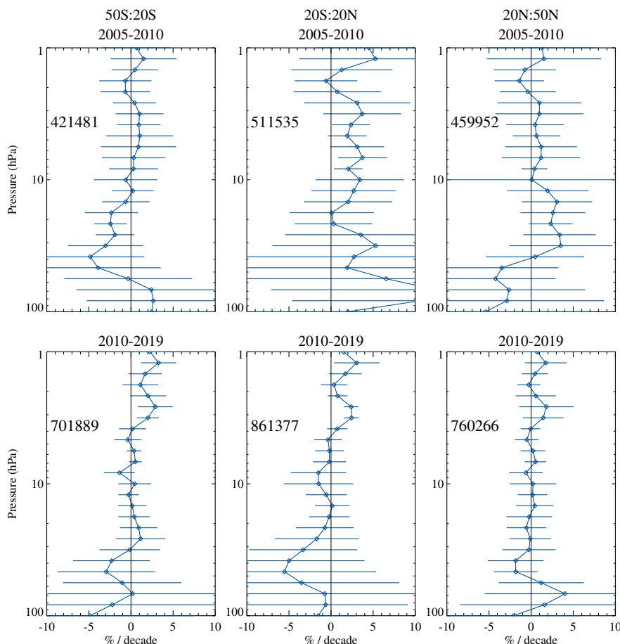
Figure 3. As Figure 2 but comparing MLS v4 to SABER version 2.07.
