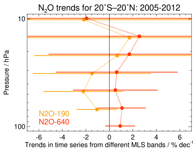
Figure 9. 2005–2012 trend seen in MLS 190- and 640-GHz tropical (20°S–20°N) N 2 O. Error bars are 2 \sigma intervals estimated from block bootstrapping.
