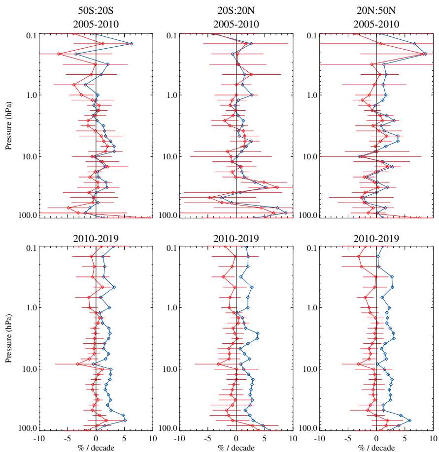
Figure 14. Drifts between MLS (v5, red, and v4, blue) and ACE-FTS version 4.1 observations. Coincidence criteria (and v4 results) are as for Figure 2, with error bars on v4 omitted here for clarity.
