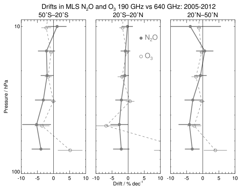
Figure 8. Drifts between MLS 190- and 640-GHz N 2 O products from 2005–2012 over three latitude bins. Also shown (dashed line) is the corresponding drift seen between MLS 190- and 640-GHz ozone. Error bars are 2 \sigma intervals estimated from block bootstrapping, as described in the text.
