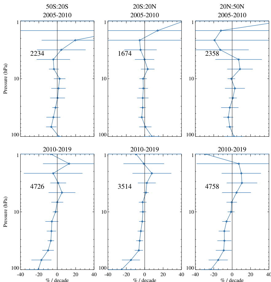
Figure 10. As Figure 2, but comparing the MLS 190-GHz \text{N}_2\text{O} product with the \text{N}_2\text{O} measurements from ACE-FTS.
