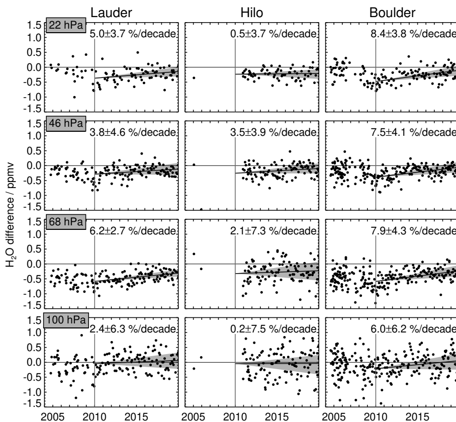
Figure 15. As for Figure 1, but comparing MLS v5 observations to frost point measurements.
