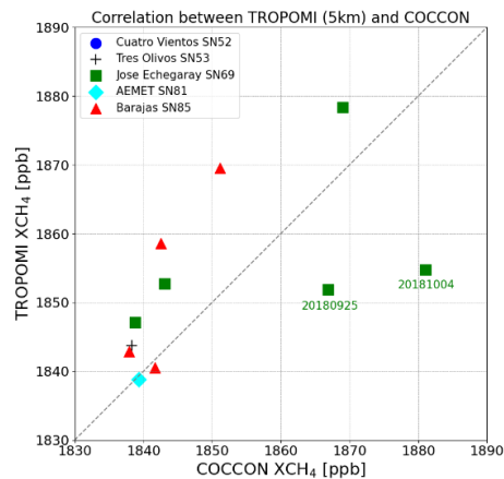
200 Figure 3: Correlation plot between TROPOMI observations collected within 5 km radius around each COCCON station and coincident COCCON measurements (30 minutes before and after the TROPOMI overpass) at five stations in 2018.
