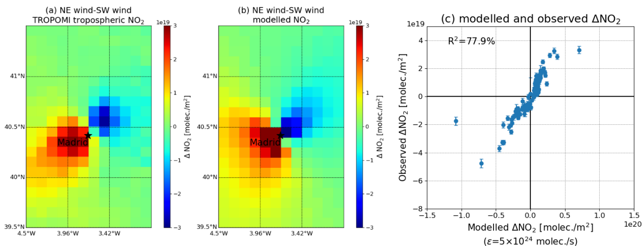
Figure 6: Wind-assigned anomalies derived from (a) TROPOMI tropospheric \text{NO}_2 column, (b) our simple plume model ( \epsilon = 5 \times 10^{24} \text{ molec s}^{-1} ) over Madrid in NE - SW direction on a 0.1^\circ \times 0.135^\circ latitude/longitude grid during 2018 – 2020, and (c) shows the correlation plot between observed \Delta\text{NO}_2 and modelled \Delta\text{NO}_2 ( \epsilon = 5 \times 10^{24} \text{ molec s}^{-1} ) during 2018-2019.
