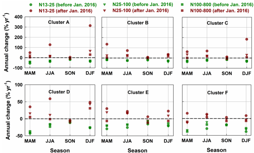
5 Figure 9: Seasonal variations in the trends of PNCs in three modes for the two contrasting periods (before vs. after January 2016) for each cluster. The annual change is calculated by Theil-Sen regression, and the calculation can refer to the above section of “2.3 Trend analysis methods”. MAM, JJA, SON and DJF are spring, summer, fall and winter, respectively.
