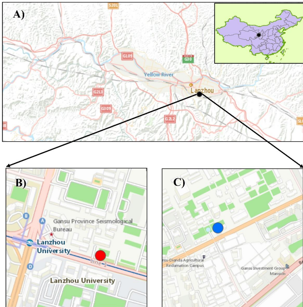
Figure 1: Map of A) Lanzhou City, B) the sampling site (red dot) and C) reference station that measured PM 2.5 and O 3 (blue dot). The map is a pure reproduction of Google Maps where our own contribution is rather small, and we only added a few marks for our study locations.
