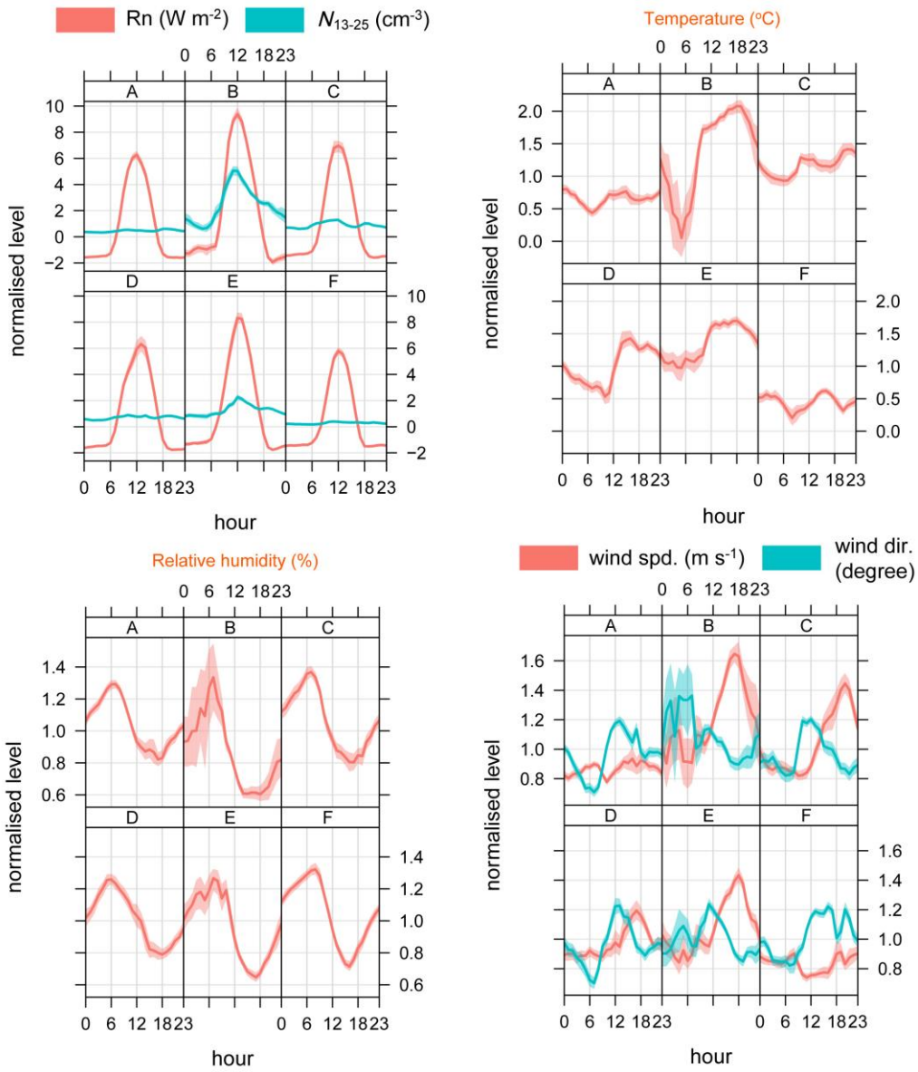
Figure 12: Normalized diurnal variations of net radiation (Rn), N_{13-25} , temperature, relative humidity, and wind speed and direction for each cluster during the campaign. The shading shows the estimated 95% confidence intervals.
