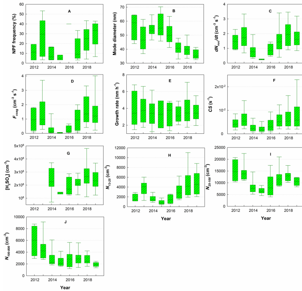
Figure 11: Inter-annual statistics of the trends of NPF frequency, mode diameter, formation ( dN_{nuc}/dt , F_{coag} ) and growth rates, CS and \text{H}_2\text{SO}_4 proxy and number concentrations in the three bins ( N_{13-25} , N_{25-100} , N_{100-800} ) during the campaign. The lines inside the box denotes the median slope, the two whiskers and the top and bottom of the box denote the 5th, 95th, 75th and 25th percentiles.
