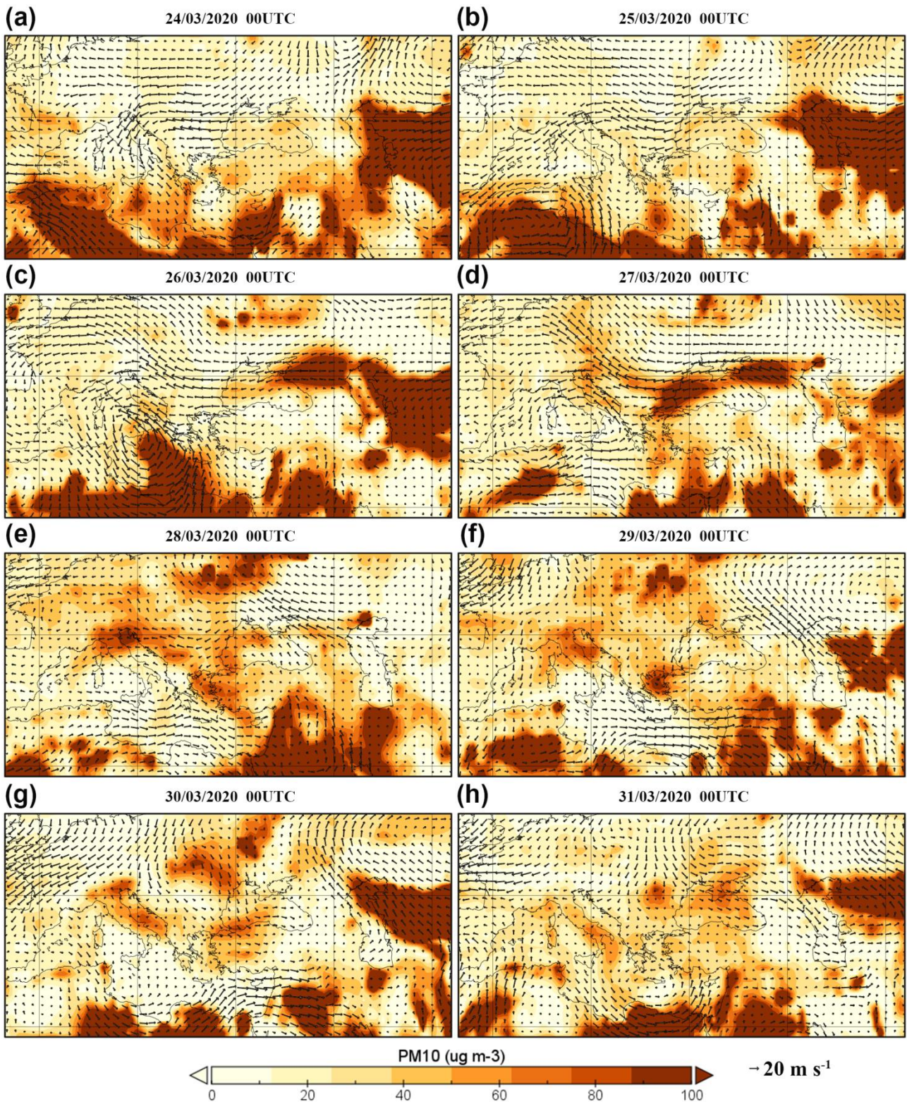
365 Figure 2. PM10 (in \mu\text{g m}^{-3} ) maps (colors) and horizontal surface wind (arrows) relative to each day in the period 24-31 March at 00 UTC (a-h). The maps were created with Panoply starting from ERA5 reanalysis. Letters from a) to h) are referred to the days from 24 to 31 March 2020.
