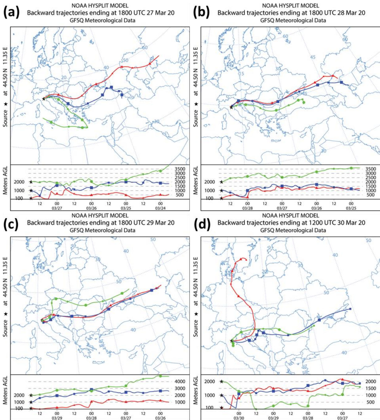
440 | Figure 23. Back-trajectories (96-h backwards) ending at Bologna on a) 27 March 18:00 UTC; b) 28 March 445 | 18:00 UTC; c) 29 March 18:00 UTC; d) 30 March 12:00 UTC
