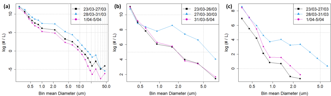
Figure 56. Particle size distributions for the OPCs: a) LOAC (Bologna); b) FAI (Trieste); c) GRIMM (Mt. Cimone). Abscissa values are in \mu\text{m} , ordinate values in \log(\# \text{ L}^{-1}) . Abscissa axis is on logarithmic scale
