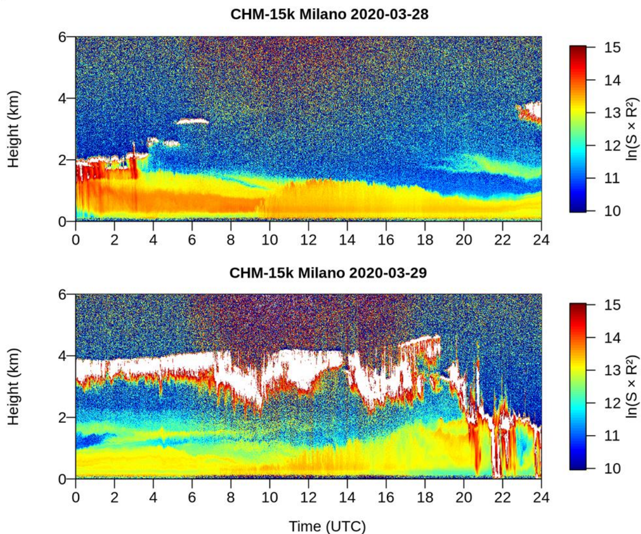
610 Figure 89. Vertical profiling from the automated LIDAR ceilometer located in Milan on 28 and 29 March 2020.
