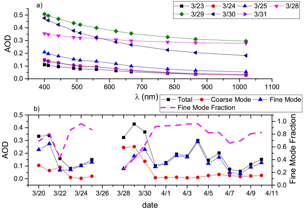
Figure 78. a) Aerosol Optical Depth (AOD) at different wavelengths and for different days of March 2020 detected at the AERONET site of Venice; b) time series of the total, coarse, and fine mode AOD, and fine mode fraction observed in March-April 2020 at the AERONET site of Venice.
