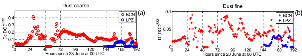
190 Figure 4. Hourly dust optical depth calculated from the extinction profiles for (a) the coarse mode and (b) the fine mode obtained using the POLIPHON algorithm in BCN (red) and LPZ (blue).
