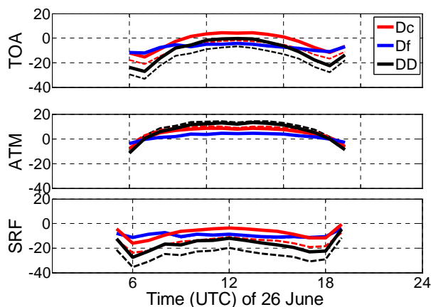
350 Figure 10. Diurnal cycle on 26 June in BCN of the dust net radiative effect ( DRE_{NET} ) for Dc, Df and DD (bottom) at SRF, (middle) in the atmosphere, and (top) at TOA. For Dc (red) and DD (black) the diurnal cycle of DRE_{SW} is also reported by dash lines. Df DRE_{SW} is not represented since it would overlap with Df DRE_{NET} .
