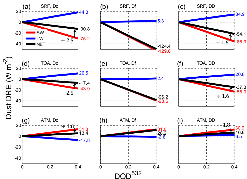
405 Figure 12. Linear fitting of the dust direct radiative effect (SW, LW and net) as a function of DOD^{532} at SRF for (a) Dc, (b) Df and (c) DD; at TOA for (d) Dc, (e) Df and (f) DD; and in the atmosphere for (g) Dc, (h) Df and (i) DD, in BCN (23-30 June). Corresponding DREff values (slope of the linear fitting of DRE vs. DOD^{532} ) are included next to the right axis. DREff units are W m^{-2} \tau^{-1} . In Dc and DD plots the arrows and number indicate the SW / NET ratio. The legend in plot (a) applies to all plots.
