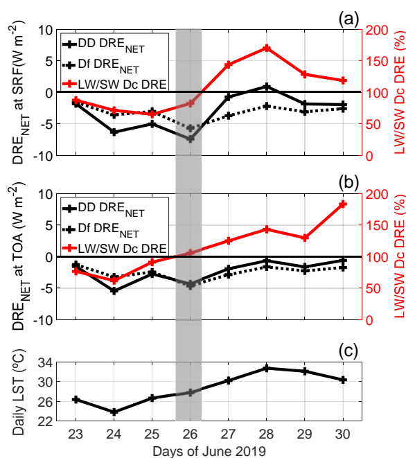
485 Figure 13. (a) Daily Df and DD DRE_{NET} (left axis) and Daily Dc LW/SW DRE ratio (right axis) at SRF; (b) Daily Df and DD DRE_{NET} (left axis) and Daily Dc LW/SW DRE ratio (right axis) at TOA; (c) Daily mean LST. Site: BCN; Time period: 23-30 June. The shaded area represents the period during which both SRF and TOA Dc LW/SW DRE ratio cross the 100 % threshold.
