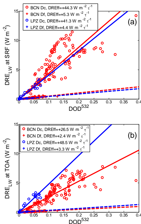
390 Figure 11. Dust longwave direct radiative effect ( DRE_{LW} ) at (a) SRF and (b) TOA as a function of DOD^{532} , as shown separately for Dc (circles) and Df (crosses) at BCN (23-30 June) and LPZ (29-30 June). Corresponding DREff values (slope of the linear fitting of DRE_{LW} vs. DOD^{532} ) are included in the legend (solid and dashed lines, respectively, for Dc and Df particles).
