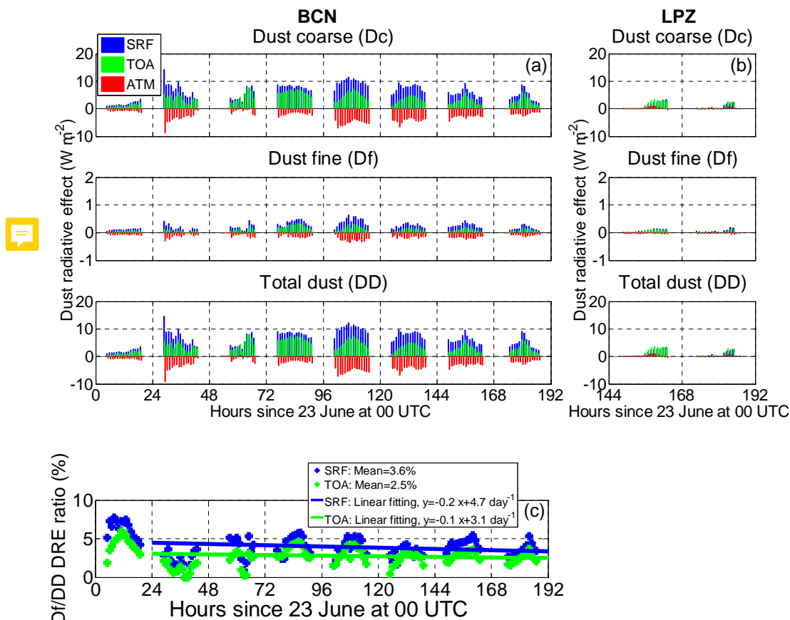
315 Figure 7. Longwave instantaneous dust direct radiative effect ( DRE_{LW} ) at SRF, TOA and in the atmosphere (ATM) in (a) BCN and (b) LPZ. (c) Df/DD DRE ratio of the instantaneous DRE_{LW} at the SRF and TOA in BCN; the mean values and best linear fits have been calculated between 24 and 30 June. The absolute decrease of Df/DD DRE_{LW} ratio at the SRF (TOA) is -0.2 ( -0.1 ) \% \text{ day}^{-1} .
