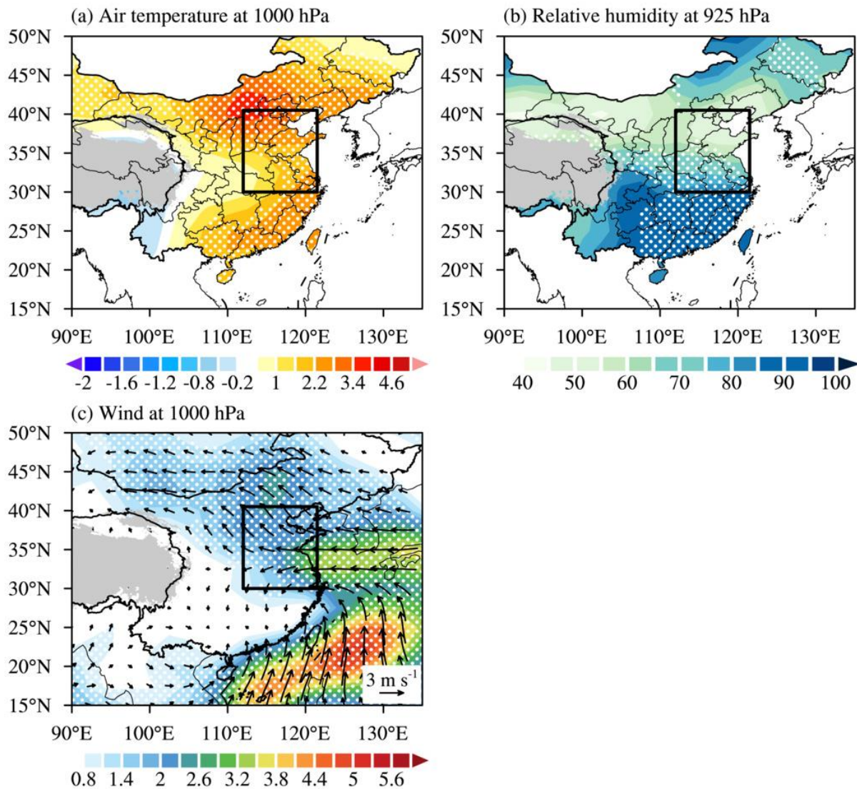
450 Figure 3: Composite (a) anomalous air temperature at 1000 hPa, (b) absolute values of relative humidity at 925 hPa, and (c) anomalous wind (arrows) and wind speed (shading, m s -1 ) at 1000 hPa for the 13 SR-NH events. The white dotted region indicates areas at the 99% confidence level based on the two-tailed Student's t test. The black box indicates the NCP (30°-40.5° N, 112°-121.5° E) and the gray area is the Tibetan Plateau.
