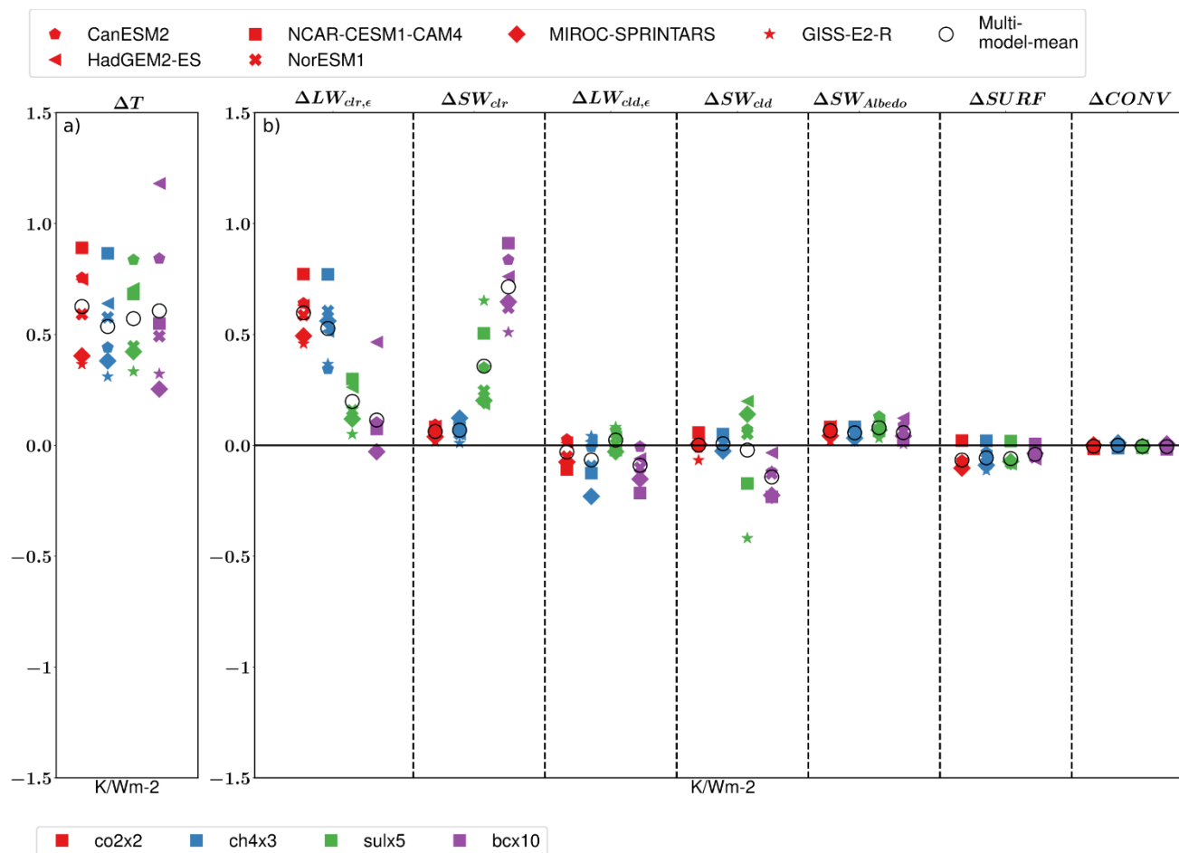
295 Figure 3. The global mean effective temperature response and its decomposition, calculated as the difference between means over the last 50 years of the perturbed and the baseline experiments. (a) The effective temperature response (absolute temperature response divided by ERF_{sst} ) for the six models shown with different symbols, and four different radiative forcers shown with different colors. (b) The decomposition of the effective temperature response to different energetic components. Individual panels in (b) describe (from the left) the contributions to total effective temperature response due to the change in longwave clear-sky emissivity ( \Delta LW_{clr,\epsilon} ), change in TOA shortwave radiation ( \Delta SW_{clr} ), change in longwave cloud emissivity ( \Delta LW_{cld,\epsilon} ), net ocean surface heat flux ( \Delta SURF ), and change in atmospheric energy transport ( \Delta CONV ). 300
