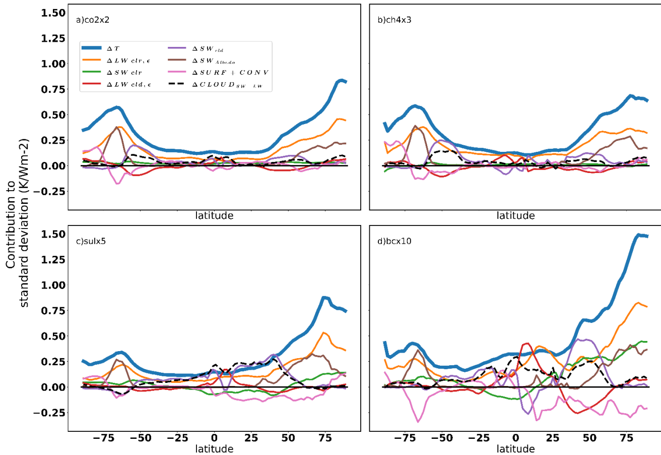
455 Figure 7. Zonal mean of the total standard deviation of the effective temperature response (thick blue line), and the contributions of the different energy balance terms to it (thin lines, see the legend in (a)). Panel (a) shows co2x2, panel (b) ch4x3, panel (c) sulx5 and panel (d) bcx10 experiment.
