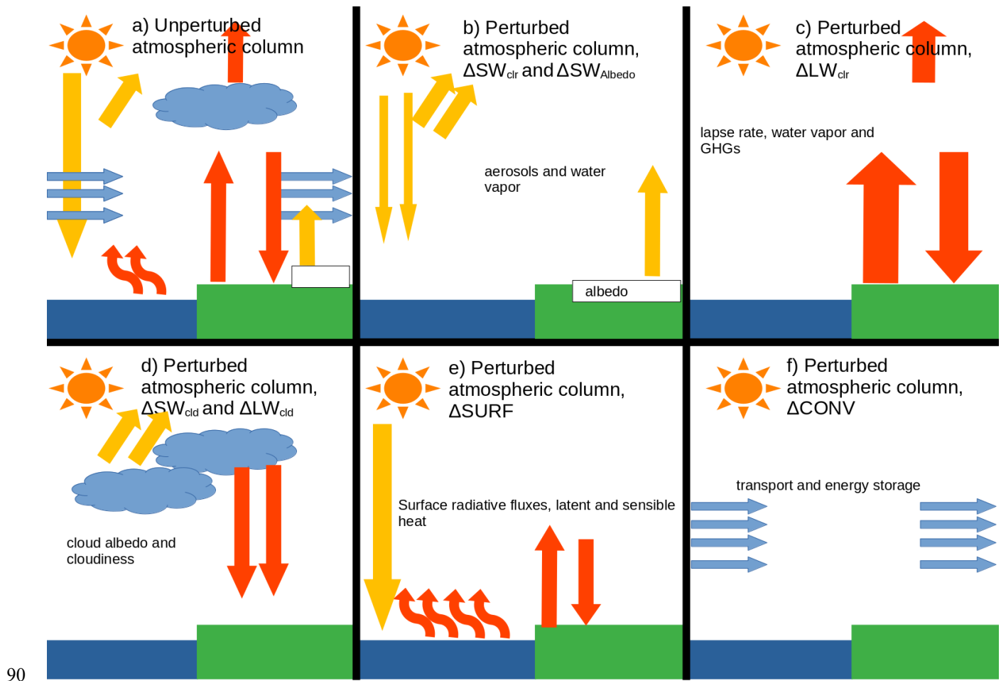
90 Figure 1. Illustration of the local atmospheric energy budget in a single atmospheric column from the surface to the top-of-model atmosphere (TOA). We attribute the change in local surface temperature to changes in different terms of the local energy budget. (a) Unperturbed conditions, where red arrows indicate longwave (thermal) radiation, yellow arrows indicate shortwave (solar) radiation, blue arrows indicate horizontal incoming and outgoing energy, and curly red arrows indicate latent and sensible heat. Under perturbed conditions, we decompose the change in the energy budget to (b) the change in TOA solar radiation due to changes in surface albedo, and to the change in shortwave clear-sky flux (separately). The change in shortwave clear-sky flux is mainly caused by changes in aerosol concentrations or changes in atmospheric water vapor; (c) the change in longwave TOA flux, which is mainly caused by changes in atmospheric water vapor concentrations, atmospheric thermal structure (lapse rate) or greenhouse gas concentrations; (d) changes in longwave and shortwave TOA fluxes, separately, due to changes in cloudiness and cloud microphysics, (e) the combined change in surface energy balance, including the change in the net shortwave and longwave energy flux into the surface and changes in latent and sensible heat fluxes; (f) the combined change in horizontal energy transport and internal energy of the atmospheric column, calculated from the convergence of energy. 95 100
