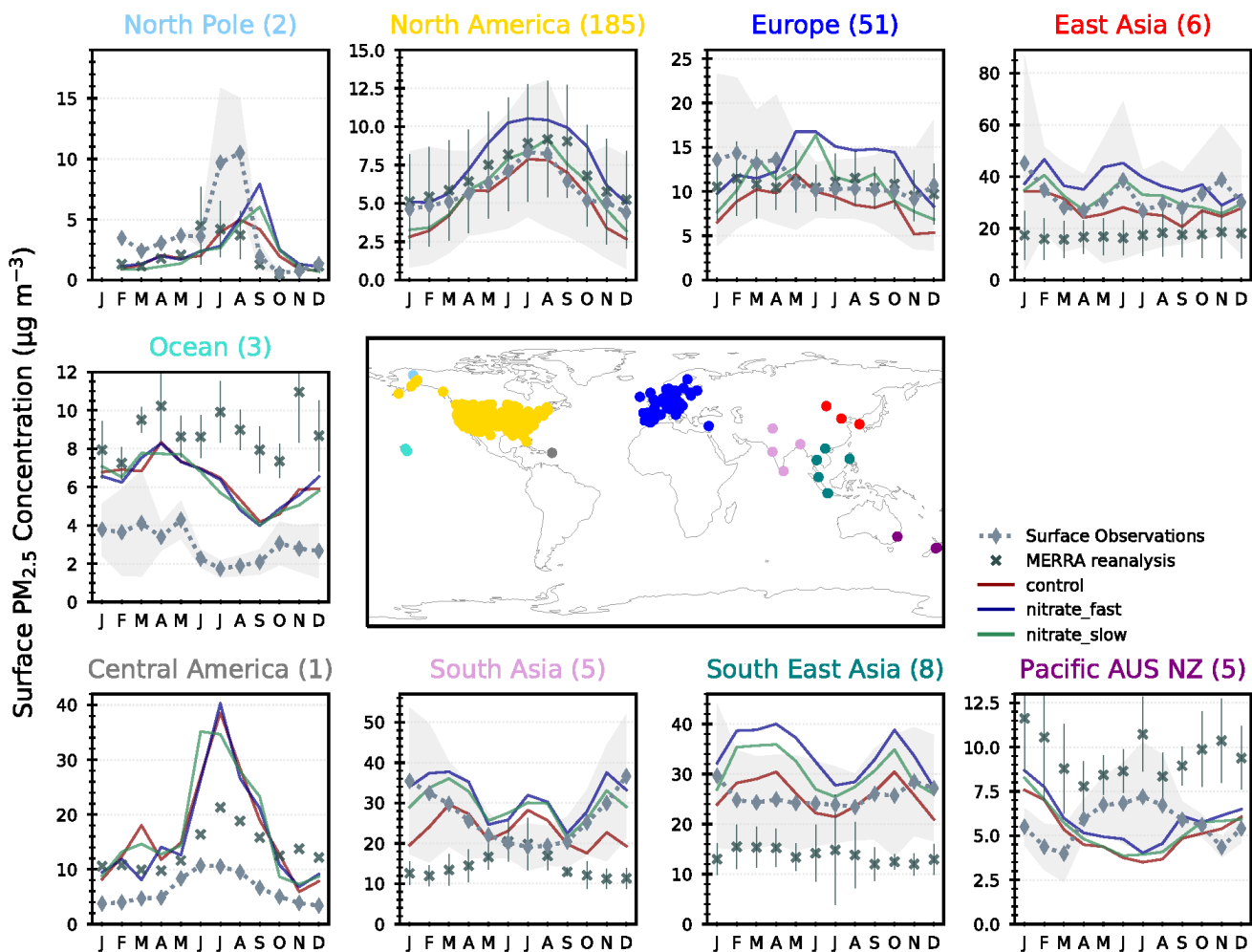
Figure 8: Regional and monthly-mean surface PM_{2.5} concentrations in the UM simulations (CNTL=red, FAST=blue, and SLOW=green lines), and from MERRA reanalyses and GASSP surface observations
