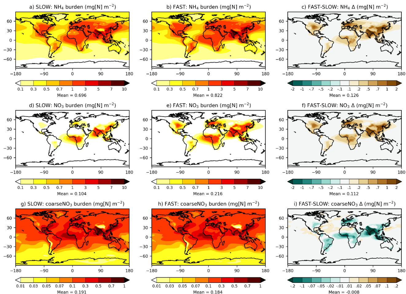
465 Figure 1: Annual-mean NH 4 , NO 3 , and coarseNO 3 burdens from the SLOW and FAST simulations
