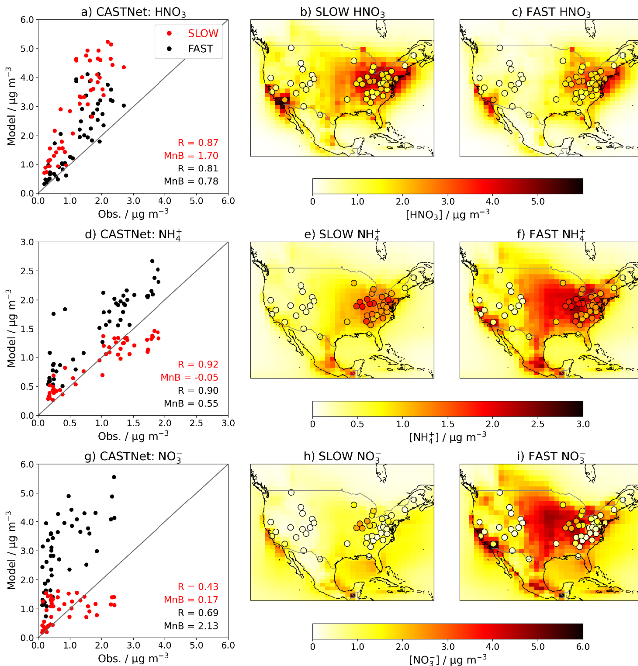
Figure 5: Annual-mean \text{HNO}_3 , \text{NH}_4 and total- \text{NO}_3 near-surface concentrations in the FAST and SLOW simulations over North America compared to CASTNet observations averaged over 1994-2013. In (b), (c), (e), (f), (h) and (i), coloured contours show simulated concentrations while overlaid filled circles represent CASTNet observations. In (a), (d), and (g), 'R' is the Pearson's correlation coefficient and 'MnB' is the mean bias between simulated and observed concentrations
