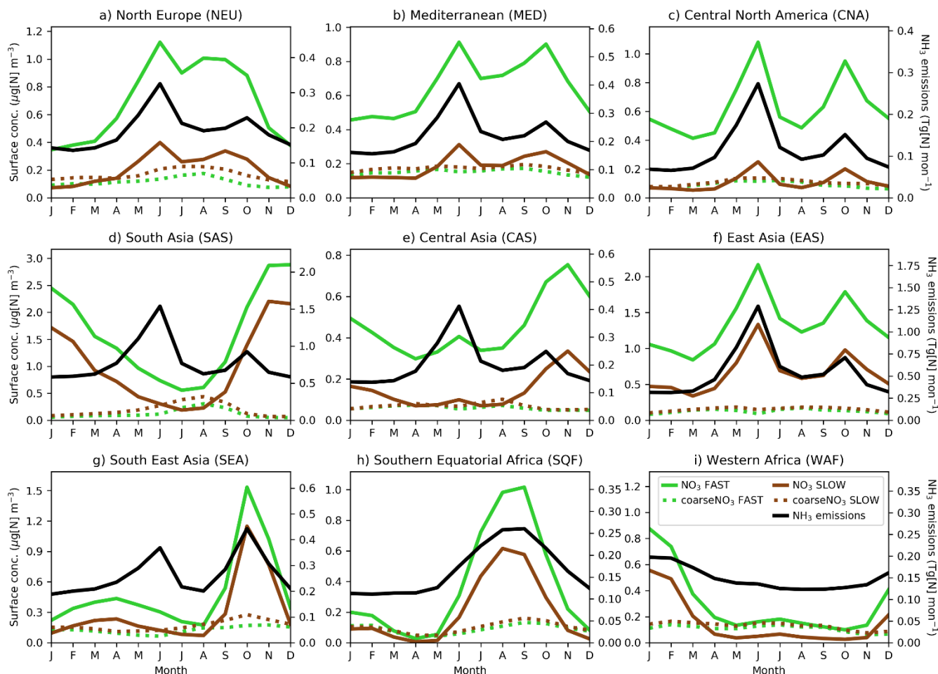
Figure 4: Regional and monthly-mean NO 3 (solid line) and coarseNO 3 (dashed line) near-surface concentrations and NH 3 emissions (solid black line) time-series for the SLOW (brown) and FAST (green) simulations for 9 'Giorgi regions' [Giorgi, 2006] (land-only) representing areas with high NO 3 concentrations.
