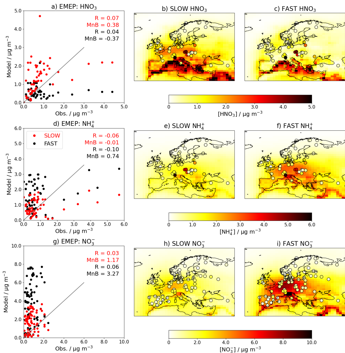
575 Figure 6: Annual-mean \text{HNO}_3 , \text{NH}_4 and total- \text{NO}_3 near-surface concentrations for the FAST and SLOW simulations over Europe compared to EMEP observations averaged over 1994-2013 where available. In (b), (c), (e), (f), (h) and (i), coloured contours show simulated concentrations while overlaid filled circles represent EMEP observations. In (a), (d), and (g), ‘R’ is the Pearson’s correlation coefficient and ‘MnB’ is the mean bias between simulated and observed concentrations
