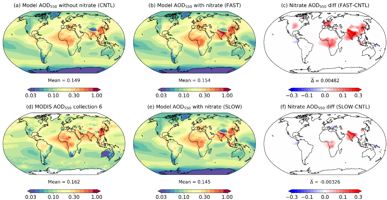
Figure 9: Annual-mean and column-integrated 550nm aerosol optical depth (AOD 550 ) in the CNTL, FAST, and SLOW simulations and from MODIS collection 6 satellite observations. (c) and (f) show the difference between the FAST and CNTL, and SLOW and CNTL, simulations respectively
