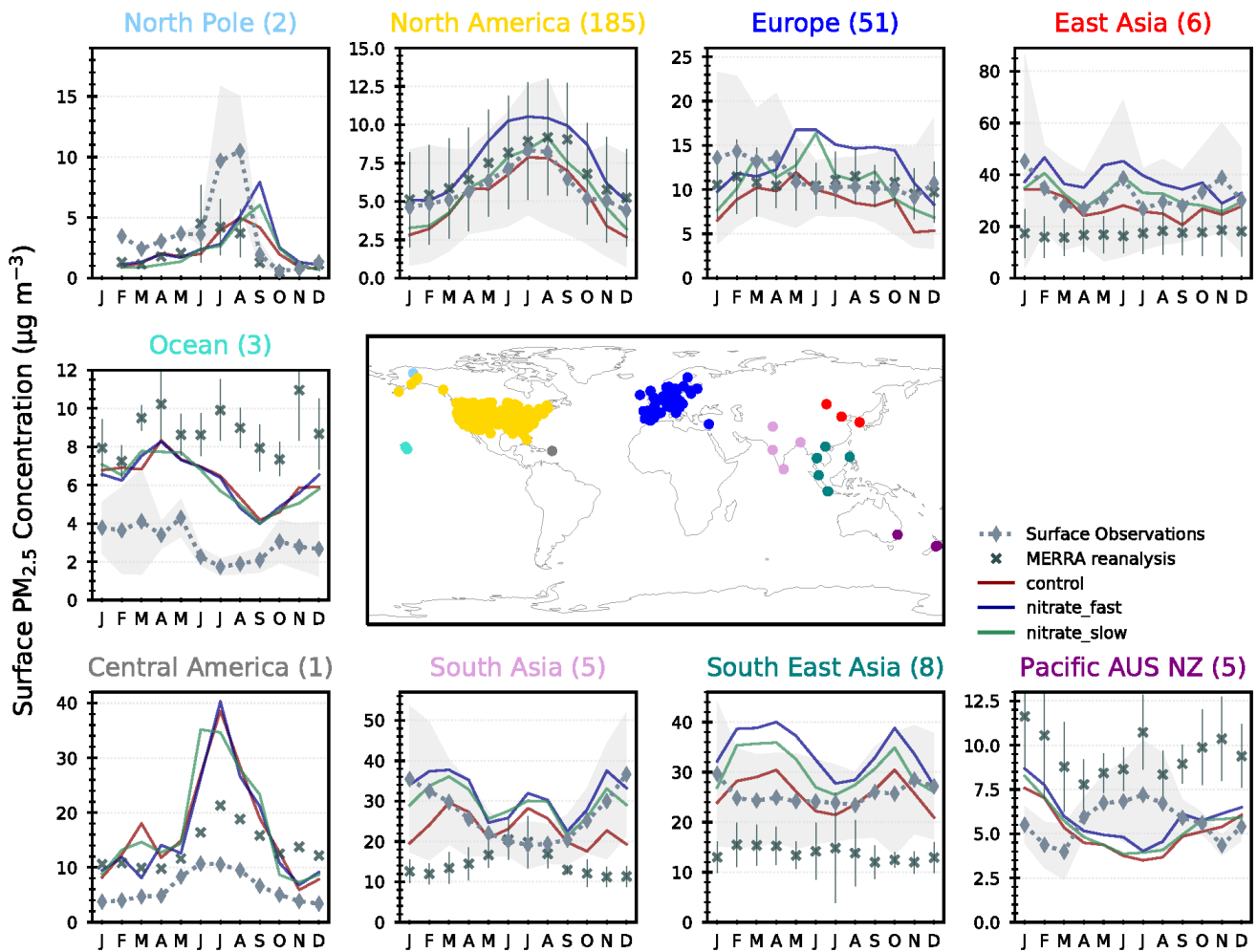
620 Figure 8: Regional and monthly-mean surface PM 2.5 concentrations in the UM simulations (CNTL=red, FAST=blue, and SLOW=green lines), and from MERRA reanalyses and GASSP surface observations
