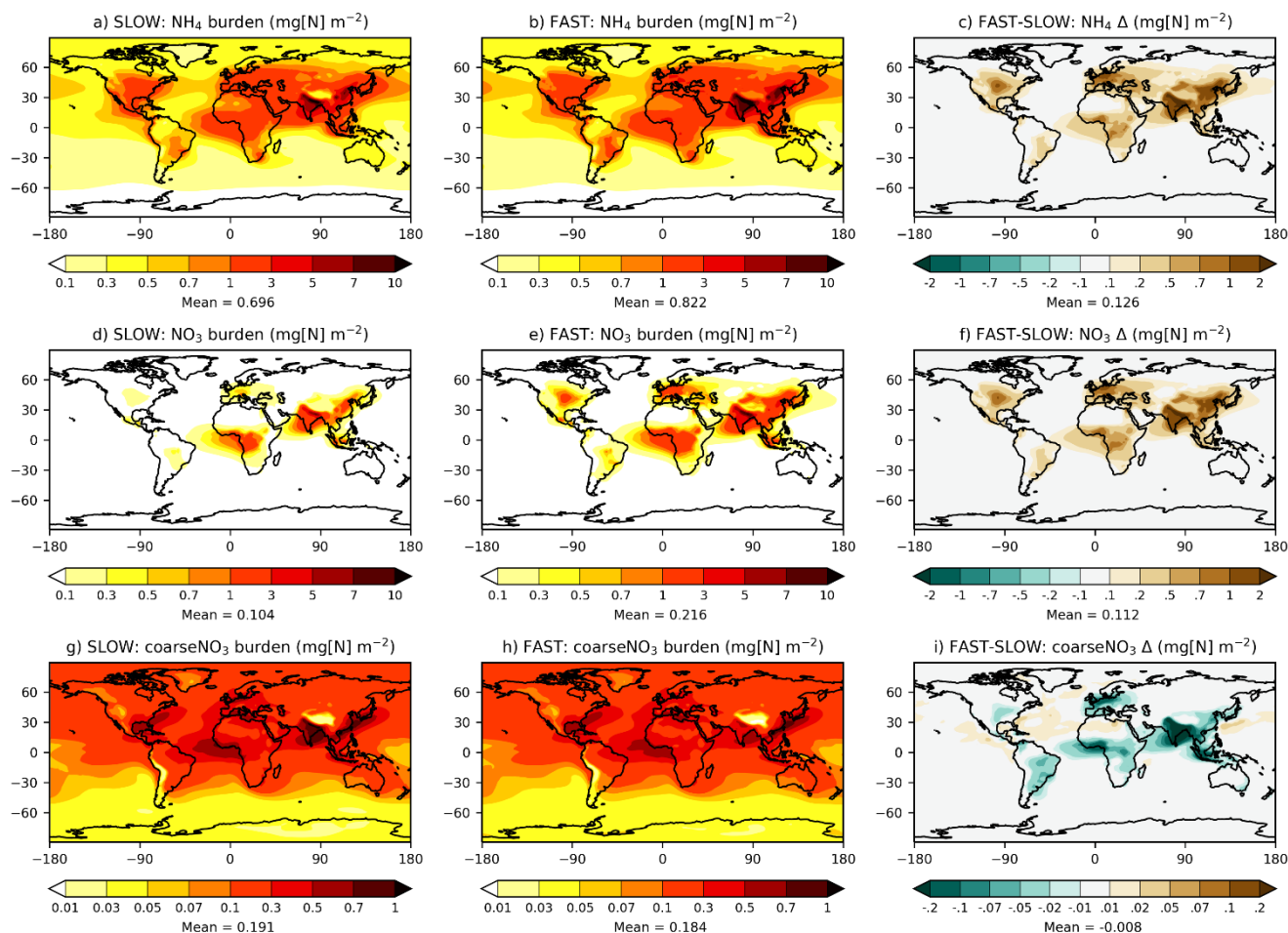
Figure 1: Annual-mean NH 4 , NO 3 , and coarseNO 3 burdens from the SLOW and FAST simulations
