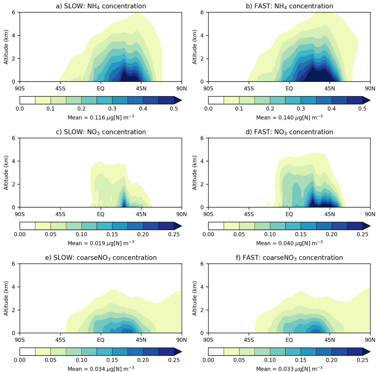
Figure 3: Annual and zonal-mean \text{NH}_4 , \text{NO}_3 , and coarse \text{NO}_3 concentrations vs altitude from the SLOW and FAST simulations
