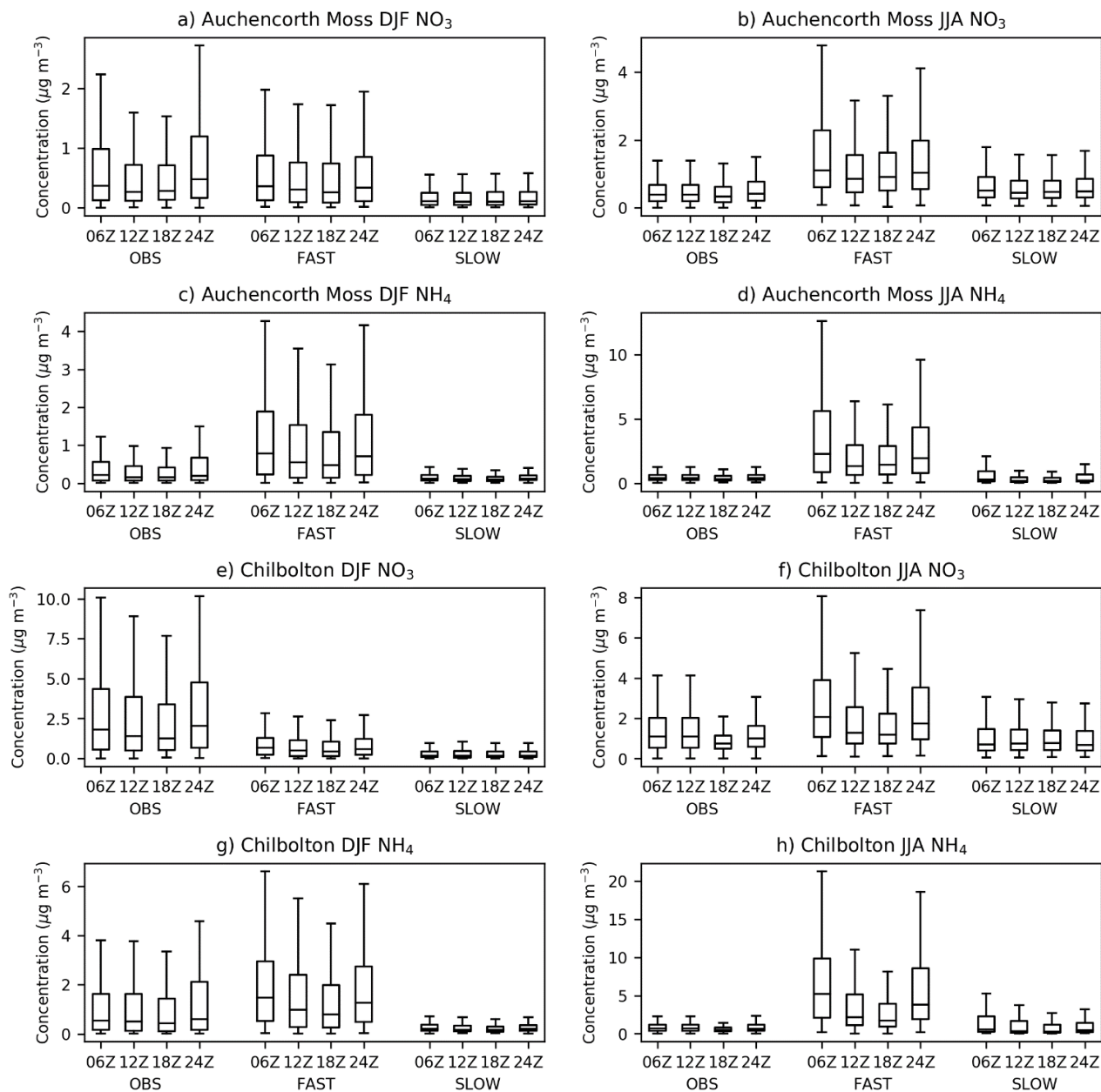
615 Figure 7: December-February (DJF) and June-August (JJA) diurnal cycles of near-surface total-NO 3 and NH 4 aerosol concentrations in the FAST and SLOW simulations interpolated to two European Monitoring and Evaluation Programme (EMEP) supersites in the UK – Auchencorth Moss [55.79216°N, -3.2429°E] and Chilbolton [51.149617°N, -1.438228°E], alongside 6 hourly observations from 2014-2018 for Auchencorth Moss and 2016-2020 for Chilbolton
