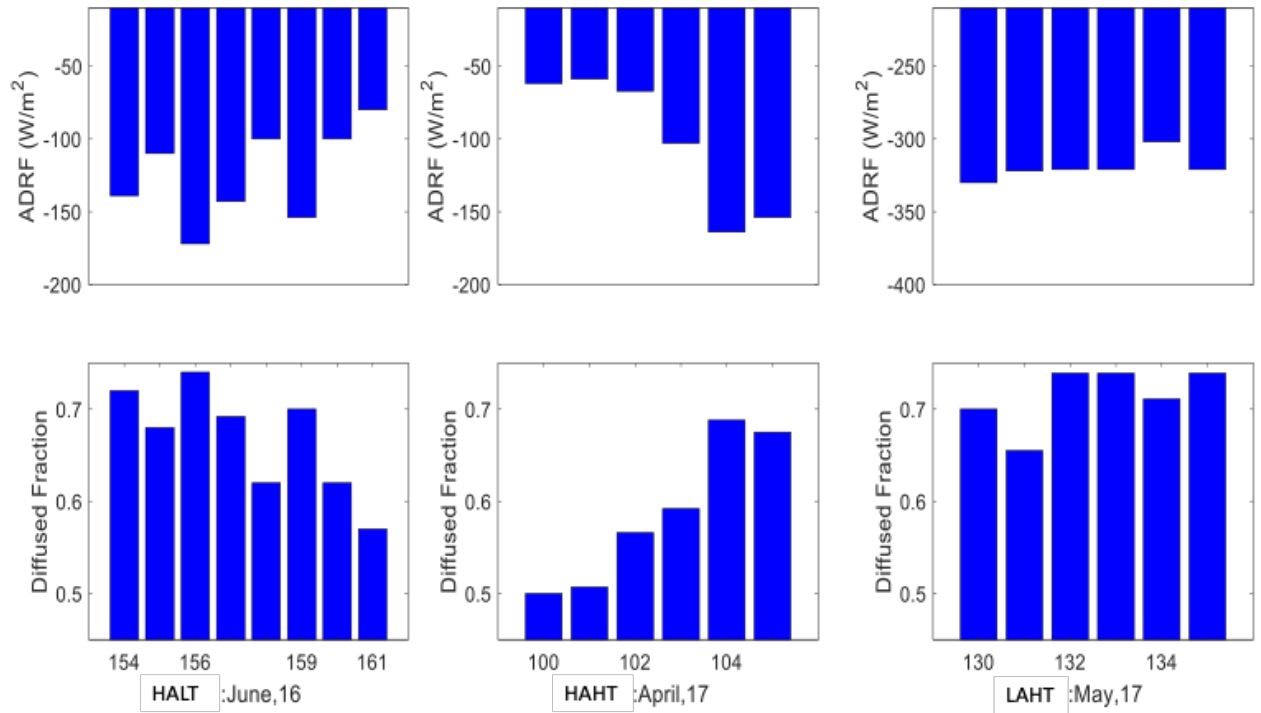
Figure S1: SBDART estimated broadband shortwave Aerosol direct radiative forcing (ADRF) at surface and fraction of diffuse radiation ( diffuse_{frac} ) at surface during (A and D) HALT episode, (B and E) HAHT episode and (C and F) LAHT episode. X-axis shows the Julian day of the year.
