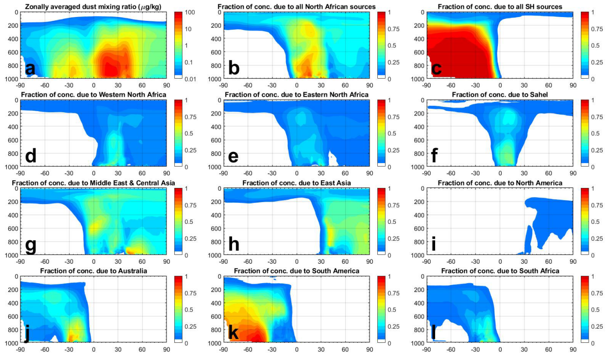
Figure 6. Attribution of the zonally averaged and annually averaged PM 20 dust concentration to the world's main source regions. Panel (a) shows the zonally averaged dust mixing ratio (dust concentration normalized by air density) as a function of latitude (horizontal axis) and pressure in hPa (vertical axis). Panels (b)-(l) show the partition of the dust concentration per source region, with panel ordering identical to Figure 5. The seasonally resolved attribution of the zonally averaged dust concentration is shown in Figures S20-S23.
