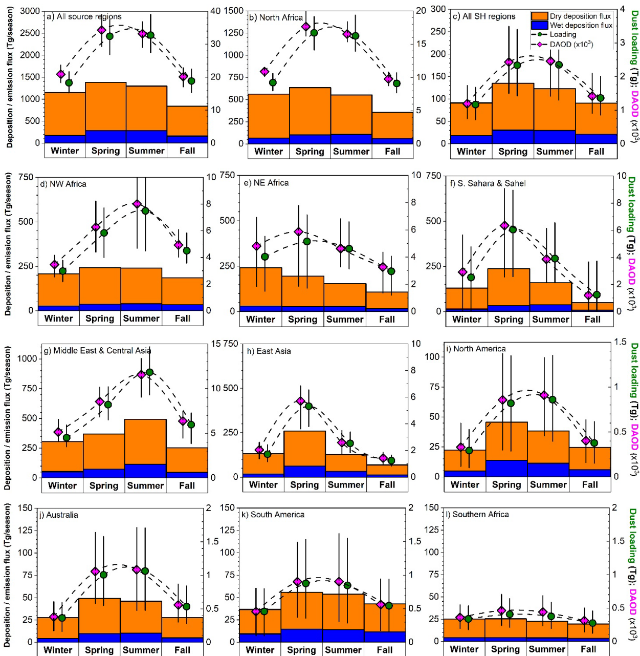
Figure 4. Seasonal contributions of each source region to the global dust cycle. Shown are the seasonal cycles of the wet deposition flux (blue bars and left axis), dry deposition flux (brown bars and left axis), dust loading (green circles and right axis), and DAOD (magenta diamonds and right axis) generated by (a) all source regions, (b) all North African source regions, (c) all Southern Hemisphere source regions, and (d-l) each of the nine individual source regions. The sum of the seasonal wet and dry deposition fluxes is approximately equal (within a few percent) to the seasonal dust emission flux generated by each source region. Results for loading and DAOD are slightly offset horizontally for clarity. Seasons refer to boreal seasons for global results (panel (a)) and for local seasons for all other panels. Note that the
