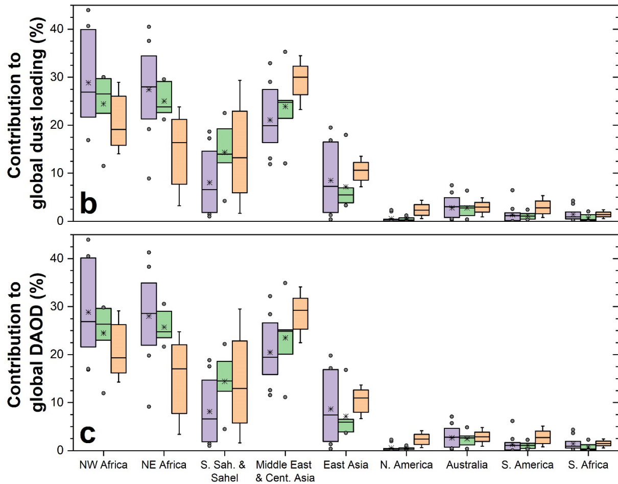
Figure 2. Fractional contribution of each source region to the global dust cycle. Shown are the fractional contributions to the annual global dust emission (and deposition) flux (a), the global dust loading (b), and the global DAOD (c) for the AeroCom ensemble (purple boxes; see Section 2.2) our model ensemble (green boxes) and for the inverse model (orange boxes). Box boundaries approximately denote the one standard error range (i.e., boxes contain 9 out of 13 AeroCom simulations, 4 out of 6 model ensemble members, and the 68% probability range for the inverse model's results), gray circles denote the individual simulation results outside of this range, whiskers denote the 95% confidence interval for the inverse model results, horizontal solid lines denote the median result, and stars denote the mean result. Results for each season are shown in Figs. S1-S4.
