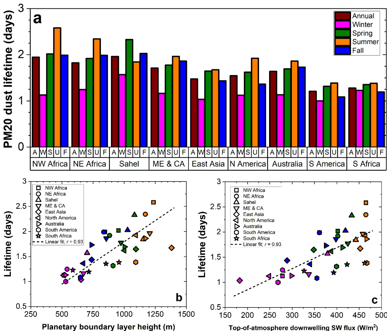
Figure 3. Seasonal variation of dust lifetime for the different source regions. (a) Mass-weighted lifetime of PM 20 dust for each source region on an annual basis (A; brown bars) and for each source region's local winter (W), spring (S), summer (U), and fall (F) seasons (magenta, green, orange, and blue bars). Variations in dust lifetime are largely explained by differences in downwelling SW flux (panel b) and planetary boundary layer (PBL) height (panel c). This indicates that the increased modeled dust lifetime in spring and summer is due to increased convection, which lofts dust to greater altitudes. Colors of symbols in panels b and c denote the season per the color scheme in panel a. The TOA downwelling SW flux was obtained from Wong and Chow (2001), the seasonally averaged PBL height was obtained from the GISS Model E2.1 simulation (Kelley et al., 2020), and the mass-weighted dust lifetimes were obtained from the ratio of the PM 20 dust loading with the deposition flux for each source region and season. Size-resolved annual and seasonal dust lifetimes of the individual model ensemble simulations used in the inverse model are shown in Figs. S5 – S9.
