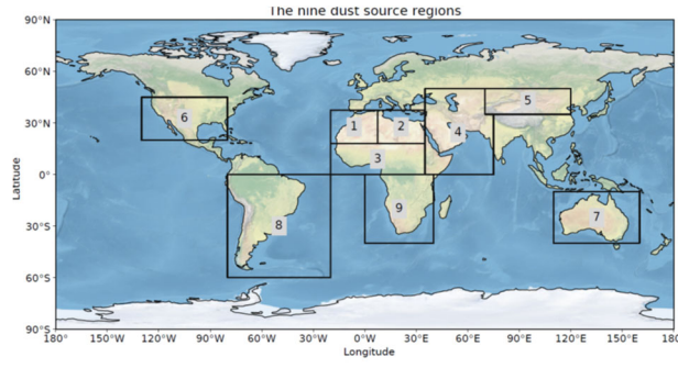
Figure 1. Coordinates of the nine main source regions used in this study. The nine source regions are: (1) western North Africa, (2) eastern North Africa, (3) Southern Sahara & Sahel, (4) Middle East & Central Asia (which includes the Horn of Africa), (5) East Asia, (6) North America, (7) Australia, (8) South America, and (9) Southern Africa. Exact coordinates for these regions are given in Kok et al. (2021). After Kok et al. (2021); made with Natural Earth.
