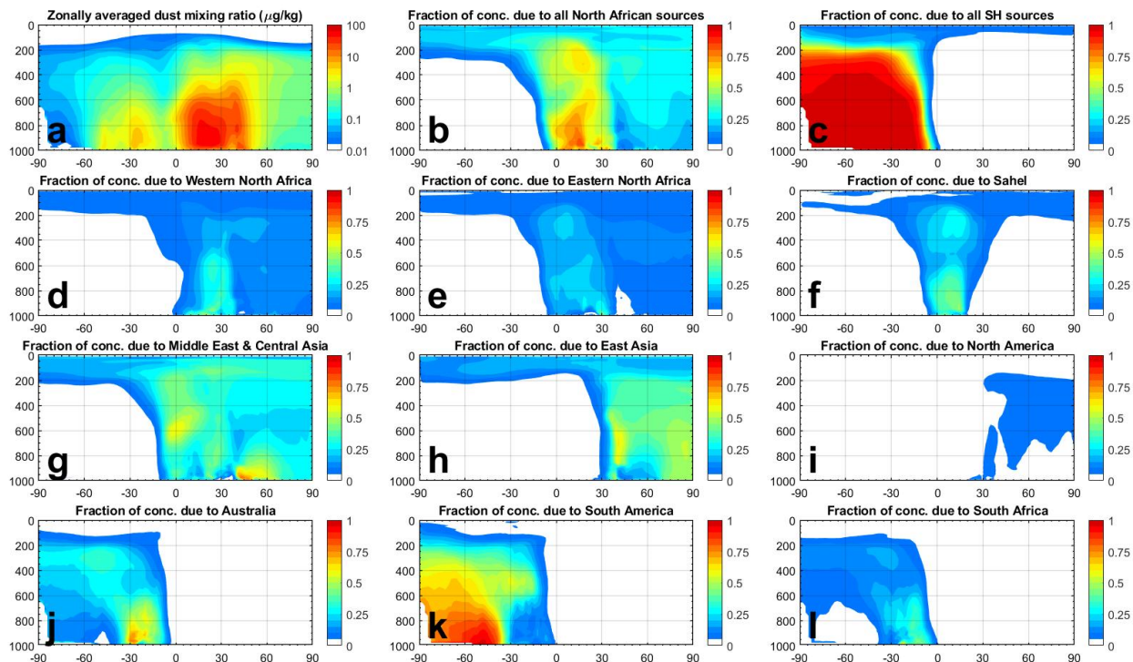
Figure 6. Attribution of the zonally averaged and annually averaged PM 2.5 dust concentration to the world's main source regions. Panel (a) shows the zonally averaged dust mixing ratio (dust concentration normalized by air density) as a function of latitude (horizontal axis) and pressure in hPa (vertical axis). Panels (b)-(l) show the partition of the dust concentration per source region, with panel ordering identical to Figure 5. The seasonally resolved attribution of the zonally averaged dust concentration is shown in Figures S20-S23.
