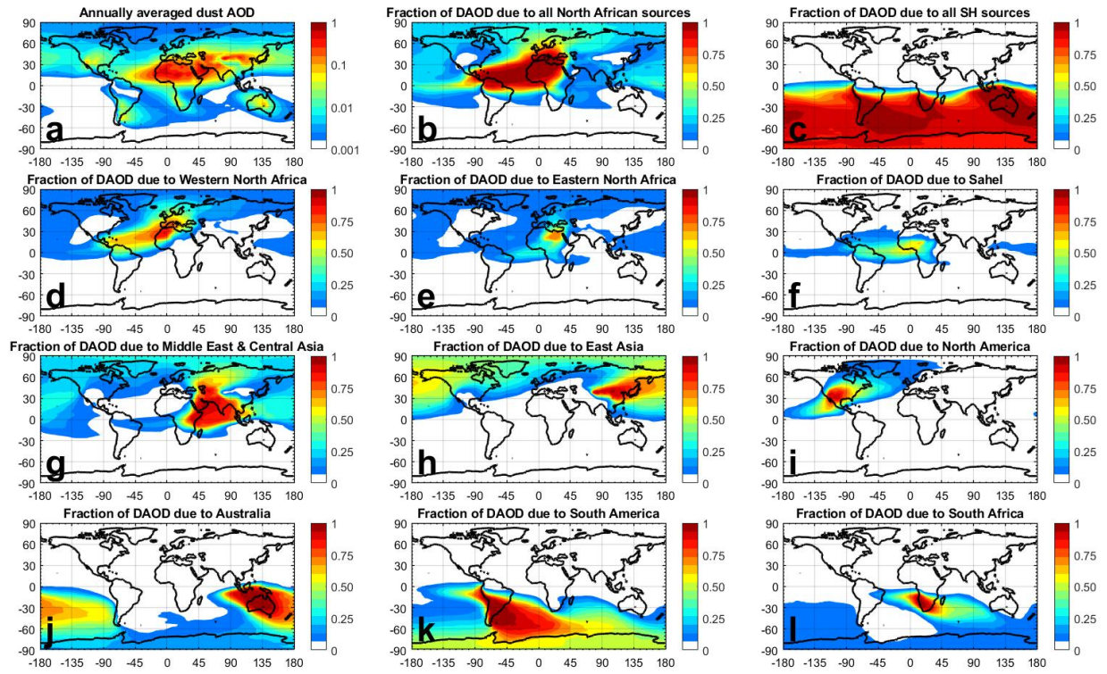
355 Figure 5. Attribution of the annually averaged DAOD to the world's main dust source regions. Shown first is (a) the annually averaged DAOD produced from all source regions combined, followed by the fraction of DAOD that is due to (b) all North African and (c) all Southern Hemisphere source regions. The fraction of DAOD due to each of the three North African source regions are shown in panels (d)-(f), and the fraction of DAOD due to the other three Northern Hemisphere source regions of Middle East & Central Asia, East Asia, and North America are shown in panels (g)-(i). Finally, the fraction of DAOD due to the three Southern Hemisphere source regions of Australia, South 360 America, and South Africa are shown in panels (j)-(l). Attributions of seasonal DAOD to the different source regions are shown in Figures S12-S15.
