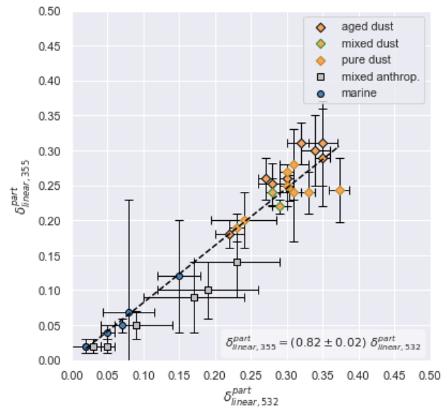
Figure 2. Scatter plot of \delta_{linear,355}^{part} versus \delta_{linear,532}^{part} for dust, marine and anthropogenic particles obtained from the literature (see Table 2).
