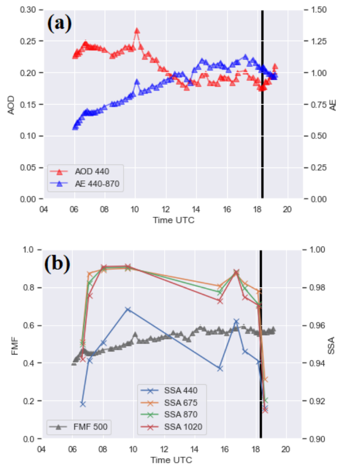
Figure 8. Sun-photometer data retrieved by AERONET at Évora on the 28th June 2019: (a) AOD 440 and AOD-AE 440-870 and (b) fine mode fraction at 500 nm (FMF 500 ) and multiwavelength SSA daily series. The black vertical line indicates the Aeolus overpass.
