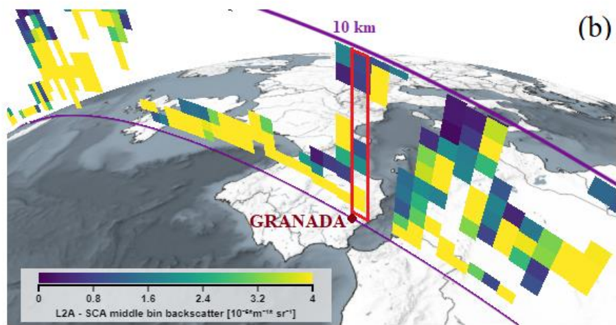
Figure 3. (a) Lidar range corrected signal measured at 1064 nm in Granada on the 5th September 2019. (b) Aeolus SCAMB backscatter retrievals along the considered orbit (6007) with the profile closest to the station marked in red (source: VirES for Aeolus, aeolus.services ). Quality flags are applied.
