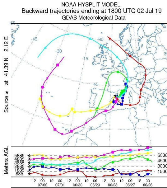
Figure 11. HYSPLIT model back trajectories for the air masses between 0.9 and 5.9 km agl (equivalent to 1 and 6 km asl) over Barcelona at 18:00 UTC on the 2nd July 2019.
