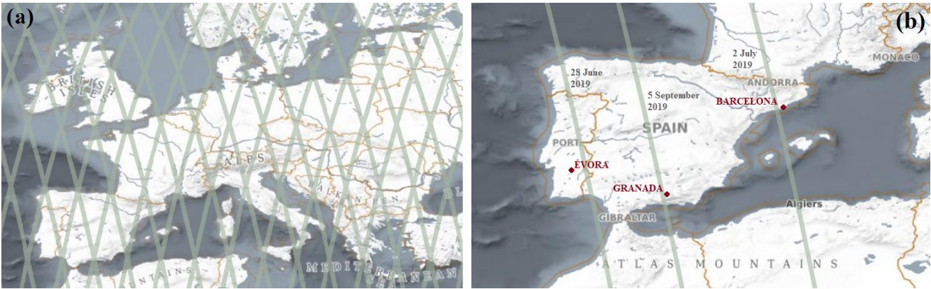
Figure 1. (a) Distribution of Aeolus overpasses over Europe during the considered period (B10, from July 2019 to December 2019 and from 20th April 2020 to 6th October 2020). (b) Location of the stations in Évora, Granada and Barcelona and the associated overpasses during the case studies analyzed in Section 4.2.. Source: ESA Aeolus online dissemination ( aeolus-ds.esa.int ).
