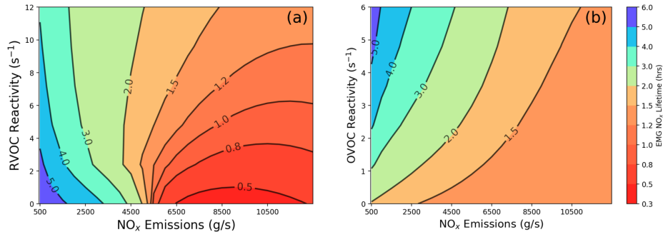
485 Figure 7 Same as Fig. 6 but showing the \text{NO}_x lifetime dependence on \text{NO}_x emissions versus the reactivities of (a) RVOC and (b) OVOC. We run the model at a constant wind speed of 5 m/s, and the \text{P}(\text{HO}_x) is set constant at 50 \times 10^6 molecules/ \text{cm}^3 .
