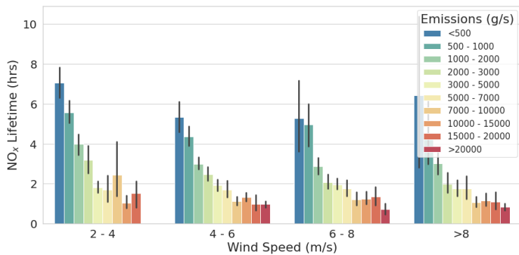
Figure 5 The mean and standard deviation of TROPOMI derived NO x lifetimes from fires at different emissions (colour) and wind speeds. Fire episodes with less than 2 m/s wind speed are not shown.
