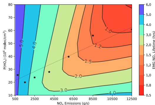
465 Figure 6 Isoleth showing the NO x lifetime dependence on NO x emissions versus P(HO x ). We run the PECANS 1-D model with varying NO x emissions and P(HO x ). The lifetime is estimated by fitting the modelled NO x concentration along the wind direction with the EMG function (Eq. (7) and (8)). We run the model at a constant wind speed of 5 m/s, and the VOC reactivity is set constant at 4.8 \text{ s}^{-1} for both groups (RVOC and OVOC). The black stars show the TROPOMI observed mean NO x emissions and lifetime at wind speed between 4 to 6 m/s, where the P(HO x ) value is estimated as the level that gives the closest NO x lifetime as observations at given NO x emissions. The dashed line represents the fitted regression line. 470
