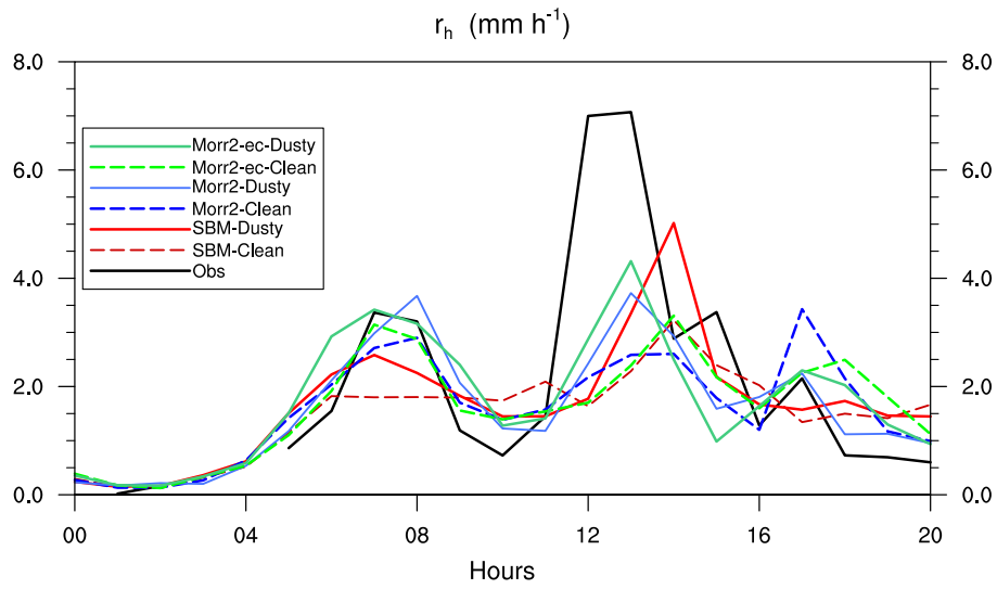
Figure S4. Hourly rainfall rates from IMERG observation (black line) and six numerical runs (colored lines) (LT 00:00–20:00, 2006-07-08), averaged among rainfall grids ( > 0 \text{ mm hr}^{-1} ) in the High-Pcp area.
