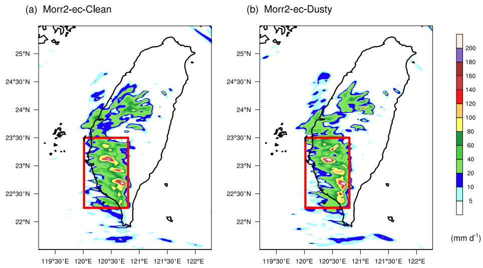
Figure S3. 24-hour accumulated precipitation (LT 2006-07-08) simulations from (a) Morr2-ec-Clean and (b) Morr2-ec-Dusty.
