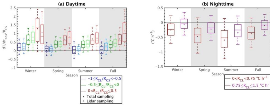
Figure 87: (a) \frac{\partial T_{2m}/\partial t_{obs}}{R_{CS}} daytime values for the four seasons for three R_{CL}/R_{CS} bins: -1.0 \leq \frac{R_{CL}}{R_{CS}} < -0.5 in blue, -0.5 \leq \frac{R_{CL}}{R_{CS}} < 0 in green and 0 < \frac{R_{CL}}{R_{CS}} \leq 0.5 in red. Dark-colors box plots with the mean represented as '*' correspond to cases when all meteorological variables are available at the same time (without considering lidar availability), whereas light-colors box plots with 'o' as their mean value represent the sample when both all meteorological variables and Lidar profiles are available simultaneously. (b) \partial T_{2m}/\partial t_{obs} nighttime values for two R_{CL} bins: 0^\circ \text{ h}^{-1} < R_{CL} < 0.75^\circ \text{ h}^{-1} in maroon and 0.75 \leq R_{CL} \leq 1.5^\circ \text{ h}^{-1} in purple. Distributions are represented by box-and-whiskers plots, where the boxes indicate the 25 th and the 75 th data percentiles, the whiskers indicate 5 th and 95 th percentiles, the middle line represents the median, and the * or ° is the mean. Negative and close-to-zero values are removed (see text for further information).
