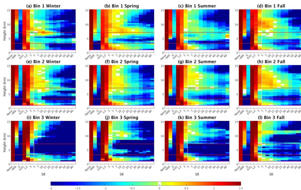
Figure 109: Lidar scattering ratio (SR(z)) histogram obtained by cumulating all lidar observations during daytime for bin 1 (a)–(d), bin 2 (e)–(h) and bin 3 (i)–(l) for winter (first column), spring (second column), summer (third column) and fall (fourth column). The color bar is the logarithm of the percentage of occurrence (the sum of one level is equal to \log_{10} 100\% ); lidar data showed in each subplot start above the instrument’s recovery altitude ( z = 1 km); the red horizontal lines represent the limits of low-, mid- and high-level clouds; and the white vertical line shows the threshold of clouds detection ( SR(z) = 5 ).
