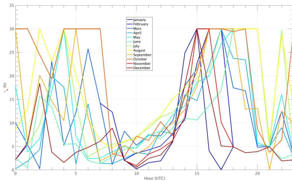
1090 Figure A3: Mean-hourly \tau_a value for each month of the year.
