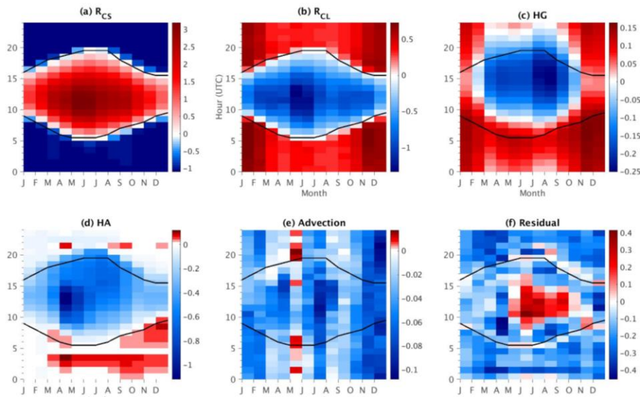
Figure 4: Monthly-hourly mean values for (a) R_{CS} , (b) R_{CL} , (c) HG , (d) HA , (e) Adv and (f) the residual (i.e. difference between the model and the observations). Units on the color bars are all in ^{\circ}\text{C h}^{-1} , and their scale is different for each subfigure. The black contour line on each figure corresponds to sunrise (bottom line) and sunset (top line) approximative hours.
