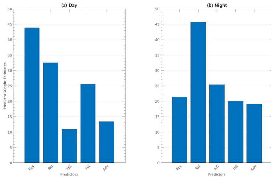
Figure 5: Predictor importance estimates obtained by the random forest method for (a) day and (b) night. The abscissa in both cases represents each predictor (or term) of the model, and the y-axis their importance (unitless) defined as the sum of their mean square error when permutation in the decision trees is done.
