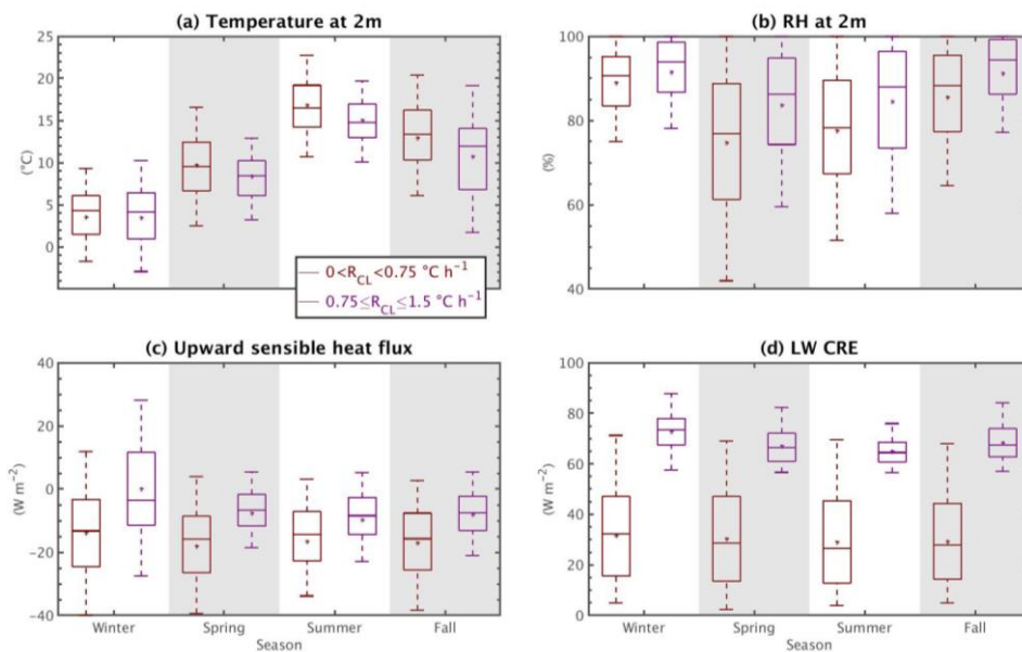
Figure 110: Nighttime values for (a) temperature, (b) relative humidity, (c) upward sensible heat flux at 2 m, and (d) longwave cloud radiative effect. Colors and boxplots follow the same definition as in Fig. 8b.
