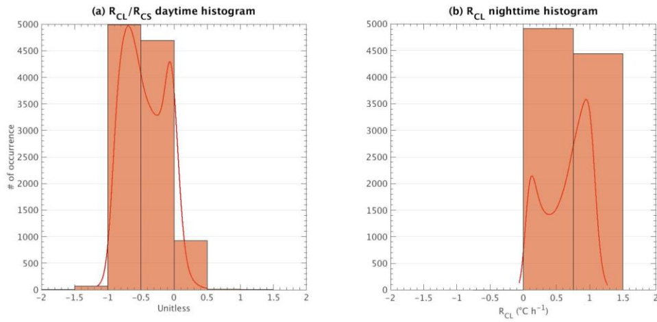
Figure C1: (a) Daytime histogram of \frac{R_{CL}}{R_{CS}} and (b) nighttime histogram of R_{CL} . The red line in both figures represents the PDF and the rectangular semi-transparent brown boxes the different bins created to analyze clouds influence. These histograms are built by considering only cloudy hours. Negative and close-to-zero values are removed for daytime hours (see text for further information).
