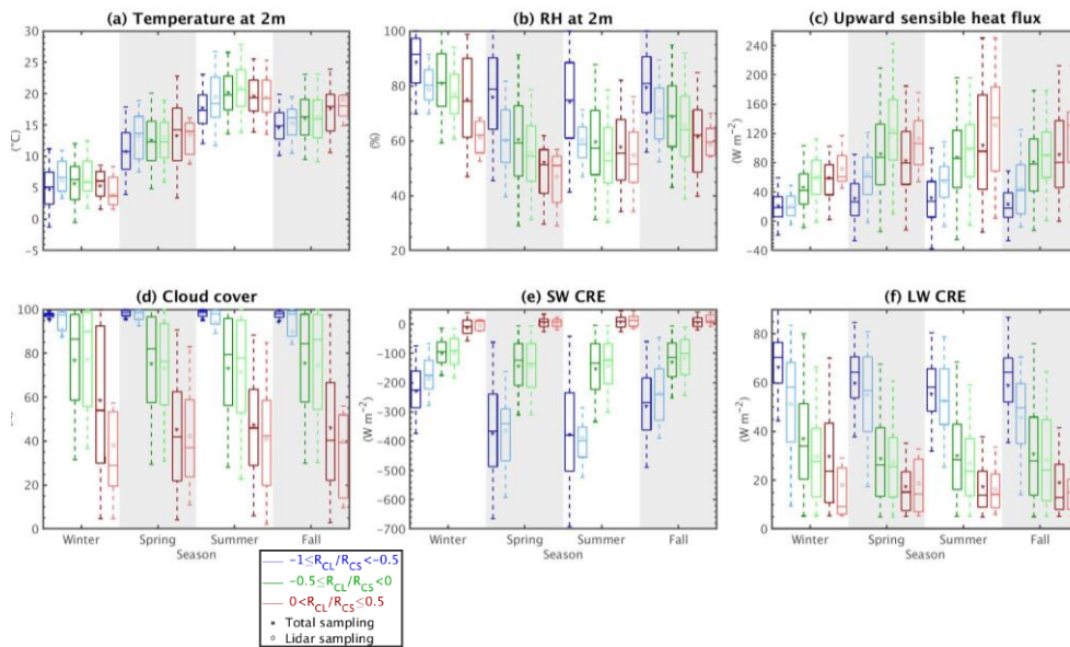
Figure 28: Daytime values for (a) temperature, (b) relative humidity, (c) upward sensible heat flux at 2m, (d) cloud cover retrieved from a sky imager, (e) shortwave and (f) longwave cloud radiative effect. Colors and boxplots follow the same definition as in Fig. 8a.
