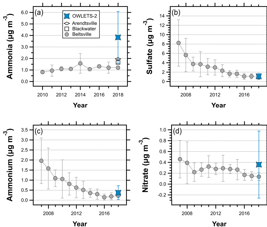
Figure 2. Summertime (June, July, and August) comparisons of a) \text{NH}_3 concentrations measured at HMI, Beltsville, Arendtsville , Arendtsville , and Blackwater; b) \text{PM}_{2.5} \text{SO}_4^{2-} measured at HMI and HUB; c) \text{PM}_{2.5} \text{NH}_4^+ measured at HMI and HUB; and d) \text{PM}_{2.5} \text{NO}_3^- measured at HMI and HUB. Error bars represent \pm the standard deviation.
