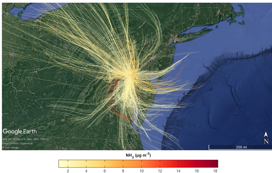
Figure 4. Aggregate 15-hour HYSPLIT back trajectories initialized at HMI (50 m altitude) and colored by \text{NH}_3 concentrations measured at HMI utilizing 12-km NAM meteorology to show regional trends 3 km HRRR meteorology. Every other back trajectory is displayed for clarity.
