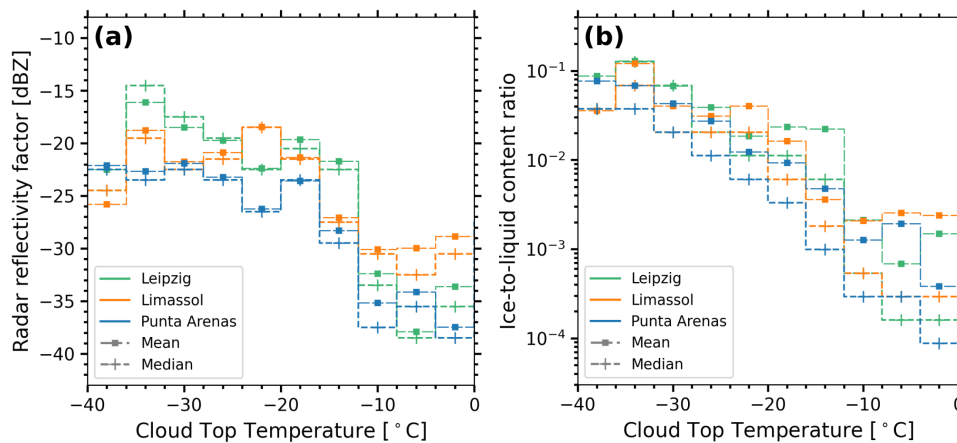
Figure 10. Radar Amount of ice observed in the virga, (a) radar reflectivity factor observed at the top of the virga (180m below the liquid-dominated layer base) (a) and ice-to-liquid-content-ratio (b) ice-to-liquid-content-ratio binned by CTT. Temperature bins of 4^{\circ}\text{C} .
