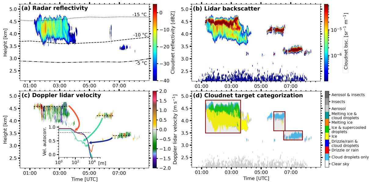
Figure 2. MIRA-35 Stratiform liquid-topped clouds as observed with LACROS. (a) Cloud radar reflectivity overlaid with the temperature, (ab) ;-PollyXT-Lidar attenuated backscatter, (bc) ;-Streamline-Doppler lidar vertical velocity(e), and (d) Cloudbnet target categorization (d) on the 28 November 2018 between -00:20 and to 09:00 UTC. The temperature information in (a) is obtained from ECMWF IFS model data. Red rectangles in (d) show indicate the automatically detected liquid-topped shallow stratiform clouds. The inset in (c) shows the autocorrelation function of the vertical velocities in the liquid-dominated layer (heights indicated by dashed lines)-of each cloud. The height of the velocity sampling is indicated with dashed lines. Further detailles details are provided in Sec. 2.5.
