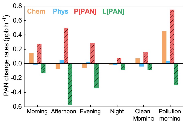
275 Figure 6. Process diagnostic analysis of PAN on average and on the mornings of clean and pollution days. Chem, Phys, P[PAN], and L[PAN] denote the net chemical production, physical changes, chemical production and loss rates of PAN, respectively. Morning, afternoon, evening and night correspond to 8:00–12:00, 12:00–16:00, 16:00–20:00 and 20:00–08:00, respectively.
