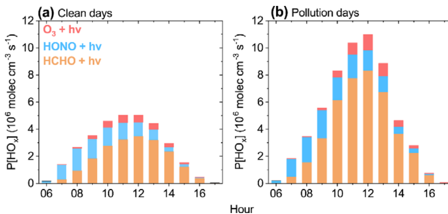
365 Figure 10. Diurnal variations of P[HO x ] through three pathways during the daytime of clean days (a, 10/13–10/19, 10/21–10/24) and pollution days (b, 10/22, 10/25 and 10/26) at the SDZ site.
