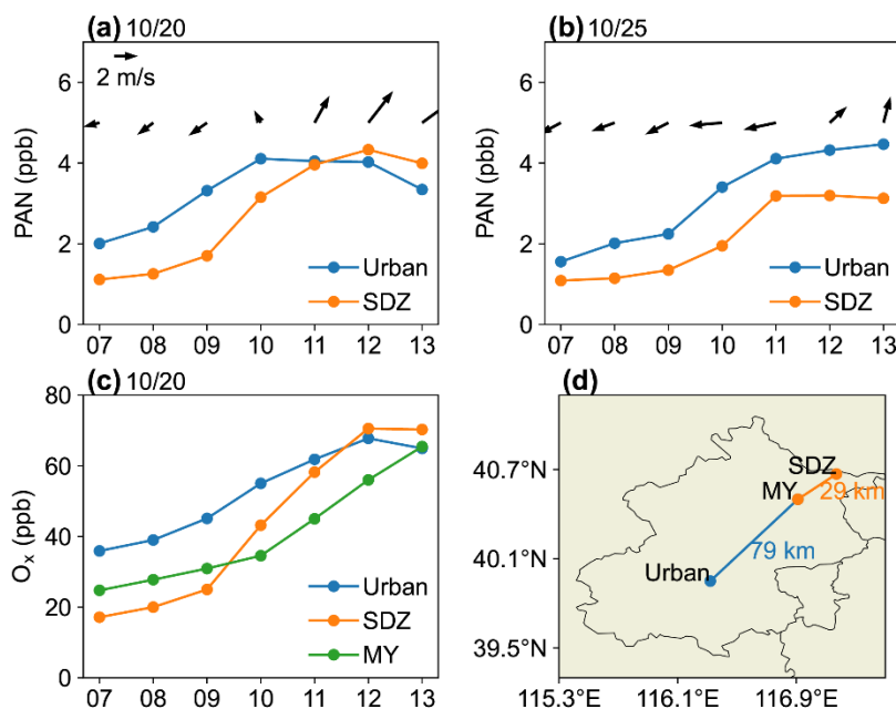
250 Figure 5. Hourly variations of PAN concentrations (ppb) and surface wind at the urban and SDZ site during 7:00–13:00 on (a) 10/20 and (b) 10/25. (c) Hourly variation of O_x concentrations (ppb) at the urban, SDZ and MY site during 7:00–13:00 on 10/20. (d) Detailed locations of the urban, SDZ and MY site and the distances between them.
