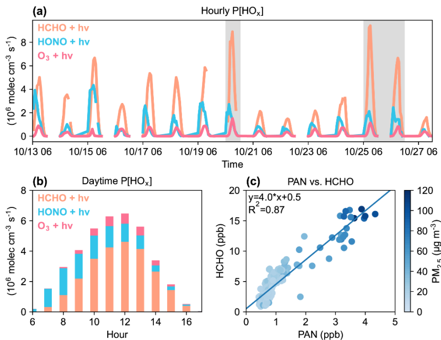
340 Figure 9. (a) Hourly time series of calculated HO x production rates (P[HO x ]) through photolysis of O 3 , HONO and HCHO during 06:00–17:00 from 10/13 to 10/27 at the SDZ site. (b) Daytime P[HO x ] through each pathway averaged during 10/13 to 10/27. (c) Daytime PAN concentrations versus HCHO concentrations from 10/13 to 10/27 at the SDZ site. The colors denote the corresponding PM 2.5 levels.
