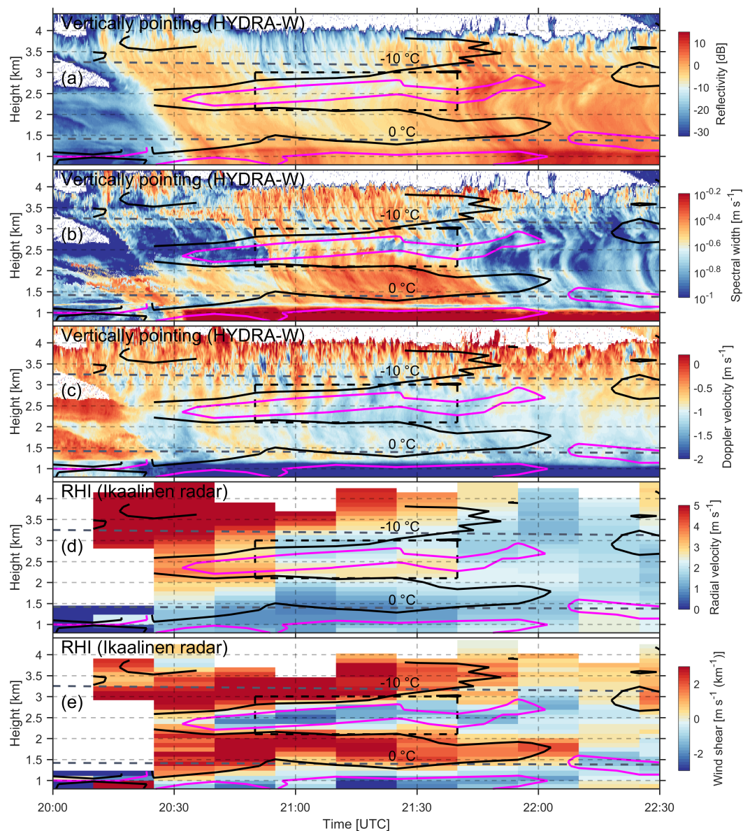
Figure 1. Radar observations collected on 18 April 2018 between 20:00 and 22:30 UTC showing: HYDRA-W reflectivity (a), spectral width (b) and mean Doppler velocity (c). Panels (d) and (e) present vertical profiles of radial Doppler velocity and vertical wind shear derived from the RHI scans of Ikaalinen radar (IKA). Purple and black contours depict the wind shear of -1 and 1 \text{ m s}^{-1}(\text{km}^{-1}) , respectively. The 0^\circ\text{C} and -10^\circ\text{C} isotherms are marked by gray dashed lines. The black dashed line box shows the region where the spectral analysis has identified presence of supercooled liquid, as shown in Fig. 4.
