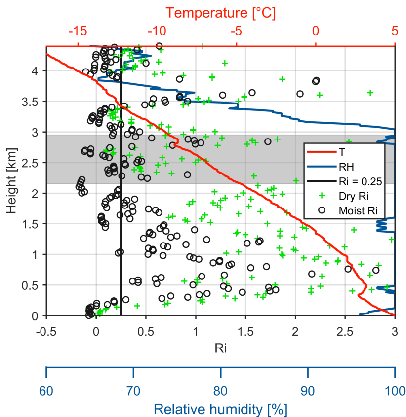
Figure 2. Radiosonde observations at 23:30 UTC on 18 April 2018 from the Jokioinen station. This panel shows the air temperature (T, red line), relative humidity (RH, blue line), dry (green cross) and moist (black circle) Ri numbers derived from the radiosonde data. The vertical black line indicates critical Richardson number Ri = 0.25 ; The gray shading area in this figure corresponds to the heights as marked by black dashed line box in Fig. 1.
