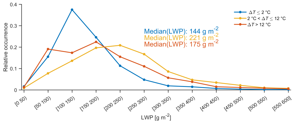
Figure 11. Relative occurrence of LWP for all columnar-ice-producing events.
