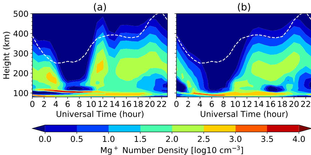
Figure 8. Mg + density over (12°N, 0°, near the dip equator) as a function of universal time and altitude at June Solstice. The dashed lines denote hmF2. (a) for the TA simulation and (b) for the CE simulation.
