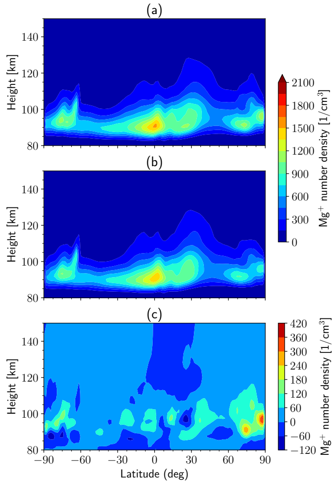
Figure 7. The monthly and zonal mean of the Mg + number density in June from (a) the TA simulation and (b) the CE simulation. (c) The difference between the TA and CE simulations.
