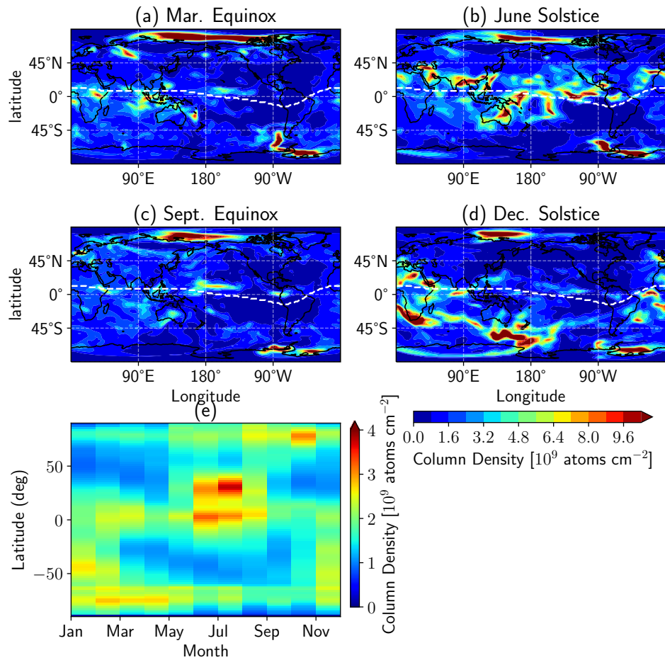
Figure 3. (a-d) Global geographical distribution of the \text{Mg}^+ column density during the equinoxes and solstices, at 00 UTC. (e) Seasonal variation of the zonal mean \text{Mg}^+ column density as a function of month and latitude. The white dashed lines indicates the position of the the dip equator.
