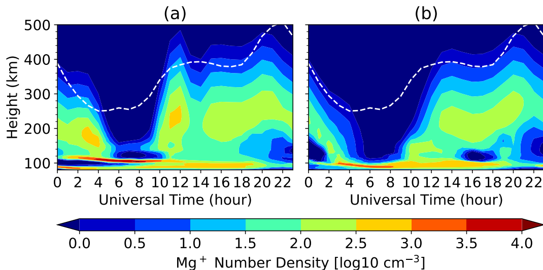
Figure 8. \text{Mg}^+ density over ( 12^\circ\text{N} , 0^\circ , near the dip equator) as a function of local -universal time and altitude at June Solstice. The dashed lines denote hmF2. (a) for the TA simulation and (b) for the CE simulation.
