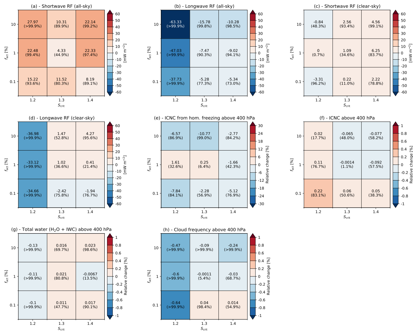
Figure 5. As in Fig. 4, but for (a) all-sky shortwave; (b) all-sky longwave; (c) clear-sky shortwave; and (d) clear-sky longwave top-of-the atmosphere RFs. Panels (e-h) depict the aviation-soot-induced relative changes in ICNC from homogeneous freezing, ICNC, total water (as the sum of water vapour and ice water), and cloud frequency, respectively, all spatially averaged above 400 hPa and over cloudy and cloud-free model grid-boxes.
