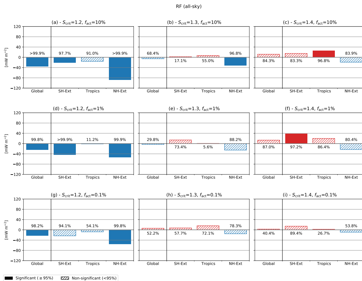
Figure 6. As in Fig. 4, but averaged over different regions. Each of the panels (a-i) corresponds to a given assumption for ice nucleation efficiency of aviation soot particles ( S_{crit} and f_{act} ) as shown on the top. The values above or below each bar indicate the confidence level. Significant and non-significant results are further marked using filled and hatched bars, respectively. To facilitate the comparison, the bar in the left box in each panel shows the global RF values as in Fig. 4.
