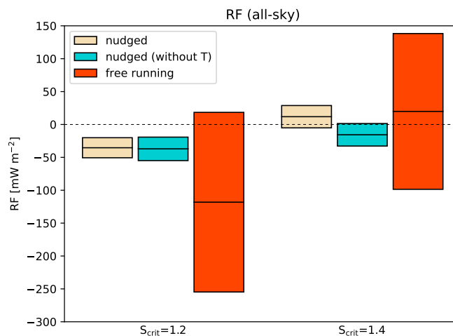
Figure 8. Multi-year average top-of-the-atmosphere all-sky RF due to the effect of aviation soot on natural cirrus clouds, under different model configurations: nudged, nudged without relating temperature, and free running. The latter configuration covers a period of 30 years, while the nudged ones cover 15 years. The horizontal line at the center of each box is the average value and each box spans the 95% confidence interval. Values are shown for S_{crit} = 1.2 and S_{crit} = 1.4 , in both cases assuming f_{act} = 10\% . Note that for the free running experiments, the confidence levels are calculated using a Welch's t-test instead of a paired-sample t-test as in the nudged ones.
