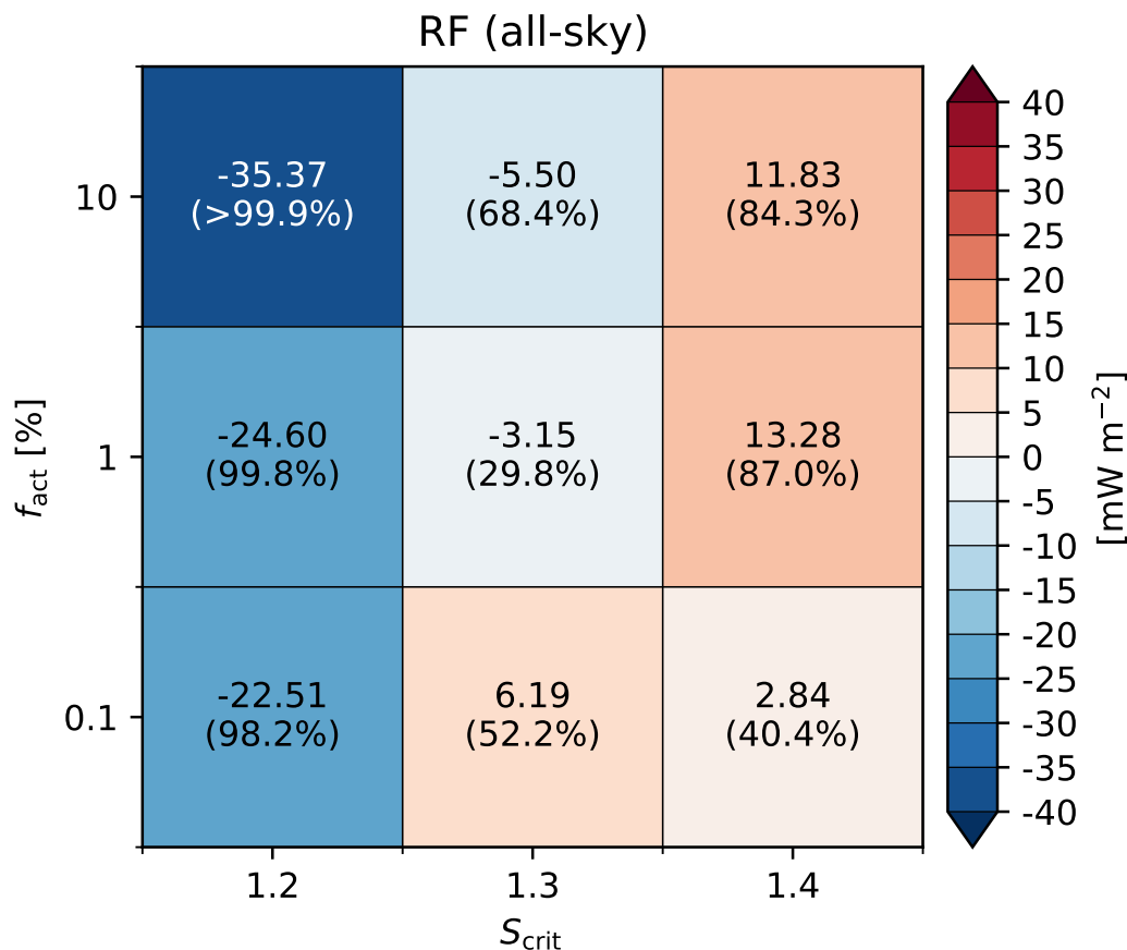
Figure 4. Multi-year average (2001–2015) top-of-the-atmosphere all-sky RF due to the effect of aviation soot on natural cirrus clouds, under different assumptions for the ice nucleation efficiency of aviation soot INPs ( S_{crit} and f_{act} ). The values in brackets within each box indicate the confidence level.
