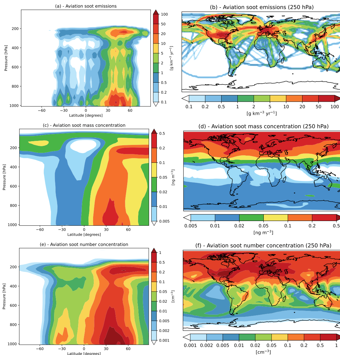
Figure 3. Zonally averaged (a) and geographical distribution at 250 hPa (b) of aviation soot emissions from the CMIP6 dataset used for the model simulations in this work. The other panels show the mass concentration (c,d) and the number concentration (e,f) of aviation soot simulated by EMAC-MADE3 (BASE experiment, see Table 1). Panels (a), (c) and (e) show zonal means, whereas (b), (d) and (f) show the \sim 250 hPa level. All panels consider the multi-year average over the simulated period (2001–2015). Note that the number concentration of aviation soot is further multiplied by the active fraction f_{act} = 0.1 - 10\% in the cirrus parametrization to obtain the number concentration of aviation soot INPs.
