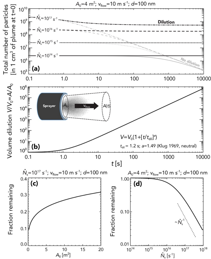
1330 Figure 11: Effects of coagulation on the concentration of particles at time t downstream of a hypothetical sprayer system with cross sectional area A=4 \text{ m}^2 and flow rate of air across the sprayer v_{\text{flow}}=10 \text{ m s}^{-1} . Here, a single particle diameter d=100 \text{ nm} is assumed, and solutions follow Turco and Yu (1997). (a) Particle concentrations with dilution proceeding according to the dispersion rates for neutral conditions from Klug (1969), as reproduced in Seinfeld and Pandis (2006, Table 18.3); concentrations in the absence of plume dilution are shown for comparison (gray) indicating major losses and eventual asymptotic solution; (b) the ratio of volume V to initial volume V_0 increases super-linearly with time with dilution timescale t_{\text{dil}}=1.2 \text{ s} ; (c) fraction of particles remaining at t=10,000 \text{ s} 1335 as a function of initial plume cross sectional area A_0 for spray rate \dot{N}_s=10^{17} \text{ s}^{-1} ; (d) fraction of particles remaining at t=10,000 \text{ s} as a function of \dot{N}_s for A_0=4 \text{ m}^2 . The dotted line shows the scaling such that the fraction remaining decreases at the same rate as \dot{N}_s increases, i.e., there is no increase in far-field particle concentration with increasing sprayer output.
