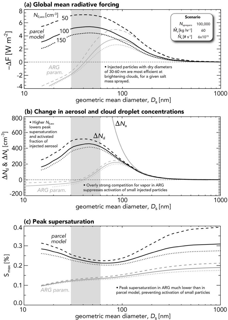
Figure 7: (a) Global mean radiative forcing -\Delta F for a fixed salt mass spray rate (based on Scenario 2, see legend) as a function of injected particle geometric mean diameter D_s for three unperturbed accumulation mode aerosol concentrations N_{0,\text{acc}}=50, 100 and 150 \text{ cm}^{-3} . Black curves show the results from the parcel model and gray curves from the ARG parameterization; (b) Change in mean cloud droplet concentration \Delta N_d and aerosol concentration \Delta N_a in regions where sprayers are operating; (c) Peak supersaturation in the updraft. The gray shaded box indicates the most effective range of D_s .
