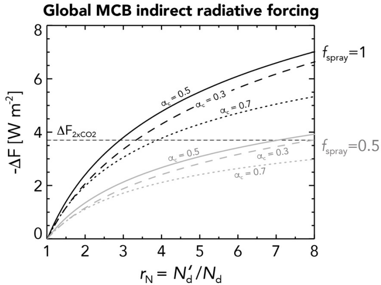
1215 Figure 1: Global radiative forcing from marine cloud brightening \Delta F as a function of the ratio of the perturbed to unperturbed (background) cloud droplet concentration r_N = N'_d/N_d . Curves are shown for the case where sprayers are deployed over all eligible ocean regions ( f_{\text{spray}} = 1 , black lines) and where sprayers are deployed over only 50% of these areas ( f_{\text{spray}} = 0.5 , gray lines), for unperturbed cloud albedos \alpha_c ranging from 0.3-0.7. The fraction of the Earth's surface area eligible for seeding is f_{\text{ocean}} = 0.54 , and the atmospheric correction factor \phi_{\text{atm}} = 0.7
