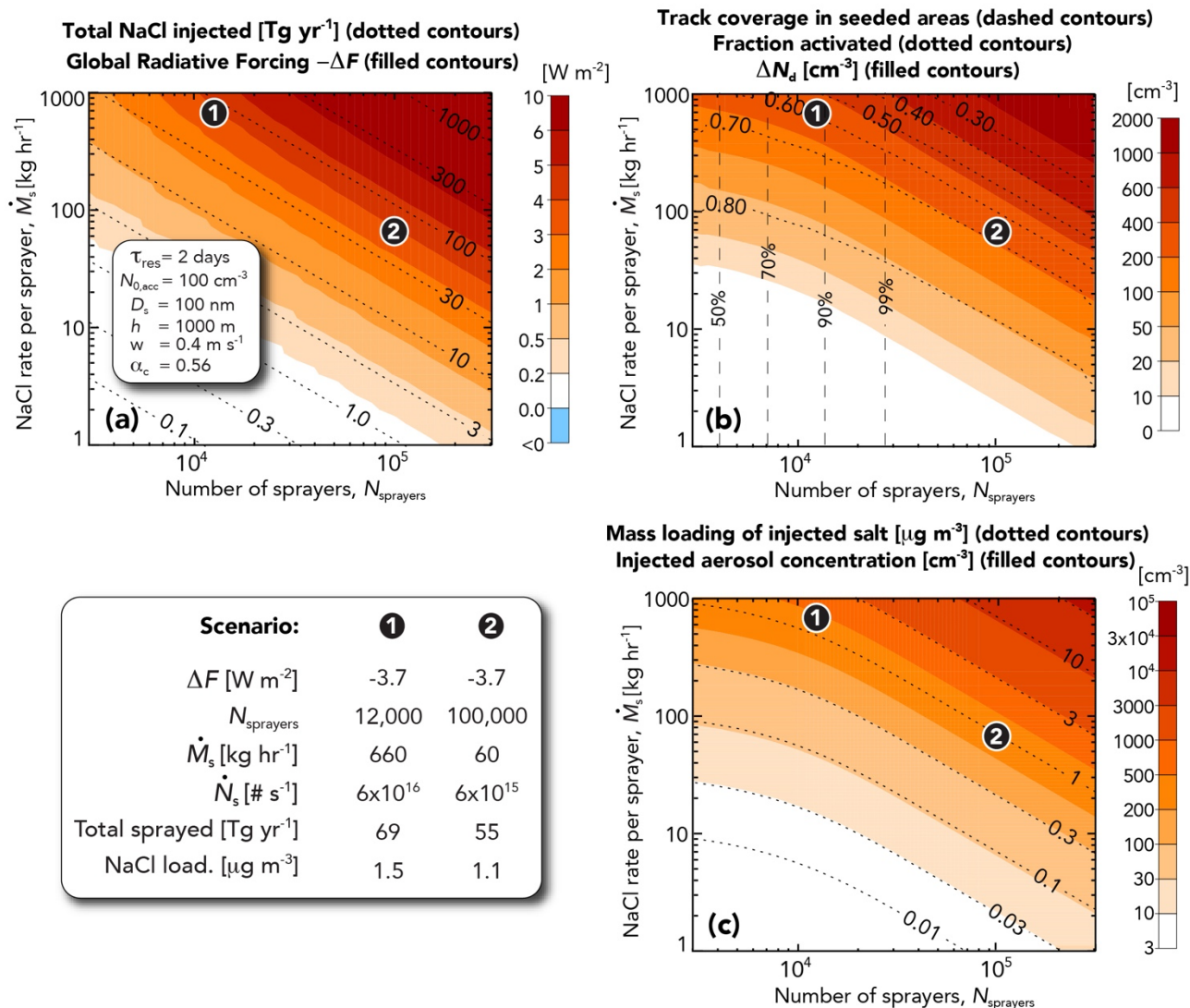
Figure 5: (a) Global mean radiative forcing \Delta F (colors) and total flux of sodium chloride (dotted contours) from MCB applied to all eligible ocean areas (54% of Earth's surface) as a function of the number of sprayers N_{\text{sprayers}} and the salt mass injection rate \dot{M}_s for each sprayer; (b) increase in cloud droplet concentration \Delta N_d (colors), mean fraction of aerosol activated in tracks (dotted contours), and track coverage (dashed contours); (c) injected aerosol number concentration in tracks (colors) and mean mass loading in the MBL of injected salt (dotted contours). The inset of panel (a) shows the key model parameters, with others as in Table 1. Two scenarios (1) and (2), which each produce sufficient forcing to offset doubled CO 2 are highlighted. Scenario (2) has a higher number of sprayers but a lower rate of particles injected per sprayer.
