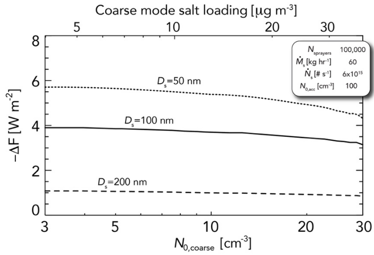
Figure 8: Global mean radiative forcing -\Delta F for a fixed salt mass spray rate (based on Scenario 2, see legend) as a function of background coarse mode aerosol concentration N_{0,coarse} for three injected particle sizes D_s=50, 100 and 200 nm. The equivalent salt mass loading in the coarse mode is indicated by the top axis.
