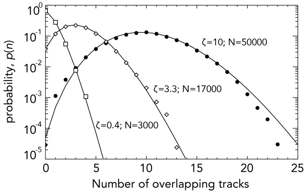
1230 Figure 3: Probability density functions p(n) derived from the Monte Carlo simulations of overlapping rectangular tracks for three values of the mean track density \zeta (0.4, 3.3 and 10). For the simulations, a domain of size 4000×4000 km is modelled using a 4000×4000 array, and tracks of length 1200 km and width 44 km (see Sect. 2.5) are placed randomly to the array, assuming periodic 1235 boundary conditions. The long dimension of each track is randomly set to be parallel to the i or j direction of the box. Poisson distributions (Equation 8) are shown corresponding based on the mean track densities and represent an excellent fit to the data. The track densities \zeta = 0.4, 3.3 and 10 correspond to a total number of ships, if spraying were to take place over the entire eligible ocean region, of \sim 3000, \sim 17000 , and \sim 50000 respectively.
