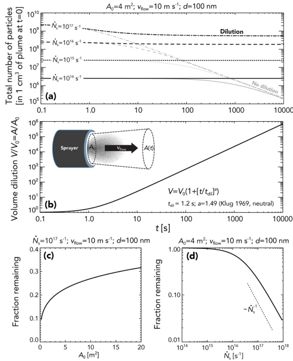
Figure 11: Effects of coagulation on the concentration of particles at time t downstream of a hypothetical sprayer system with cross sectional area A=4 \text{ m}^2 and flow rate of air across the sprayer v_{\text{flow}}=10 \text{ m s}^{-1} . Here, a single particle diameter d=100 \text{ nm} is assumed, and solutions follow Turco and Yu (1997). (a) Particle concentrations with dilution proceeding according to the dispersion rates for neutral conditions from Klug (1969), as reproduced in Seinfeld and Pandis (2006, Table 18.3); concentrations in the absence of plume dilution are shown for comparison (gray) indicating major losses and eventual asymptotic solution; (b) the ratio of volume V to initial volume V_0 increases super-linearly with time with dilution timescale t_{\text{dil}}=1.2 \text{ s} ; (c) fraction of particles remaining at t=10,000 \text{ s} as a function of initial plume cross sectional area A_0 for spray rate N_s=10^{17} \text{ s}^{-1} ; (d) fraction of particles remaining at t=10,000 \text{ s} as a function of N_s for A_0=4 \text{ m}^2 . The dotted line shows the scaling such that the fraction remaining decreases at the same rate as N_s increases, i.e., there is no increase in far-field particle concentration with increasing sprayer output.
