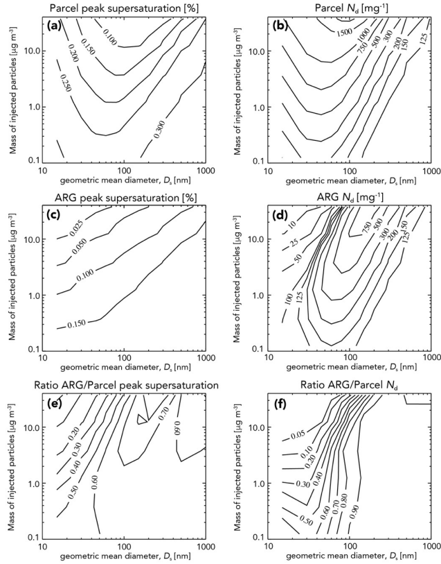
Figure A1: Comparison of the parcel model and ARG peak supersaturations (panels a, c, e) and activated cloud droplet concentrations N_d (panels b, d, f) as a function of the injected particle geometric mean diameter D_g and the mass loading of injected particles. The other parameters are set as w=0.4 \text{ m s}^{-1} , N_{0,\text{acc}}=100 \text{ mg}^{-1} , N_{0,\text{coarse}}=10 \text{ mg}^{-1} (base values used throughout the paper). The top row shows results from the parcel model, the center from ARG, and the bottom row is the ratio of ARG to the Parcel model.
