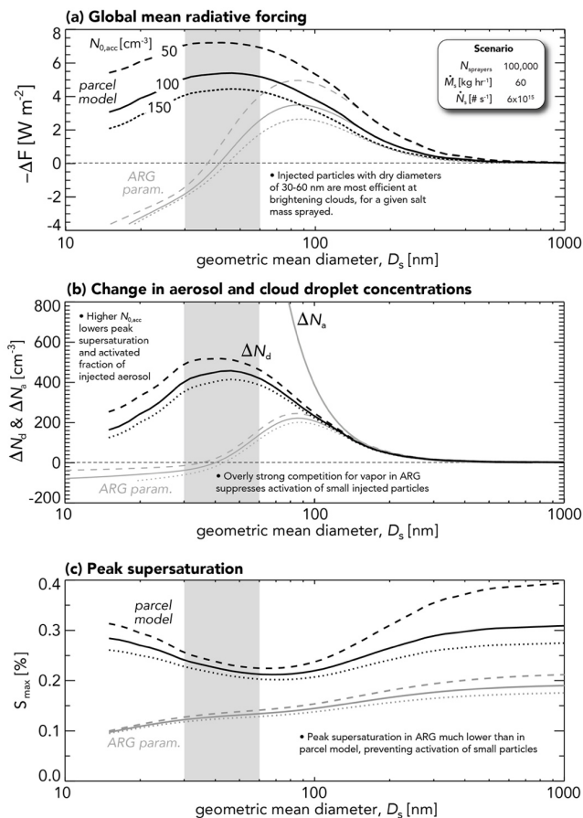
1380 Figure 7: (a) Global mean radiative forcing -\Delta F for a fixed salt mass spray rate (based on Scenario 2, see legend) as a function of injected particle geometric mean diameter D_s for three unperturbed accumulation mode aerosol concentrations N_{0,acc}=50, 100 and 150 \text{ cm}^{-3} . Black curves show the results from the parcel model and gray curves from the ARG parameterization; (b) Change in mean cloud droplet concentration \Delta N_d and aerosol concentration \Delta N_a in regions where sprayers are operating; (c) Peak supersaturation in the updraft. The gray shaded box indicates the most effective range of D_s .
