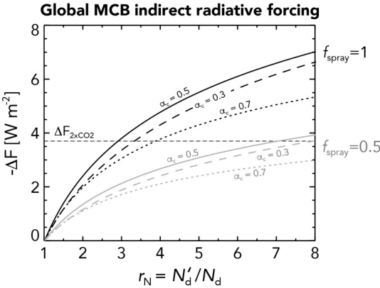
Figure 1: Global radiative forcing from marine cloud brightening \Delta F as a function of the ratio of the perturbed to unperturbed (background) cloud droplet concentration r_N = N'_d/N_d . Curves are shown for the case where sprayers are deployed over all eligible ocean regions ( f_{\text{spray}} = 1 , black lines) and where sprayers are deployed over only 50% of these areas ( f_{\text{spray}} = 0.5 , gray lines), for unperturbed cloud albedos \alpha_c ranging from 0.3–0.7. The fraction of the Earth’s surface area eligible for seeding is f_{\text{ocean}} = 0.54 , and the atmospheric correction factor \phi_{\text{atm}} = 0.7 .
