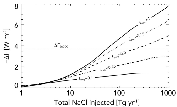
1435 Figure 12: Sensitivity of the radiative forcing to different fractions f_{\text{spray}} of the eligible ocean where sprayers operate. Forcing is shown as a function of the total (global) rate of salt mass injection. The mass injected per sprayer is the same as that for scenario 2 (Sect. 4.1 and Fig. 5) and the sprayer density is the same in each case, i.e., the number of sprayers is proportional to f_{\text{spray}} and is 100,000 for f_{\text{spray}}=1 . The geometric mean spray diameters D_s=100 nm and the background N_{0,\text{acc}}=100 cm -3 . All other parameters are the same as those used in Fig. 5.
