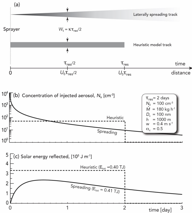
Figure 2: (a) Plan view of a realistic laterally-spreading plume/track (top) and the track assumed in the heuristic model, as a function of time/distance downstream of the sprayer. The shading qualitatively indicates the injected particle concentration. (b) Injected aerosol concentration as a function of time for the two plume types given the spray injection information in the box. A residence time \tau_{res} = 2 days, and a widening rate K = 1.85 km hr -1 are assumed, and the model is run out to 10 days to capture the total reflected solar radiation for the spreading plume. (c) additional reflected solar radiation per meter length of track from aerosol-cloud interactions for the two plume types. The total additional reflected energy E_{tot} from the two plumes is very similar. In this case, approximately 43% of the energy reflected from the spreading plume occurs for times t > \tau_{res} .
