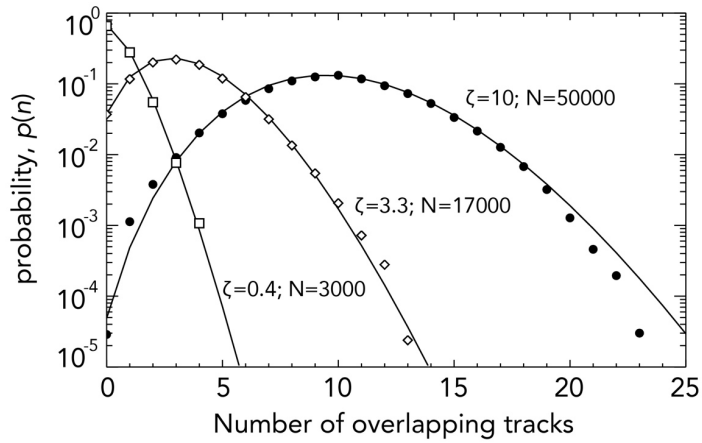
Figure 3: Probability density functions p(n) derived from the Monte Carlo simulations of overlapping rectangular tracks for three values of the mean track density \zeta (0.4, 3.3 and 10). For the simulations, a domain of size 4000×4000 km is modelled using a 4000×4000 array, and tracks of length 1200 km and width 44 km (see Sect. 2.5) are placed randomly to the array, assuming periodic boundary conditions. The long dimension of each track is randomly set to be parallel to the i or j direction of the box. Poisson distributions (Equation 8) are shown corresponding based on the mean track densities and represent an excellent fit to the data. The track densities \zeta = 0.4, 3.3 and 10 correspond to a total number of ships, if spraying were to take place over the entire eligible ocean region, of ~3000, ~17000, and ~50000 respectively.
