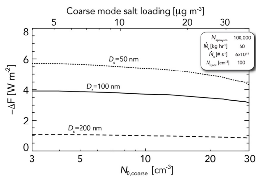
1385 Figure 8: Global mean radiative forcing -\Delta F for a fixed salt mass spray rate (based on Scenario 2, see legend) as a function of background coarse mode aerosol concentration N_{0,coarse} for three injected particle sizes D_s=50, 100 and 200 nm. The equivalent salt mass loading in the coarse mode is indicated by the top axis.
