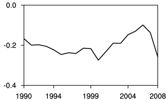
Figure R1. The 21-year sliding correlation coefficients between Nino3.4 index and OWI.
