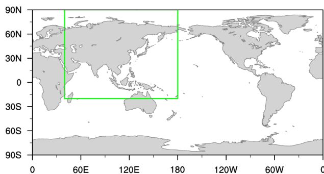
Figure R4. The scope of fixed anthropogenic emissions (green box).
