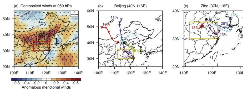
Figure R3. Winds that transport O 3 from central eastern China to North China during OPEs5. (a) Composites of anomalous wind fields at 950 hPa during OPEs5 in North China relative to the seasonal-mean over May-July in 2014-2018. The daily time series of wind in each grid is standardized by the standard deviation. Shades indicate anomalous meridional wind speeds during OPEs5 relative to seasonal-mean. Blue dots indicate grids with statistically significant differences in meridional wind speed at 99% confidence level. The North China and central eastern China are enclosed by green and red rectangles, respectively. (b)-(c) Five-day backward trajectories of the air mass at two cities (Beijing and Zibo) in North China for days of OPEs5 over May-July in 2014-2018. The trajectories are retrieved at 2:00, 8:00, 14:00 and 20:00 GMT +8 for each day during the OPEs5. Inverted triangles appear every 24 h on each trajectory. The percentages with different colors indicate the frequencies of different trajectories. The yellow rectangle encloses central eastern China.
