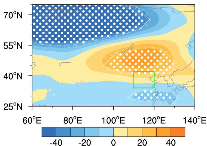
Figure R5. Composite difference of the geopotential height at 500 hPa (unit: gpm) in summer between the six highest and the six lowest EU index years from 1980 to 2018. The white dots (hatching) indicate that the difference was above the 95% (90%) confidence level (t test). The green box represents the location of North China.
