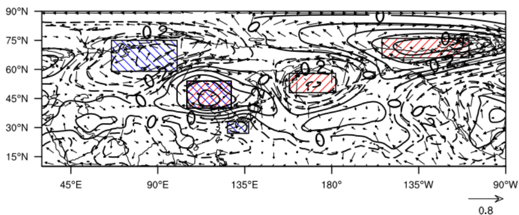
Figure R2. Correlation coefficients between the May Sea ice index and JJA mean geopotential height at 500 hPa (contour) and JJA mean wind at 200 hPa (arrow) from 1979 to 2017. Regions of red (blue) oblique lines mean the centres of the TP_{WP} ( TP_{EU} ), which were used to calculate the Rossby wave index. The linear trend was moved. The atmospheric data used were ERA-interim data sets.
