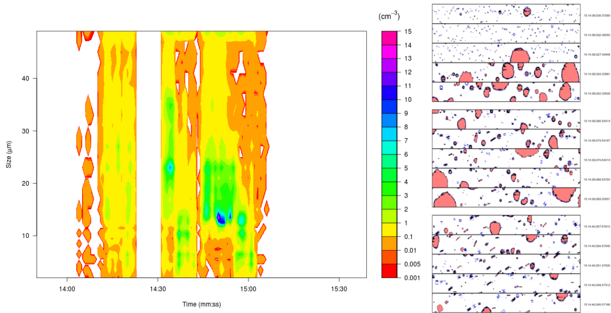
Figure 14. (left): Size distribution of drops measured with the Cloud Drop Probe, and (right) examples of images measured with the Cloud Imaging Probe (CIP) during Run 6. The CIP image width is 960 \mu\text{m} .
