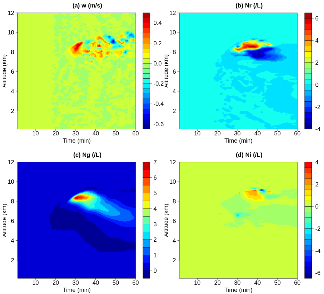
835 Figure 10. Difference between the Paukert run and the control run: (a) vertical velocity ( \text{m s}^{-1} ), (b) raindrop number concentration (per litre), (c) the graupel concentrations (per litre), and (d) the ice crystal concentrations (per litre), respectively.
