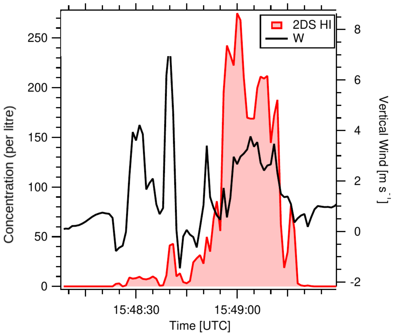
Figure 3. Time series of the concentration of ice particles ( L^{-1} ) in the size range of 50 -1280 \mu\text{m} measured with 2D-S Stereo Probe and vertical velocity ( \text{ms}^{-1} ) between 15:48:05 UTC and 15:49:30 UTC on 21 August 2015.
