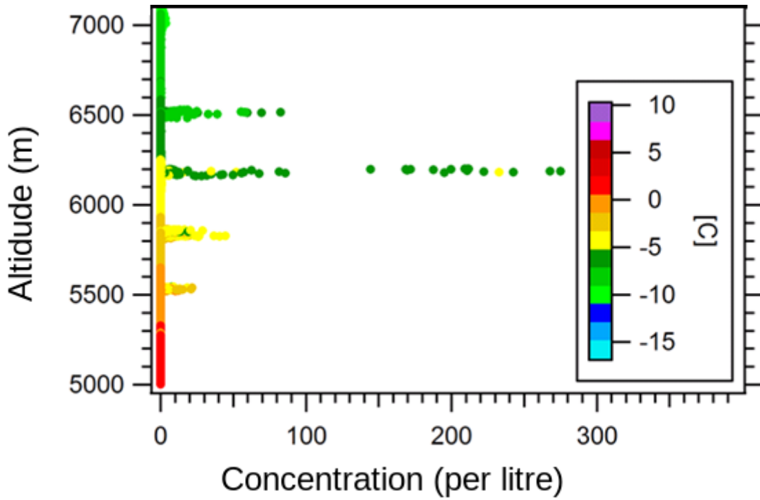
725 Figure 2. Ice concentration as a function of altitude as measured with the 2DS probe on board the Bae 146 aircraft. The colour bar represents temperature.
