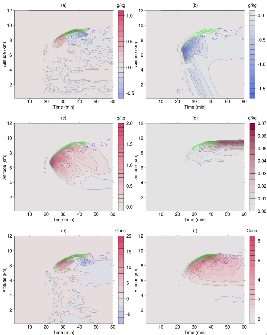
790 Figure 8. Difference between the sensitivity runearly onset1 & Cooper10x, and the control run, control: (a) cloud water mixing ratio ( \text{gkg}^{-1} ), (b) rain water mixing ratio ( \text{gkg}^{-1} ), (c) graupel mixing ratio ( \text{gkg}^{-1} ), (d) ice mixing ratio ( \text{gkg}^{-1} ), (e) raindrop concentration (per litre), and (f) graupel concentration (per litre), respectively. Imposed on these figures are the differences in vertical velocity, with green contour lines indicating positive and blue contour lines negative differences, and contour intervals of 0.5 \text{ ms}^{-1} .
