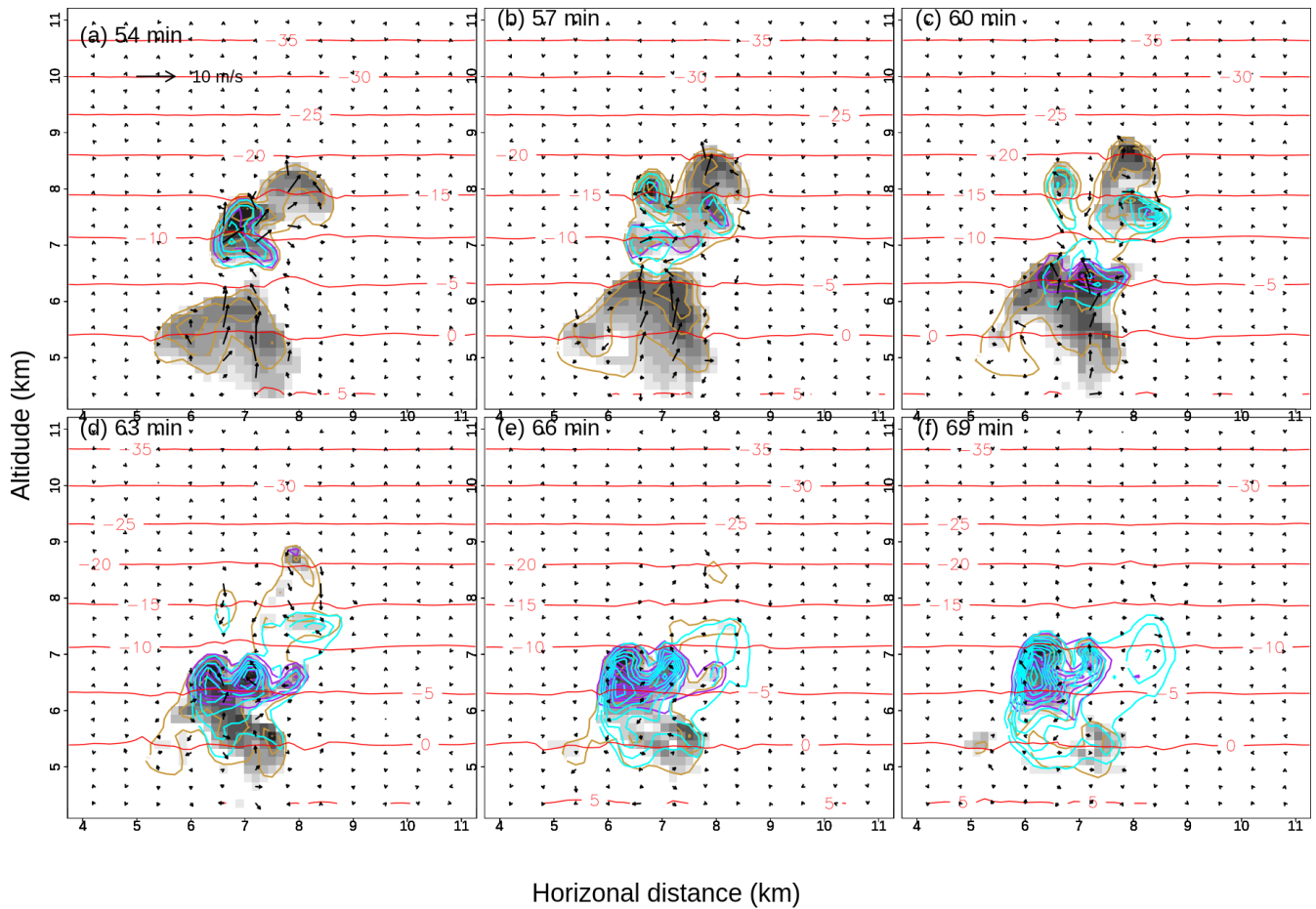
845 Figure 12. Time sequence for the multi-thermals run of spatial distribution of wind vectors, concentration of raindrops, ice crystals, and graupel particles at (a) 54 min, (b) 57 min, (c) 60 min, (d) 63 min, (e) 66 min and (f) 69 min. The orange, purple and cyan lines are the concentration of raindrops (intervals at 2L^{-1} ), ice crystals (intervals at 10L^{-1} ), and graupel particles (intervals at 2L^{-1} ), respectively. Cloud drop mass mixing ratio is shown in shade in each panel. The cyan lines are isotherms in ^{\circ}C . The maximum concentrations are shown in each panel in L^{-1} . The scale for the wind vectors is also shown in (a).
