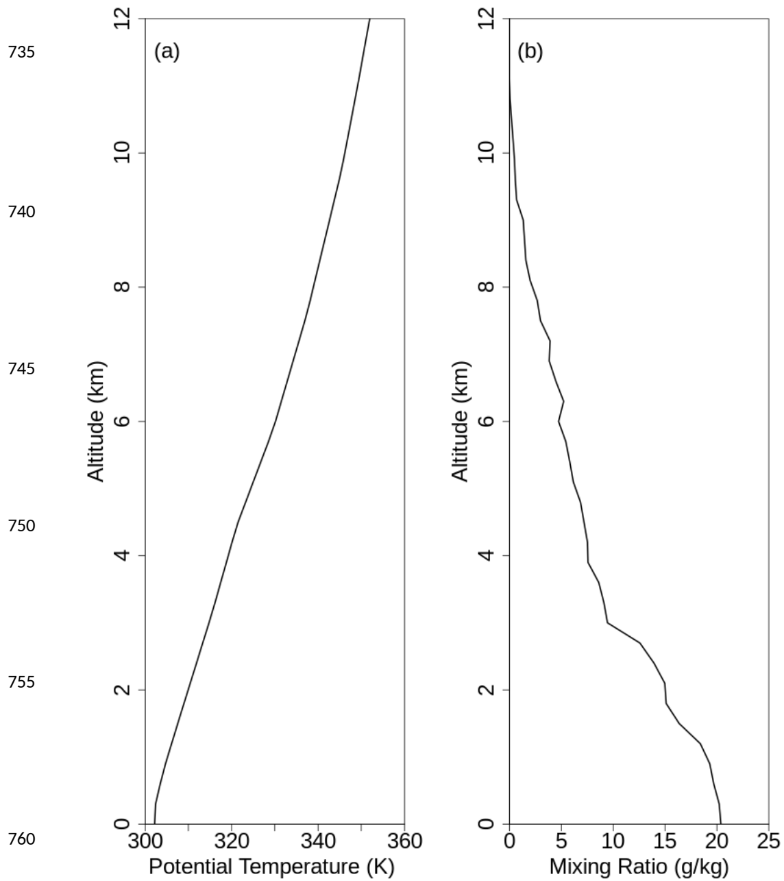
Figure 4. Initial profiles of (a) potential temperature and (b) mixing ratio for the model simulations. Altitude is the height above mean sea level.
